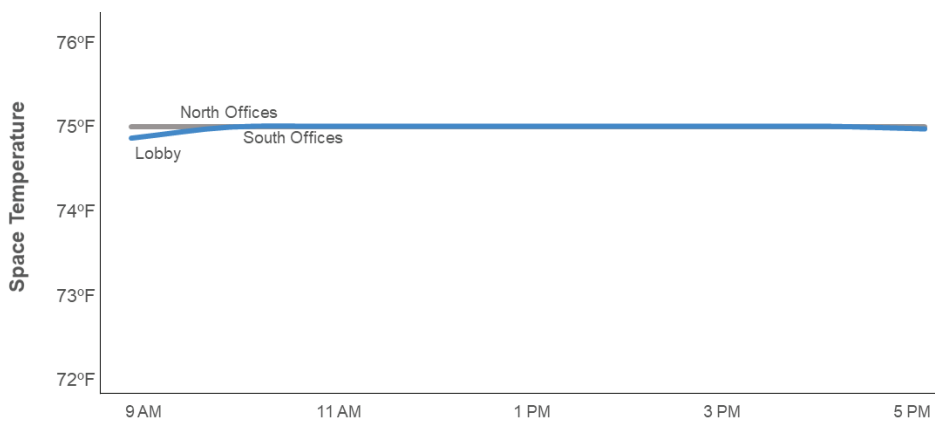
Temperature Control in Multiple-Zone VAV System (Minneapolis, July)
