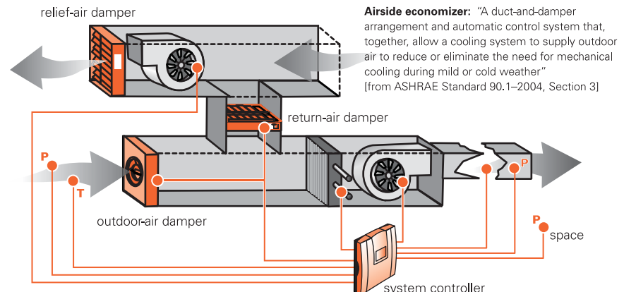
Figure 1. Typical air handler
