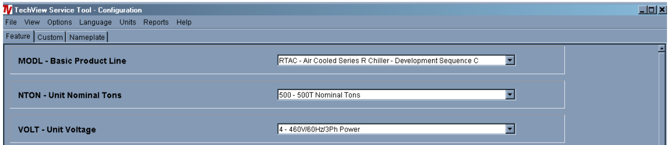
Figure 8. Software view
