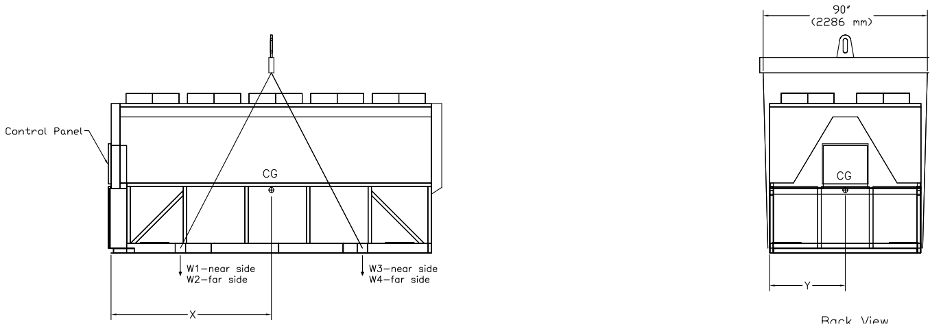
Figure 11. Lifting the unit (packaged and remote) — 30 to 36 foot base
