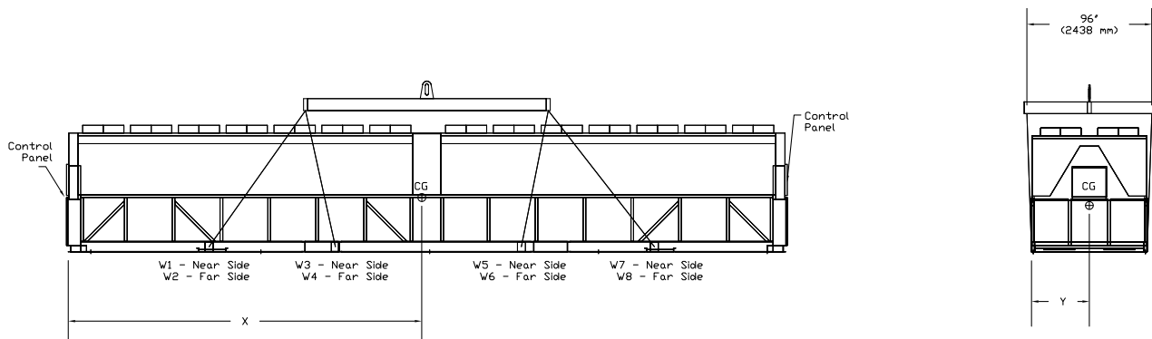
Figure 12. Lifting the unit (packaged and remote) — 39 to 45 foot base
