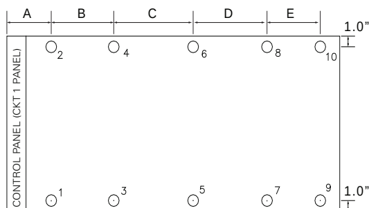
Figure 19. Mounting locations (without seismic rating)
