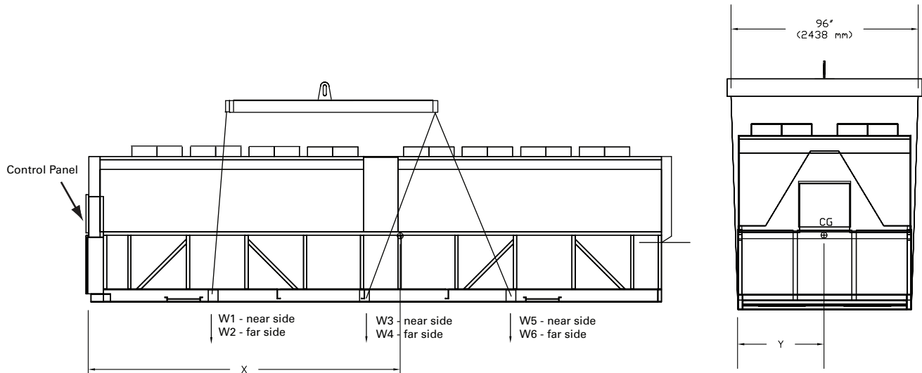
Figure 12. Lifting the unit (packaged and remote) — 39 to 45 foot base
