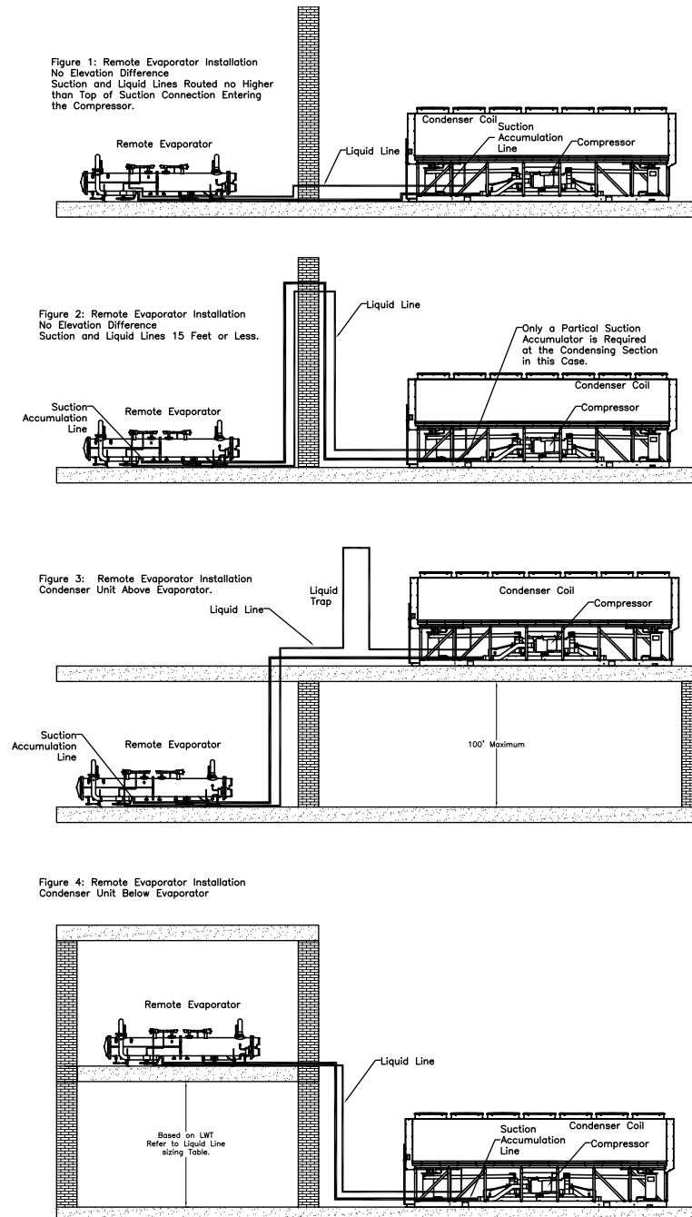
Figure 29. Remote evaporator installations
