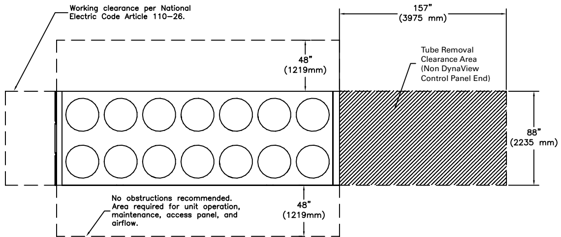
Figure 7. Recommended unit clearances — 30 to 45 foot bases
