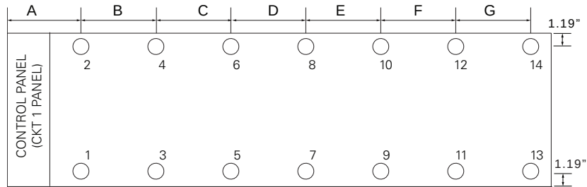
Figure 20. Mounting locations — seismic spring isolators or seismic elastomeric pads
