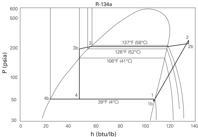
Figure 37. Pressure enthalpy (P-h) diagram - RTAC
