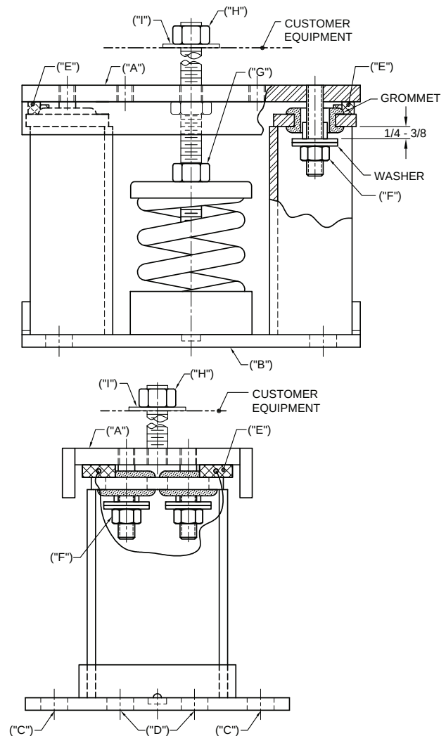
Figure 18. MSSH seismic isolator installation reference
