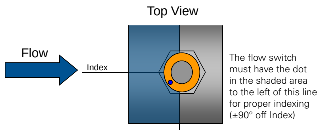
Figure 23. Proper flow switch indexing
