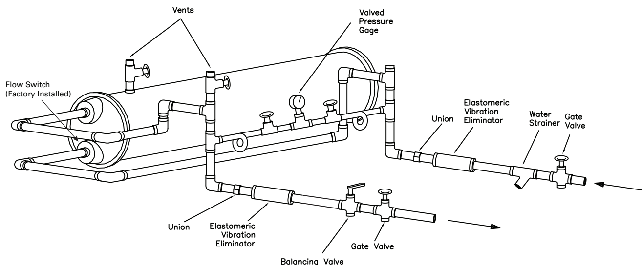
Figure 28. Suggested piping for typical RTAC evaporator
