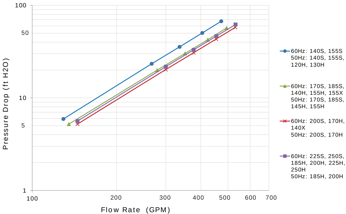
Figure 26. Evaporator water pressure drop, 3-pass evaporator, 120 to 250 tons
