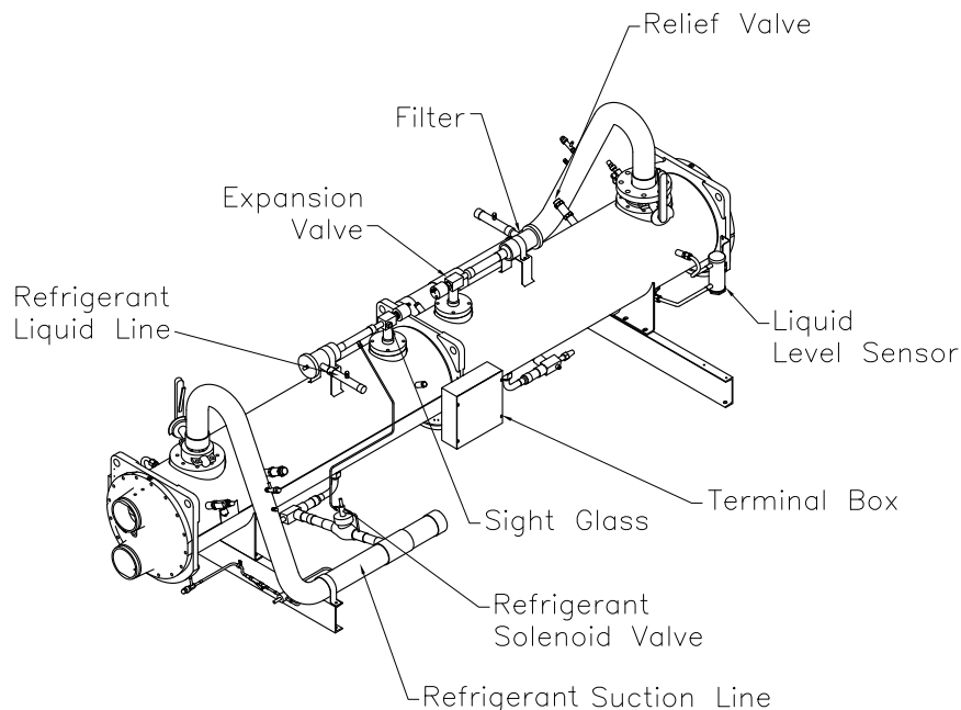
Figure 32. Remote evaporator
