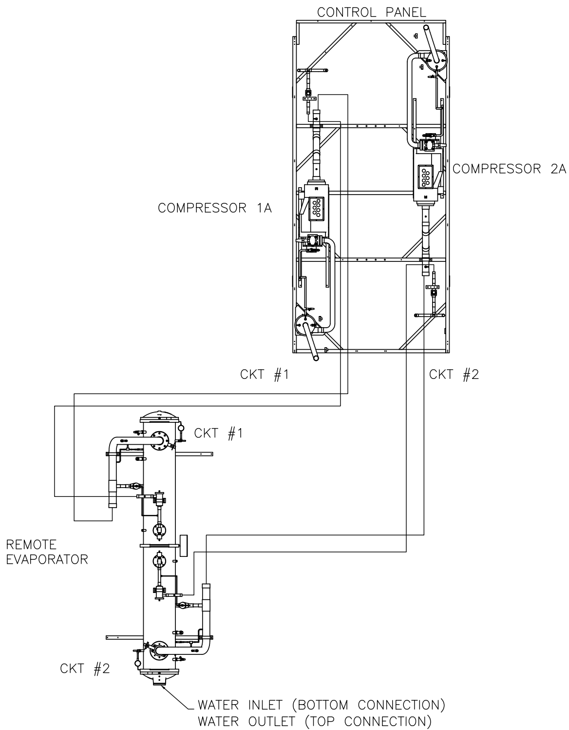
Figure 30. Circuit identification
