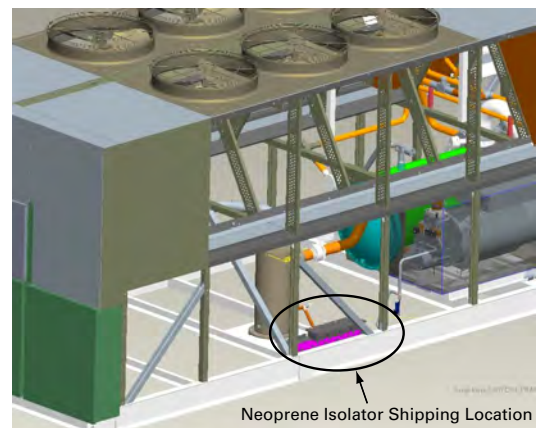
Figure 4. Isolator shipping locations, 275 to 500 ton units
