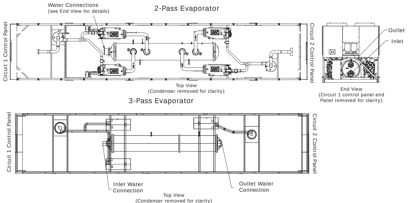
Figure 22. Evaporator pass configurations, 3 or 4 compressor units
