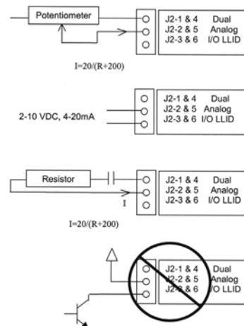
Figure 36. Wiring examples for ECLS and ECWS
