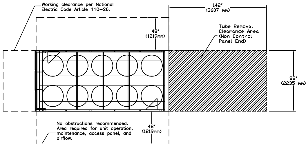
Figure 6. Recommended unit clearances — 18 to 21 foot bases
