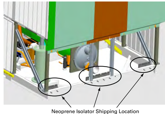
Figure 3. Isolator shipping locations, 140 to 250 ton units
