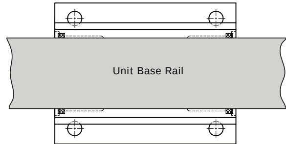
Figure 17. Seismic isolator installation orientation
