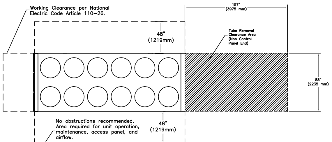
Figure 6. Recommended unit clearances — 18 to 21 foot bases
