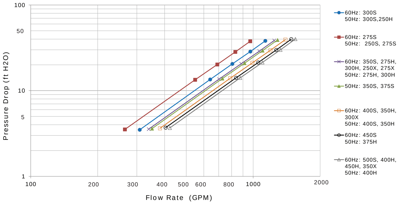
Figure 25. Evaporator water pressure drop, 2-pass evaporator, 250 to 500 tons
