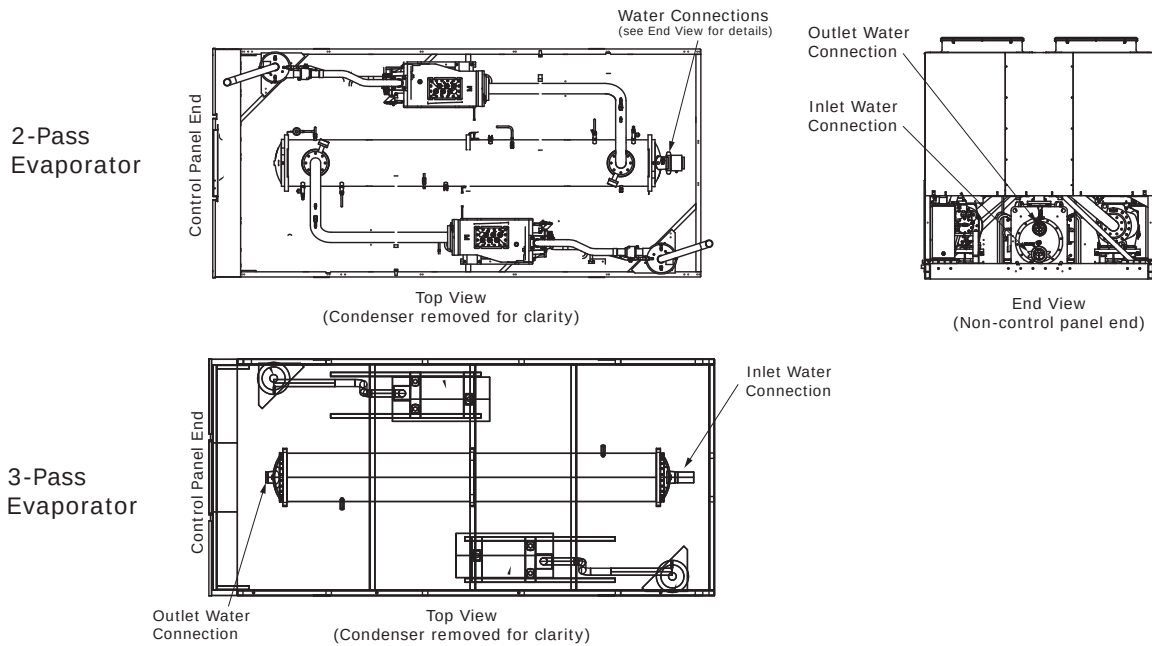
Figure 22. Evaporator pass configurations, 3 or 4 compressor units
