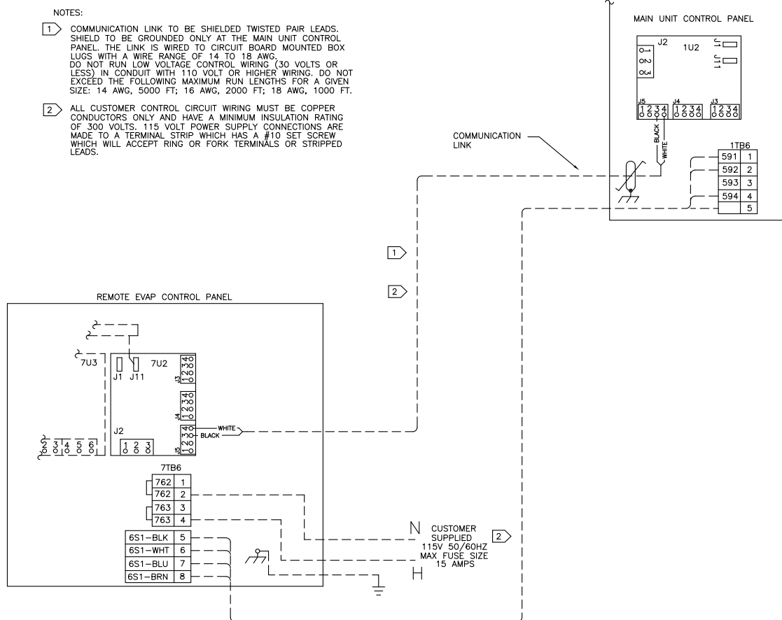
Figure 33. Field wiring between remote evaporator and condensing unit
