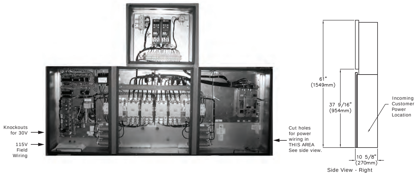
Figure 35. Single point power box (optional on dual panel units)
