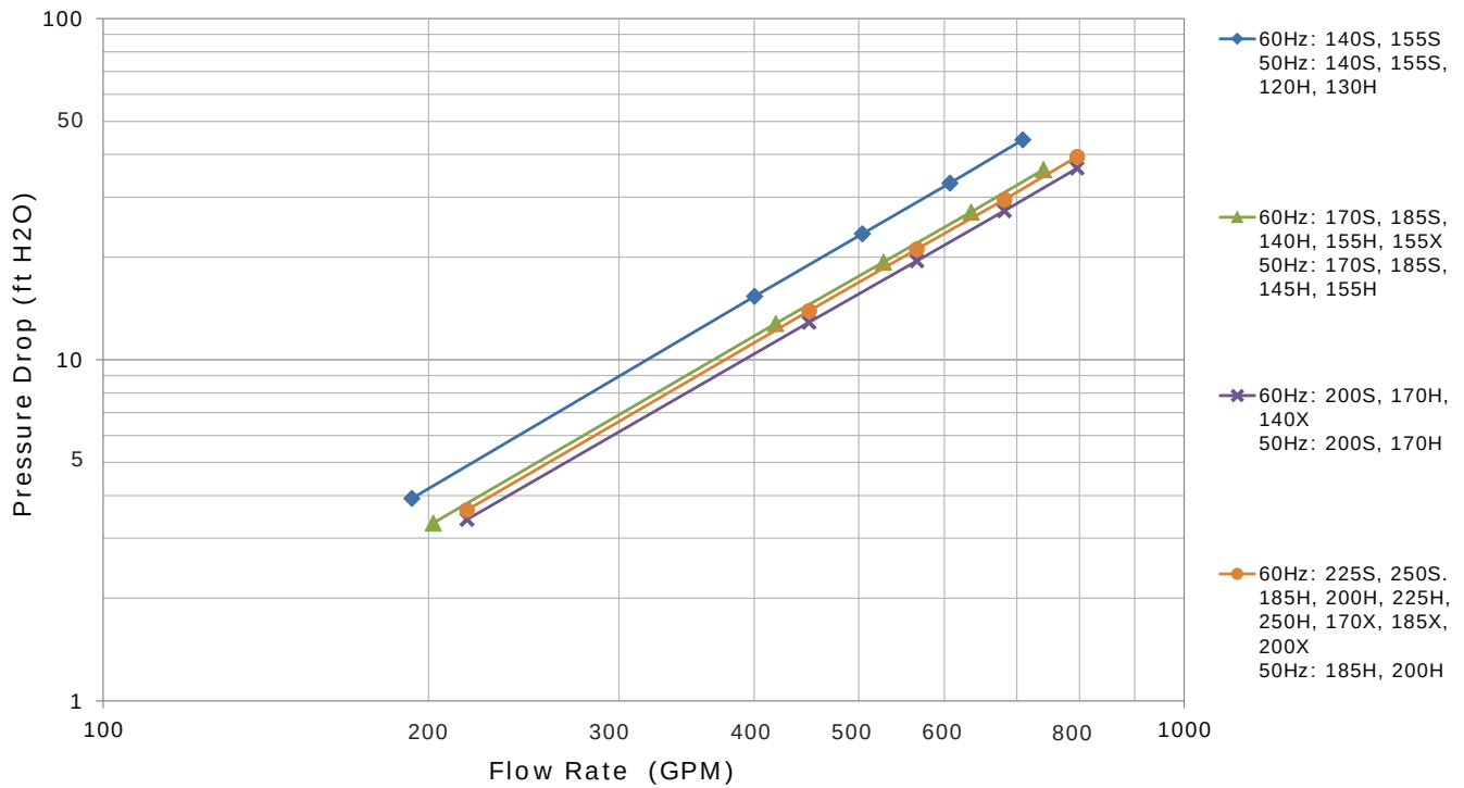
Figure 25. Evaporator water pressure drop, 2-pass evaporator, 250 to 500 tons
