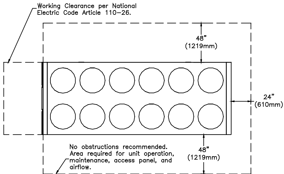
Figure 8. Recommended remote evaporator unit clearances — 15 to 30 foot bases
