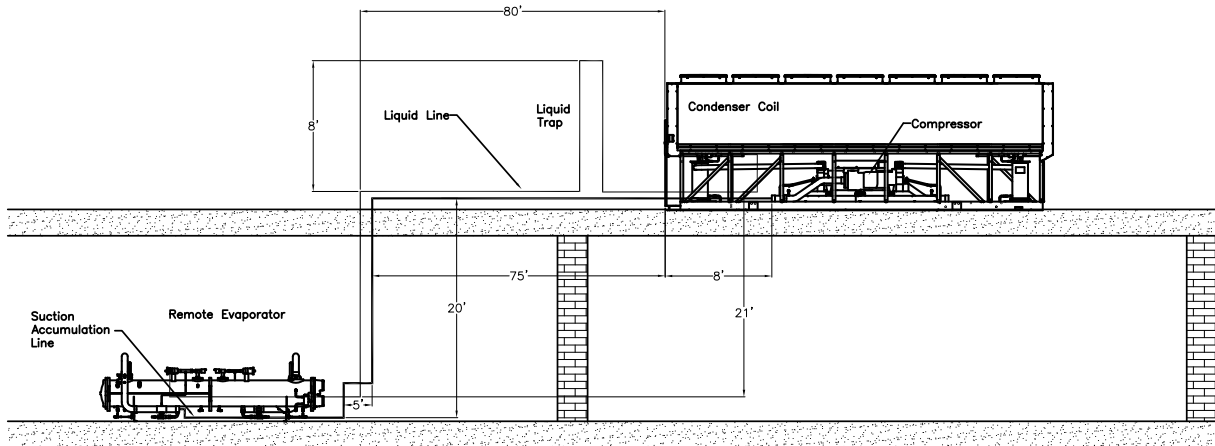
Figure 31. Liquid line sizing example
