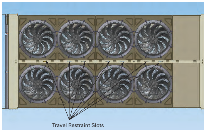
Figure 49. Roof view — travel restraint slots
