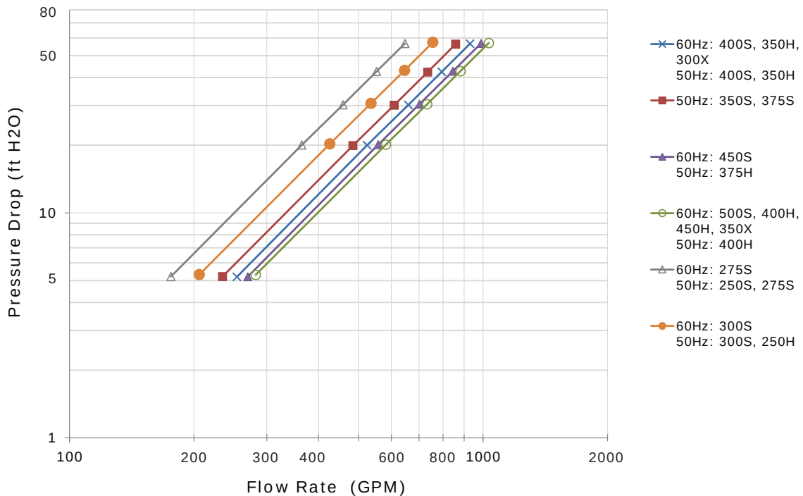
Figure 27. Evaporator water pressure drop, 3-pass evaporator, 250 to 500 tons
