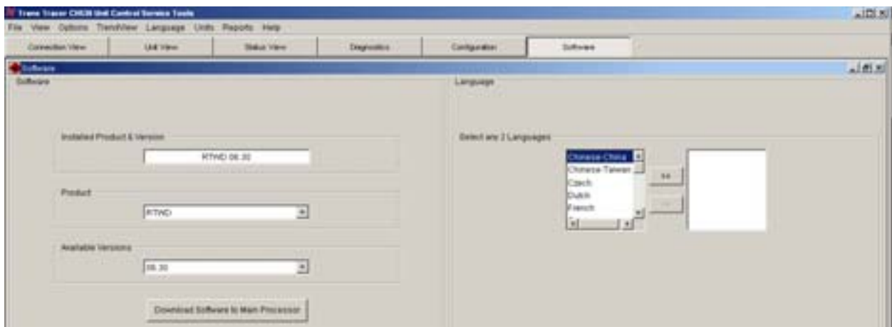
Figure 65. Software view
