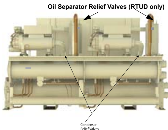
Figure 33. High pressure side relief valves
