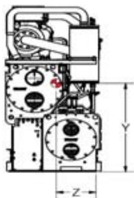
Figure 18. Center of gravity RTWD - High efficiency, 150-250T (60Hz), 130-250T (50Hz) RTWD - Premium efficiency (all) RTUD - 150-250T
