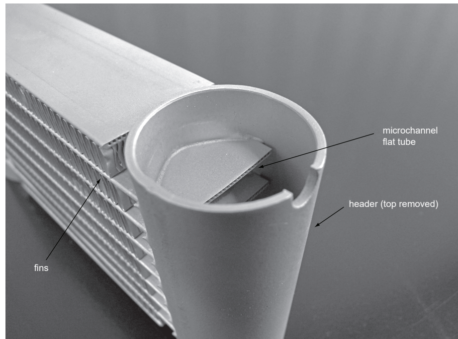
Figure 7. MCHE condenser
