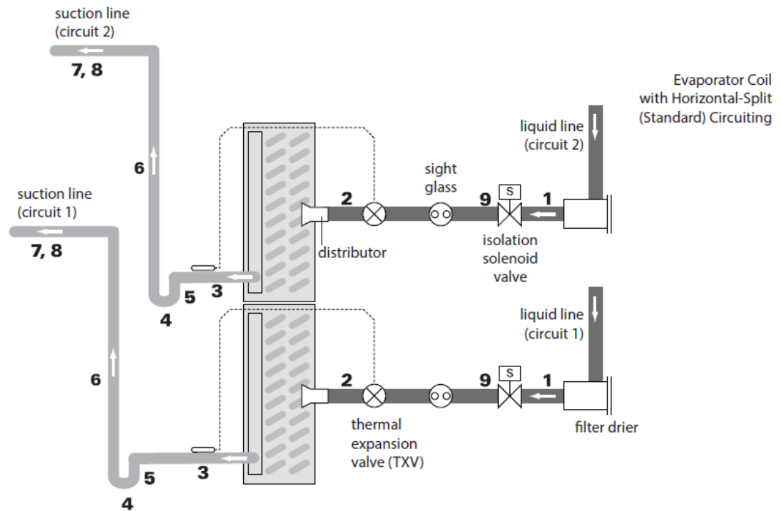
Figure 11. Type UF evaporator coil with two distributors
