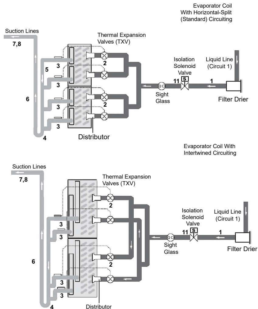
Figure 10. Type UF evaporator coil with four distributors
