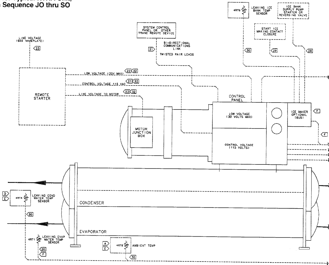
Figure 22 Field Wiring and Remote Sensor Layout for Typical RTHA Unit, Design Sequence JO thru SO
