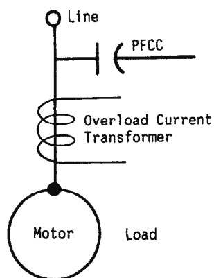
PFCC Connected Before Overload Current Transformer
