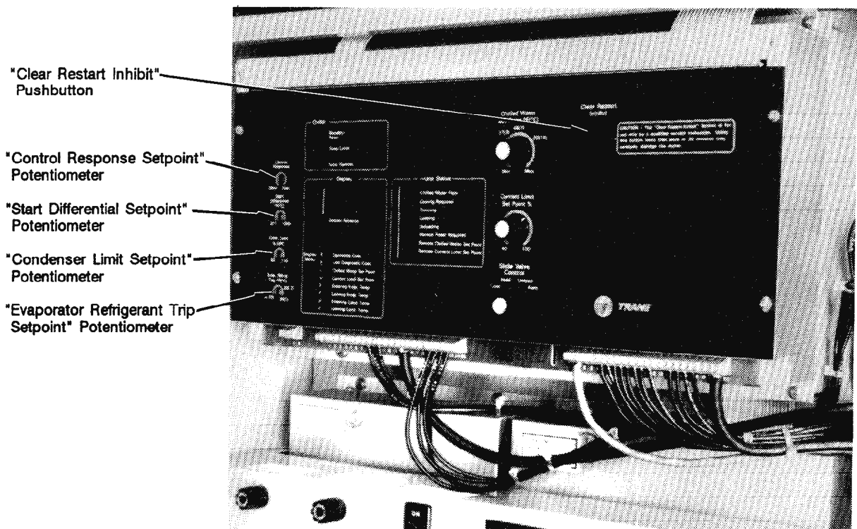
Figure 54 UCM Service Interface Controls (Qualified Technicians Only)
