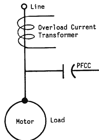
PFCC Between Overload Current Transformer and Motor
