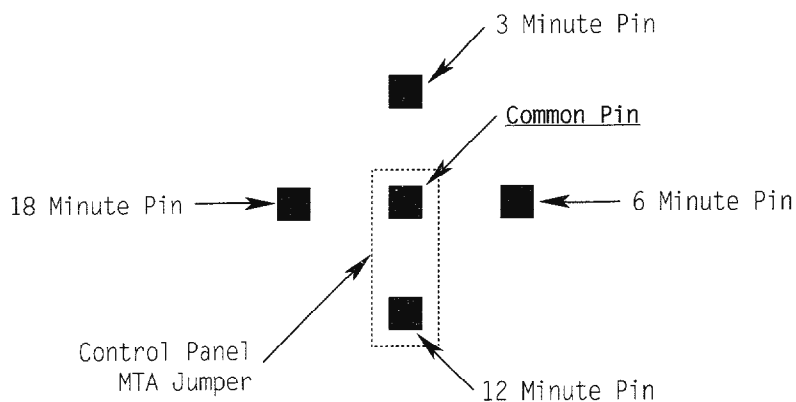
Figure 33 Active Oil Return Time Setting
