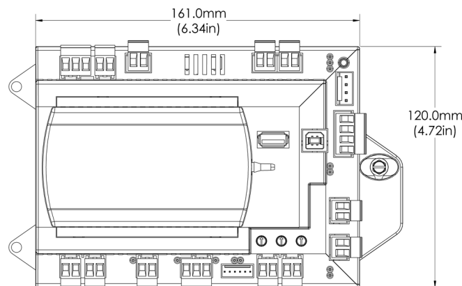
Figure 1. Symbio 210 dimensions without actuator
