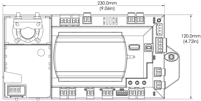
Figure 2. Symbio 210 dimensions with actuator
