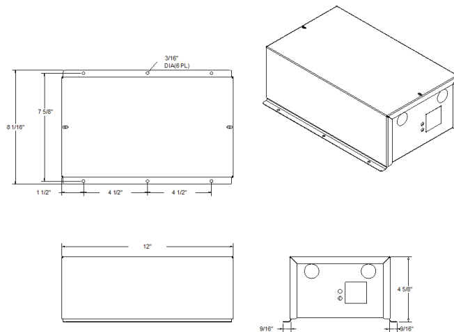
Figure 4. Optional Symbio 210 control box 501897940100 dimensions
