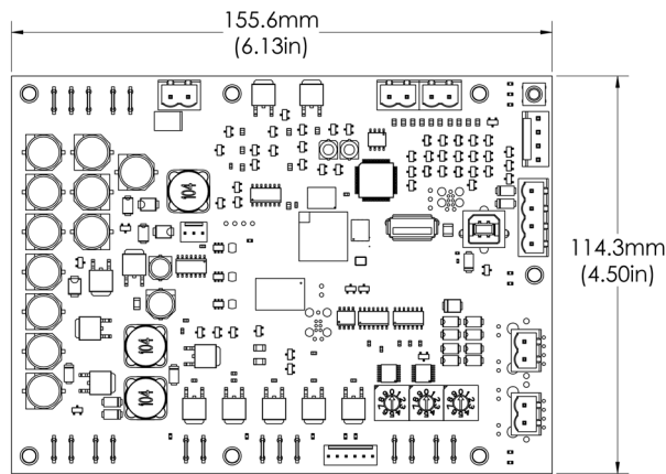
Figure 3. Symbio 210 dimensions (Trane VAV factory version)
