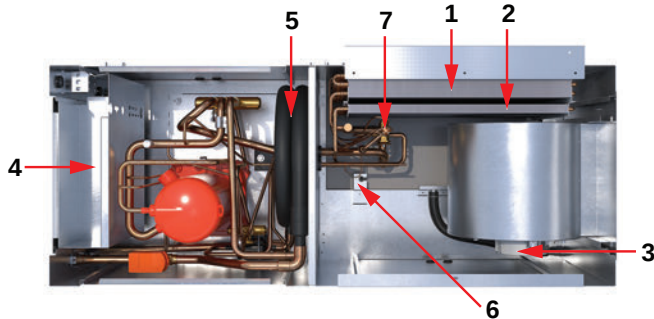
Figure 1. EXH/DXH unit
