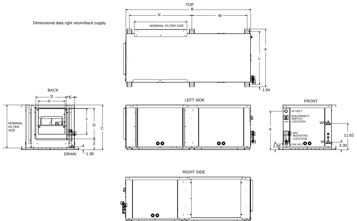
Figure 25. Right return/back supply (EXHG/DXHG)
