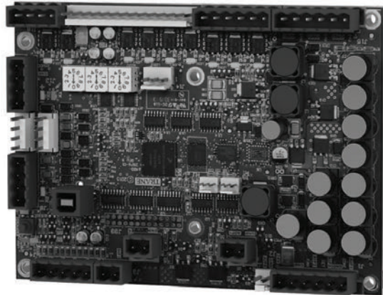
Figure 18. Tracer® UC400B
