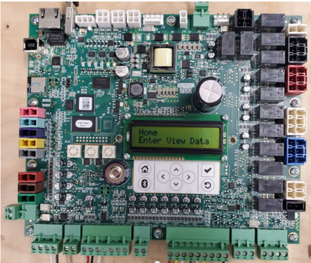
Figure 14. Symbio 700 controller
