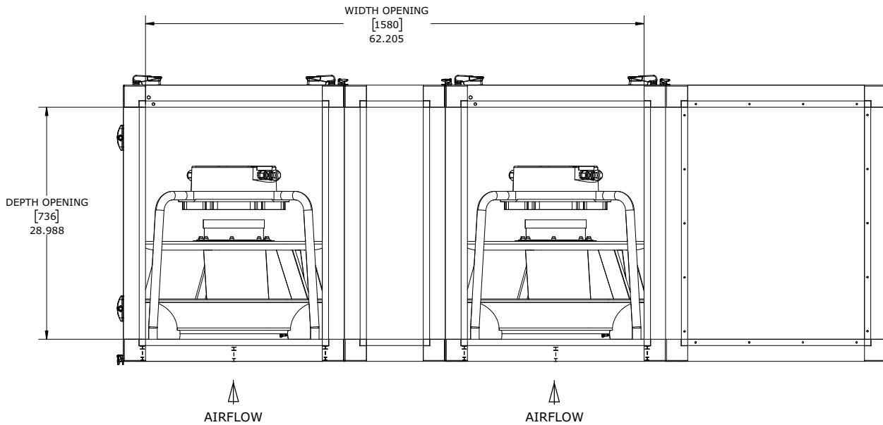
Figure 13. Discharge opening for 70-80 ton
