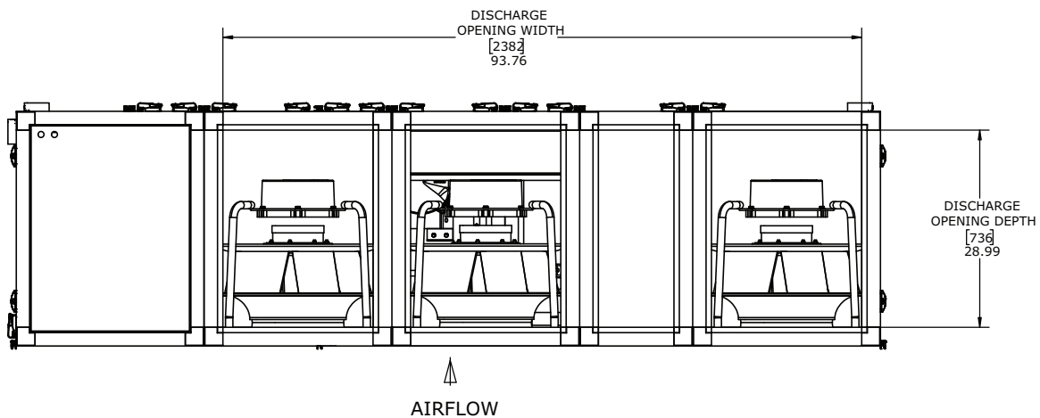
Figure 13. Discharge opening for 70-80 ton
