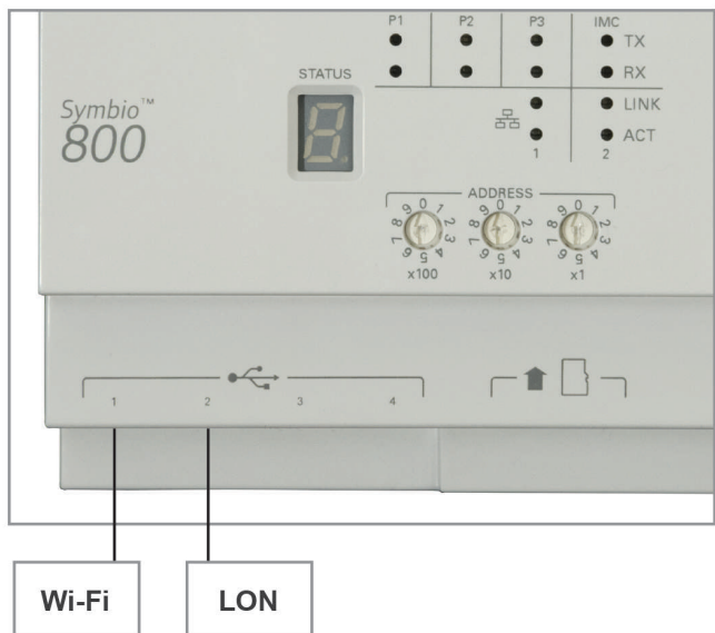
Figure 13. (4) USB connectors
