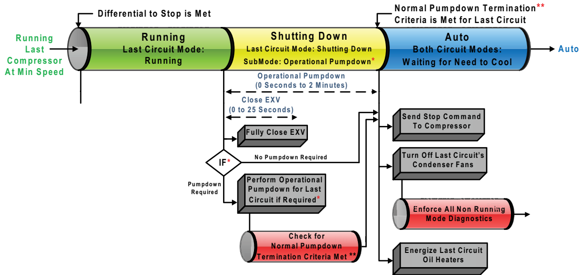
Figure 58. Sequence of events: satisfied setpoint
