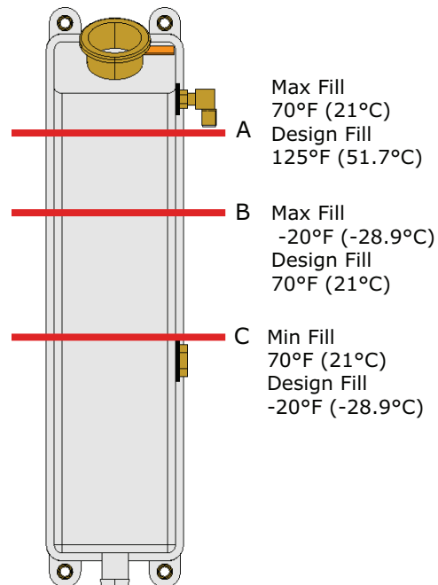
Figure 66. Drive cooling expansion tank fill
