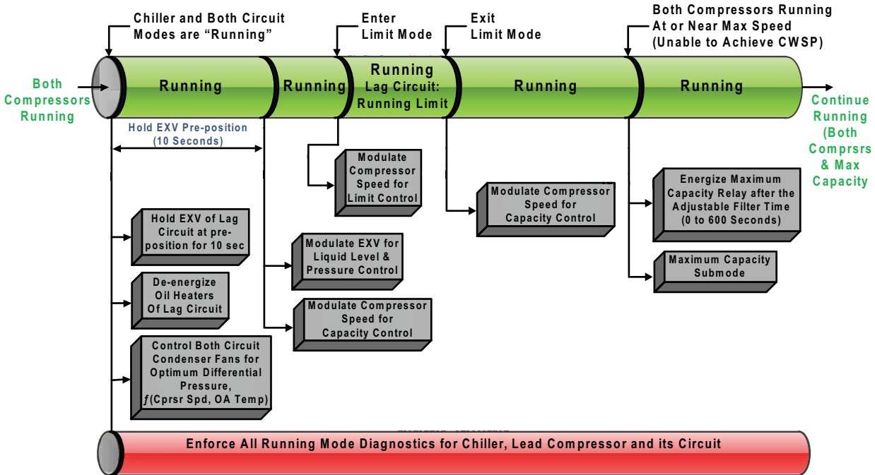
Figure 57. Sequence of operation: running (lag compressor/circuit start and run)
