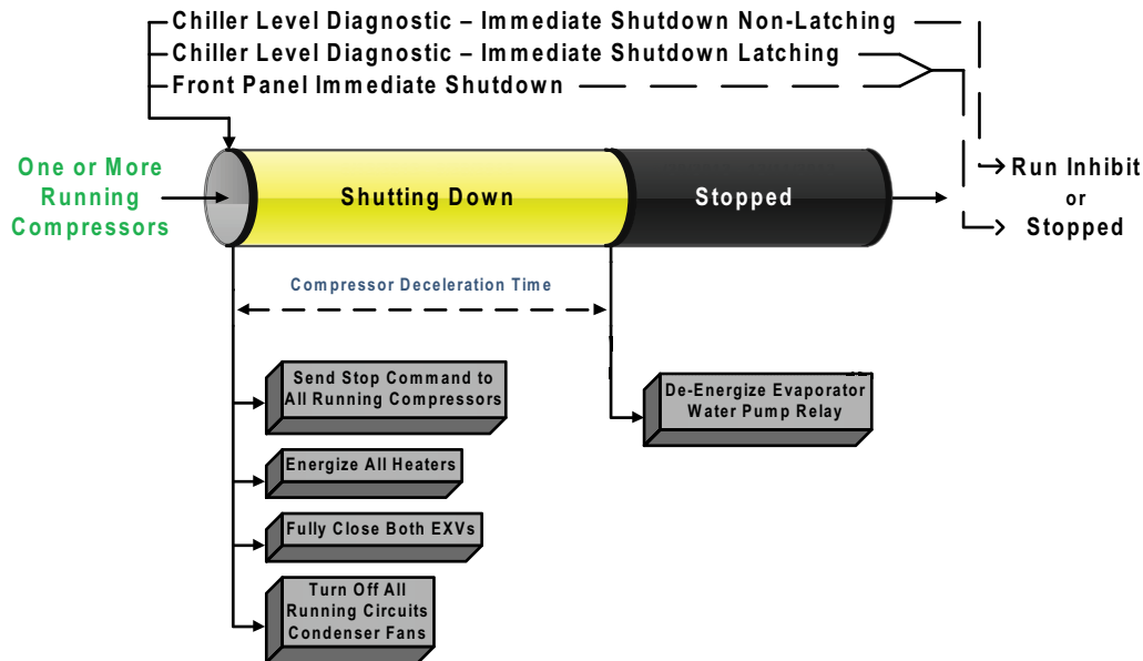
Figure 60. Sequence of events: immediate shutdown to stopped or run inhibit
