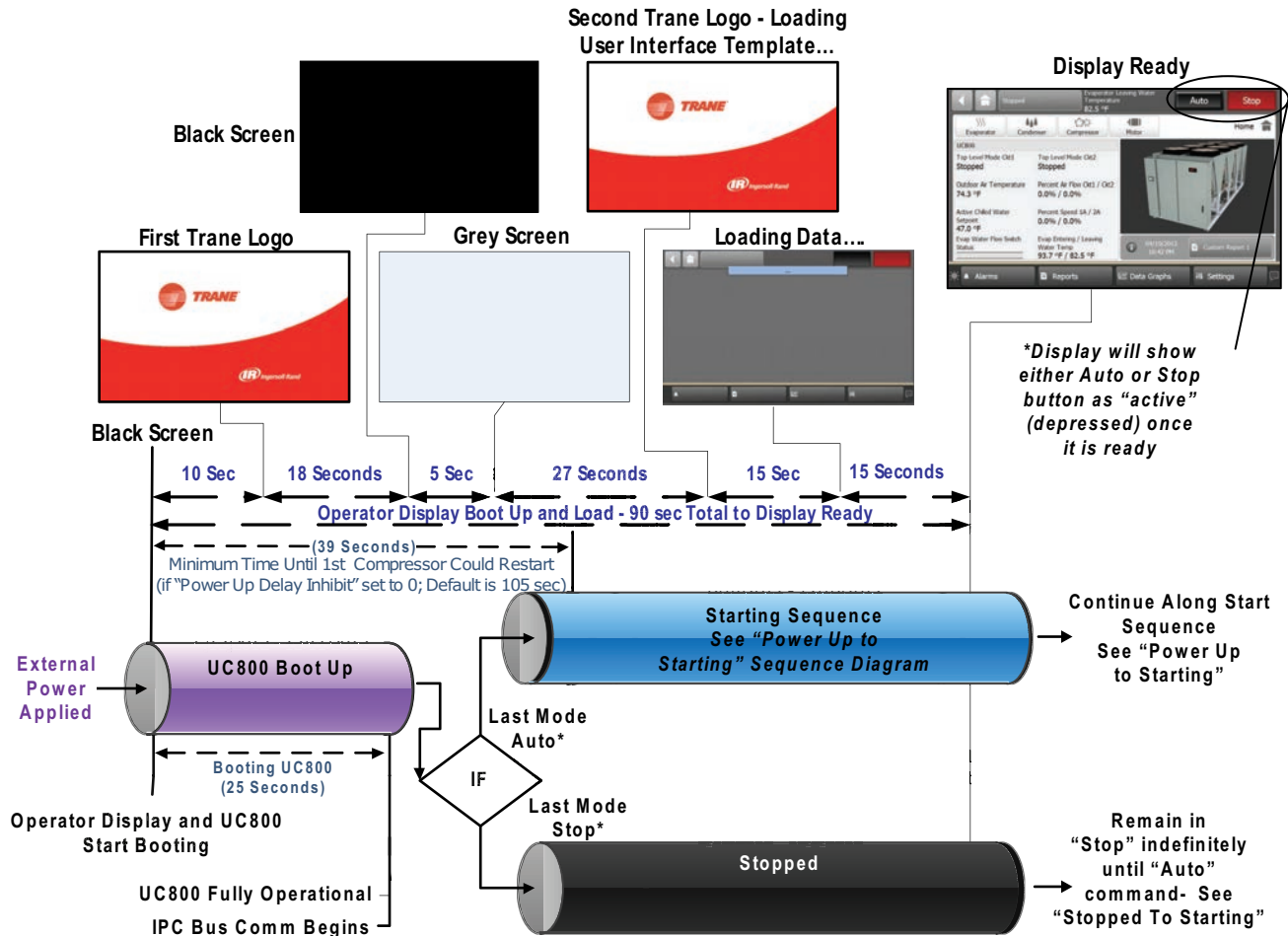
Figure 53. Sequence of operation: power up diagram
