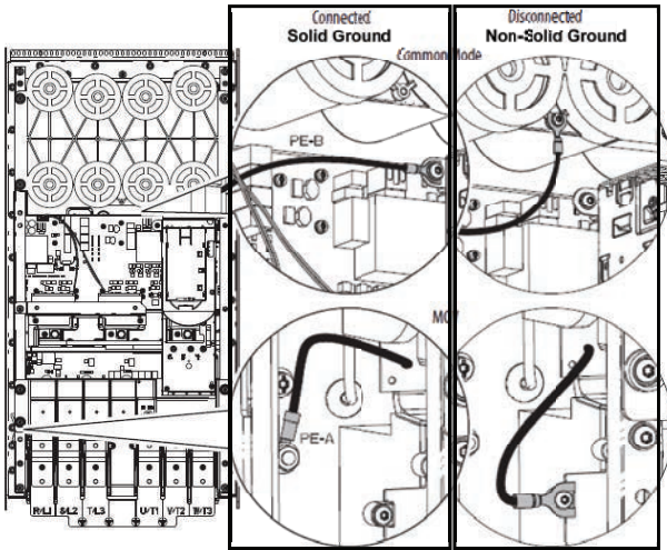
Figure 22. AFD frame 7 power jumper locations
