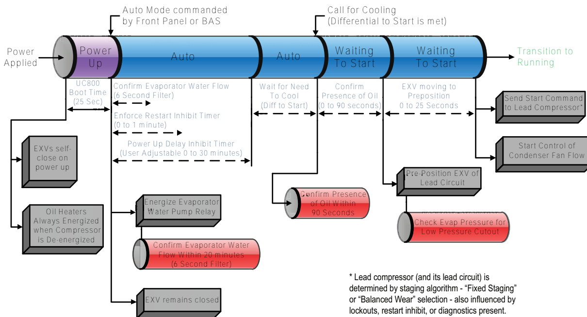
Figure 54. Sequence of events: power up to starting
