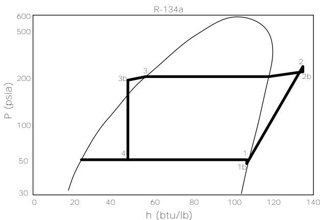
Figure 26. Pressure-enthalpy (P-h) diagram
