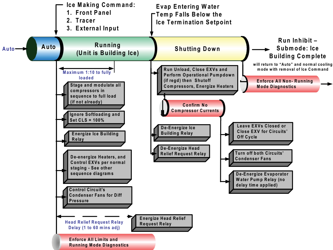
Figure 62. Sequence of events: ice making (auto to ice making to ice making complete)
