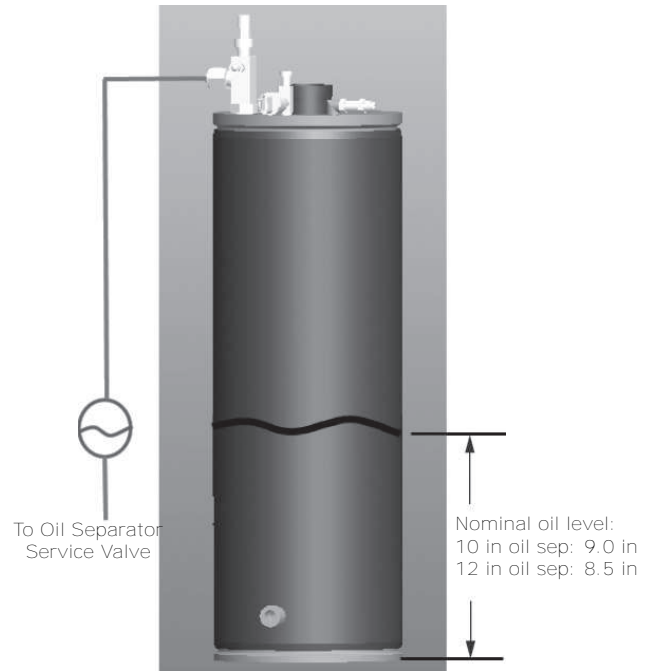
Figure 64. Nominal oil level
