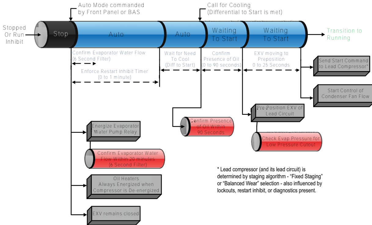
Figure 55. Sequence of events: stopped to starting
