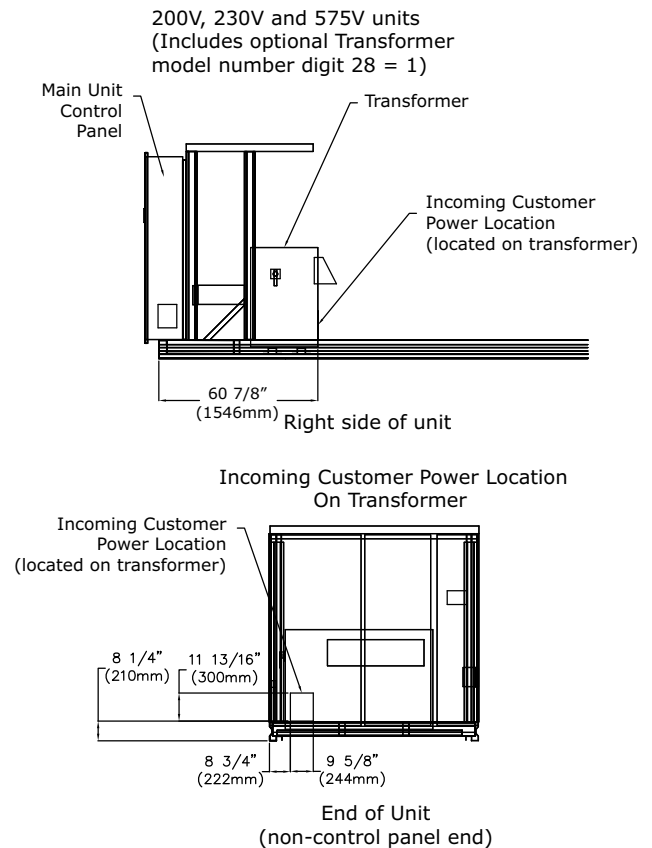
Figure 24. Incoming customer power – transformer
