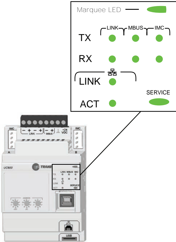
Figure 28. LED locations
