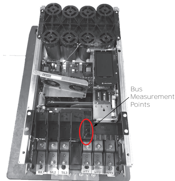
Figure 20. Bus measurement nodes detail
