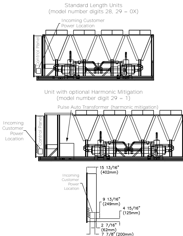
Figure 23. Incoming customer power – control panel (right side view)
