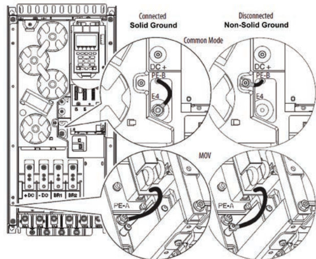
Figure 21. AFD frame 6 power jumper locations
