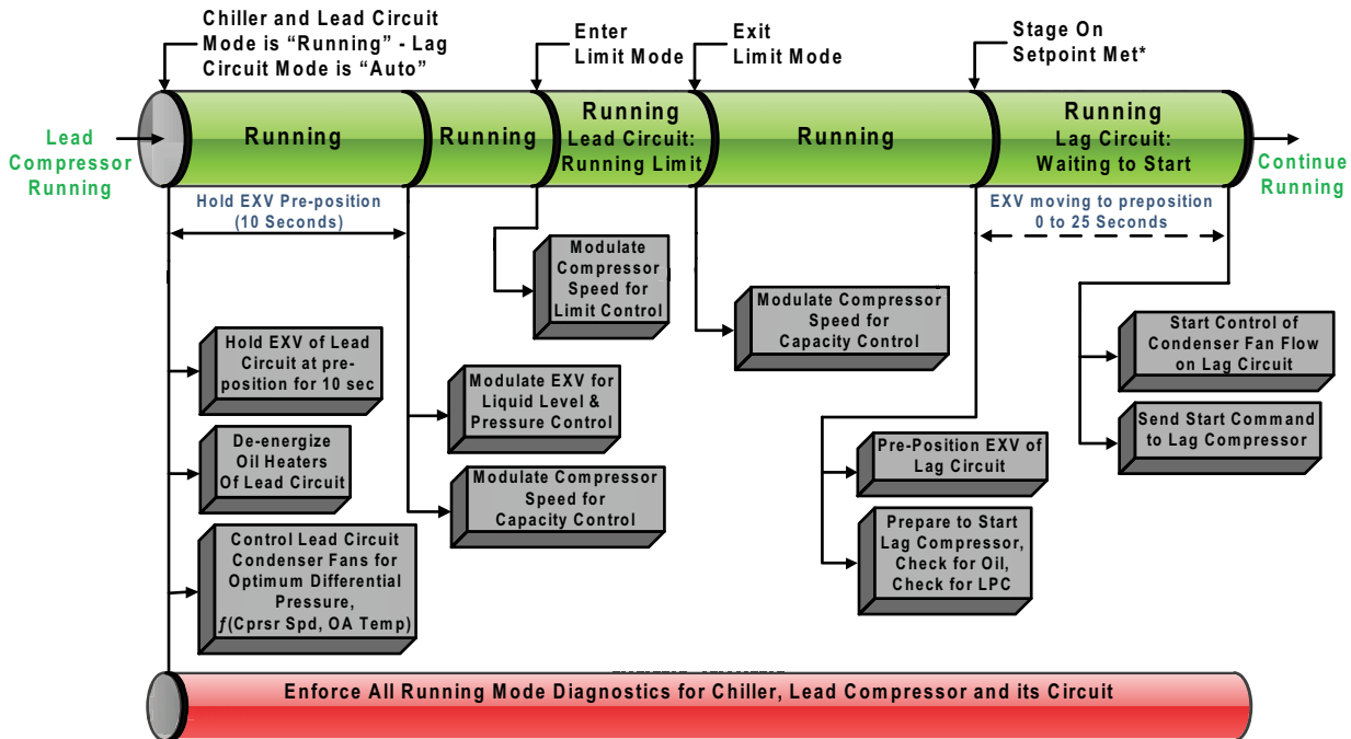
Figure 56. Sequence of operation: running (lead compressor/circuit start and run)
