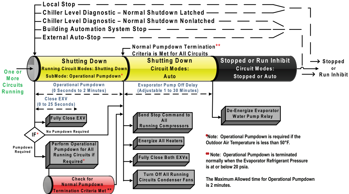
Figure 59. Sequence of events: normal shutdown to stopped or run inhibit
