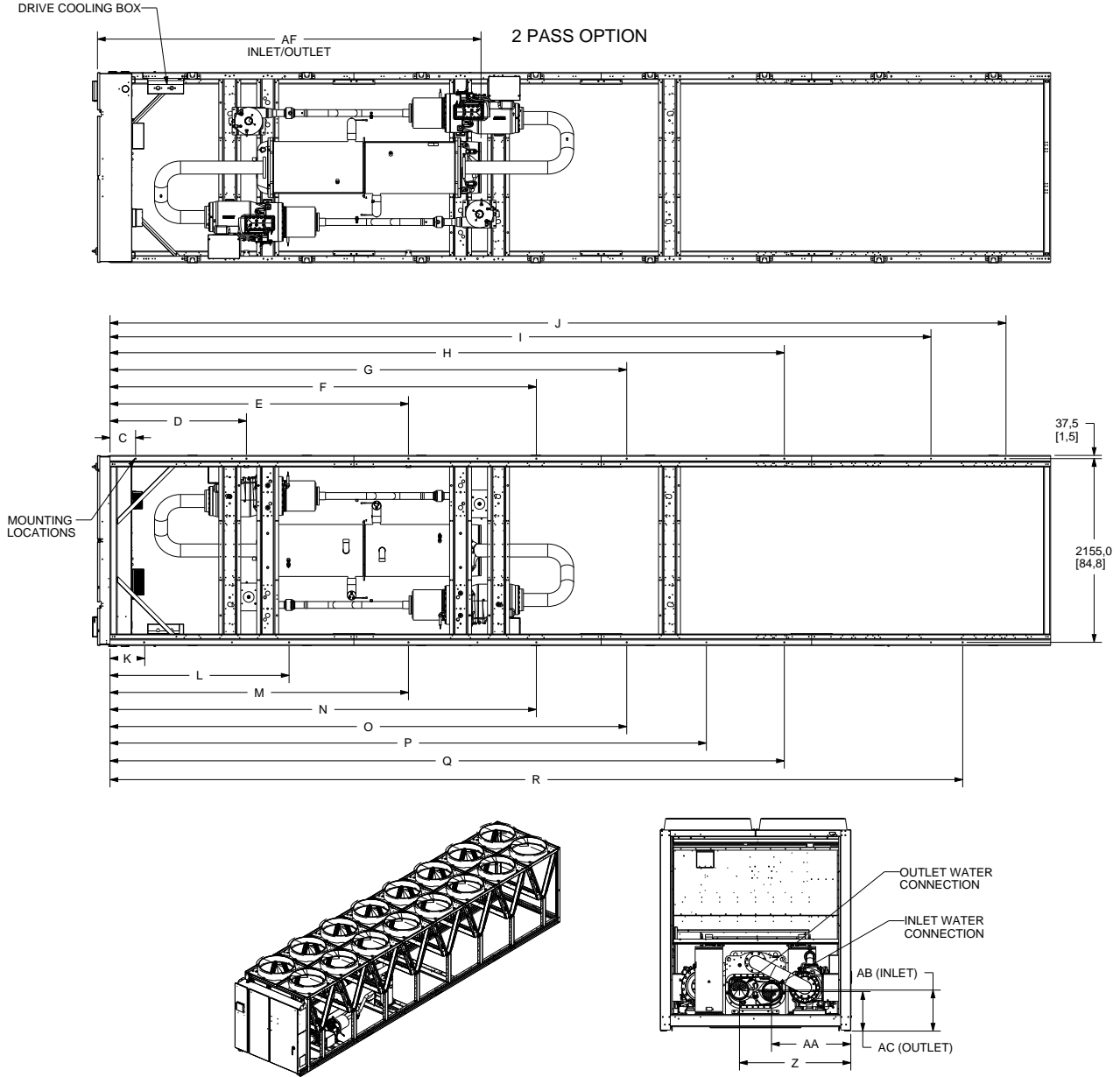
Figure 9. Dimensions — 150 to 300 ton units, standard length, 2-pass
