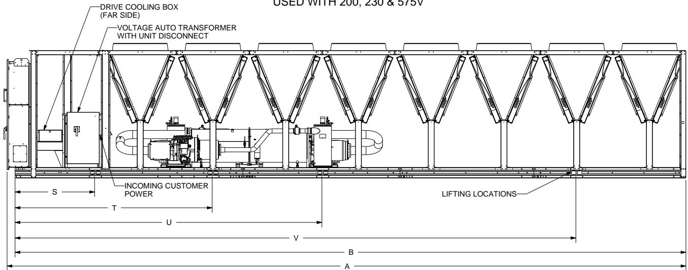
Figure 11. Dimensions – 150 to 300 ton units, extended length
