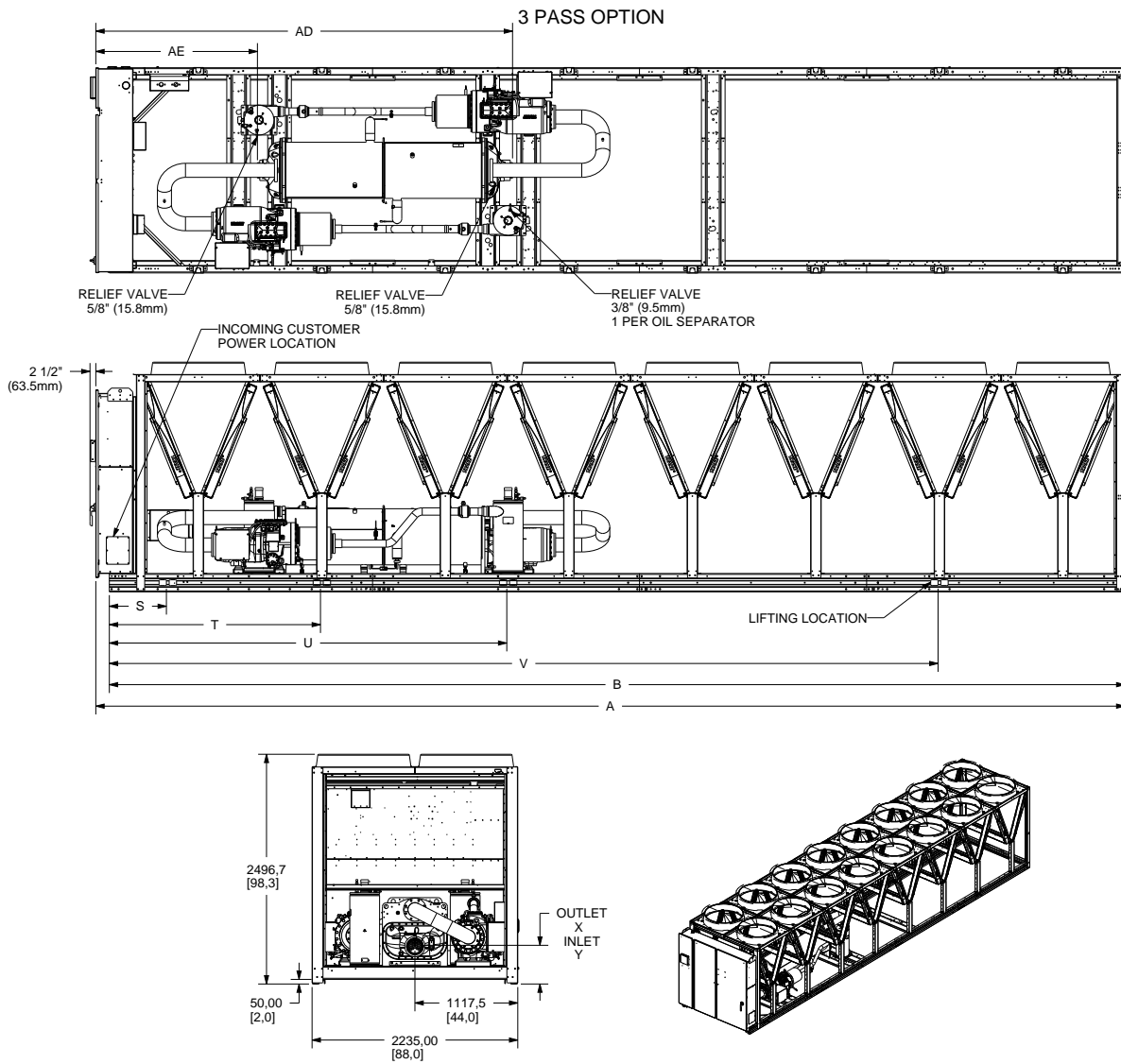
Figure 10. Dimensions – 150 to 300 ton units, standard length, 3-pass
