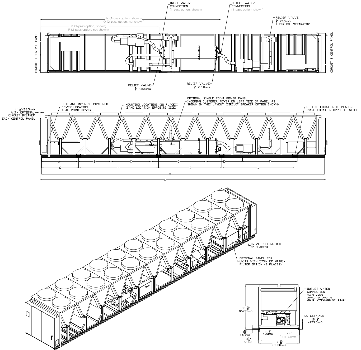
Figure 13. Dimensions – units larger than 300 tons, units without direct-free cooling
