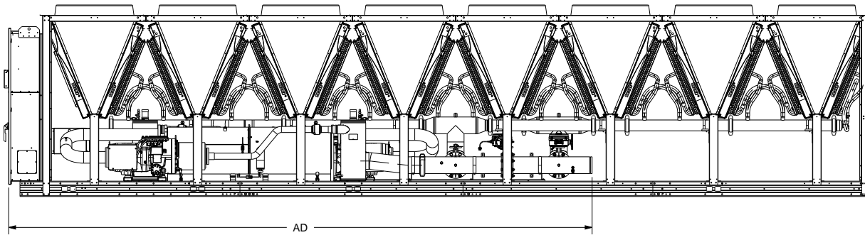
Figure 12. Water connection dimensions – 150 to 300 ton units with free-cooling or pump package option
