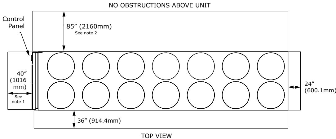
Figure 8. Unit service clearance requirements — units larger than 300 tons
