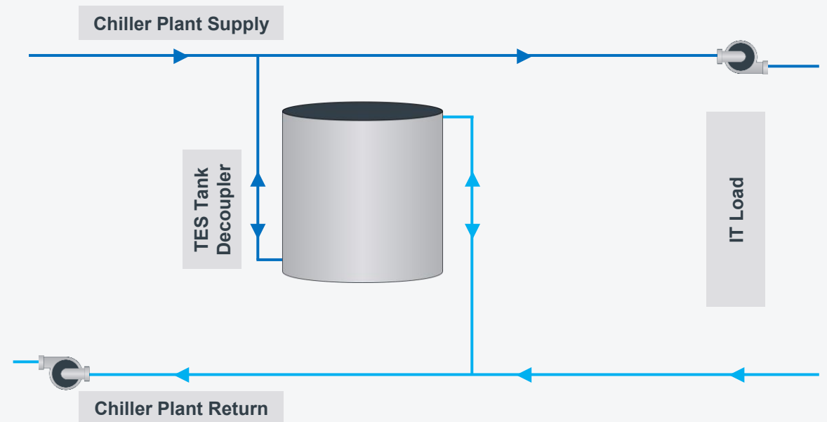
Thermal storage tank in the decoupler pipe
