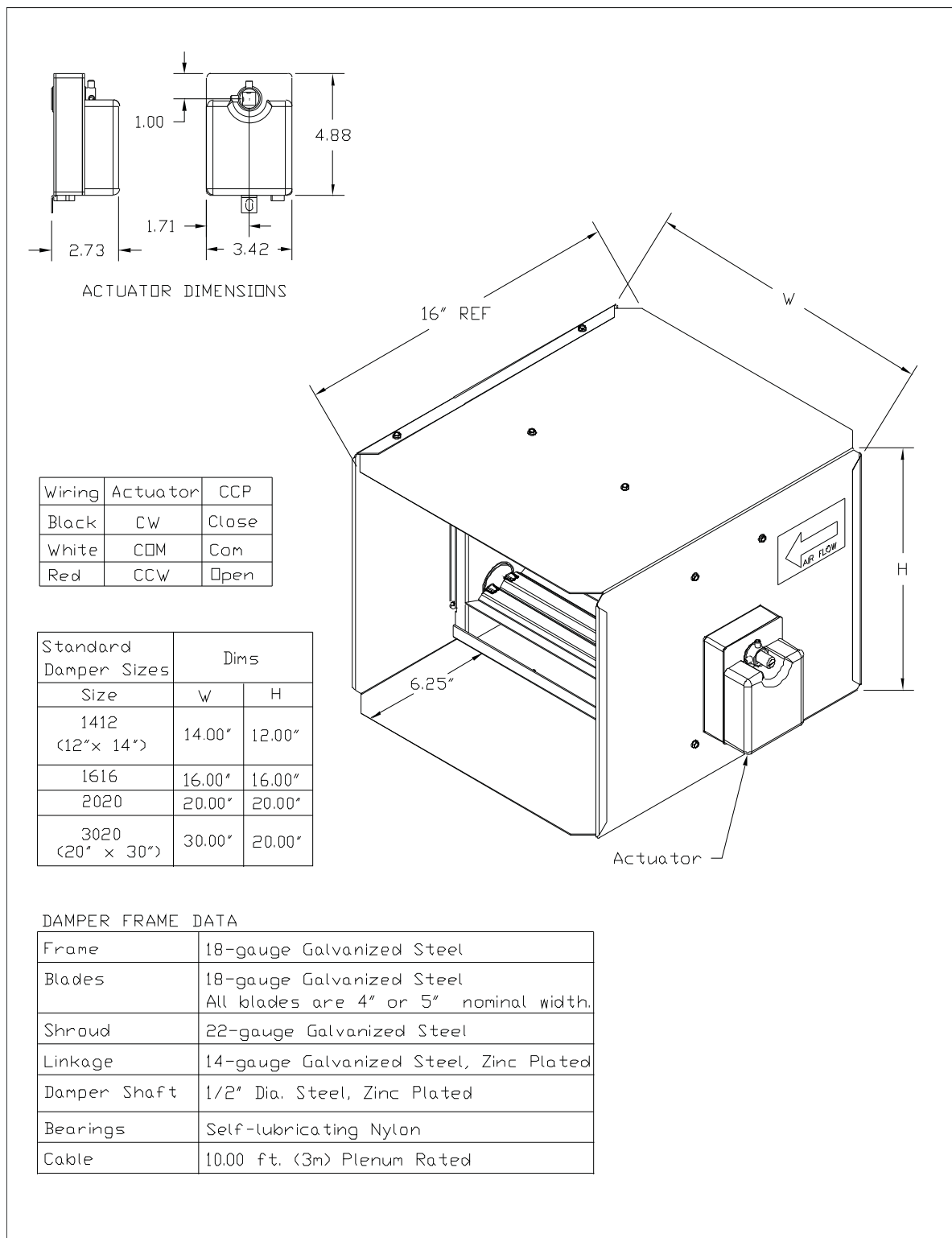
Figure 41. Rectangular bypass damper dimensions
