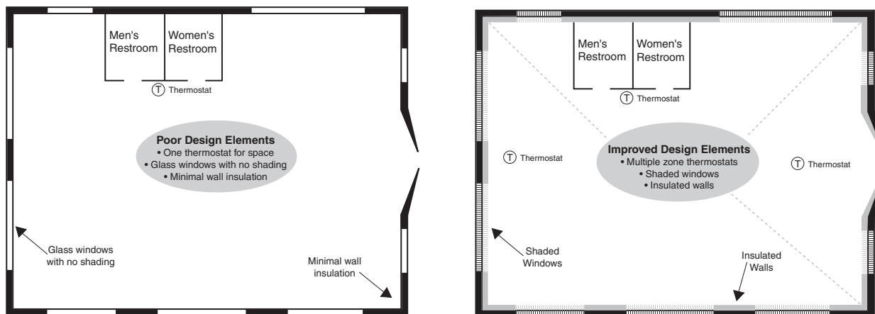
Figure 15. Building Example 1 illustrates a small, poorly insulated office on the left, and improved design on the right.
