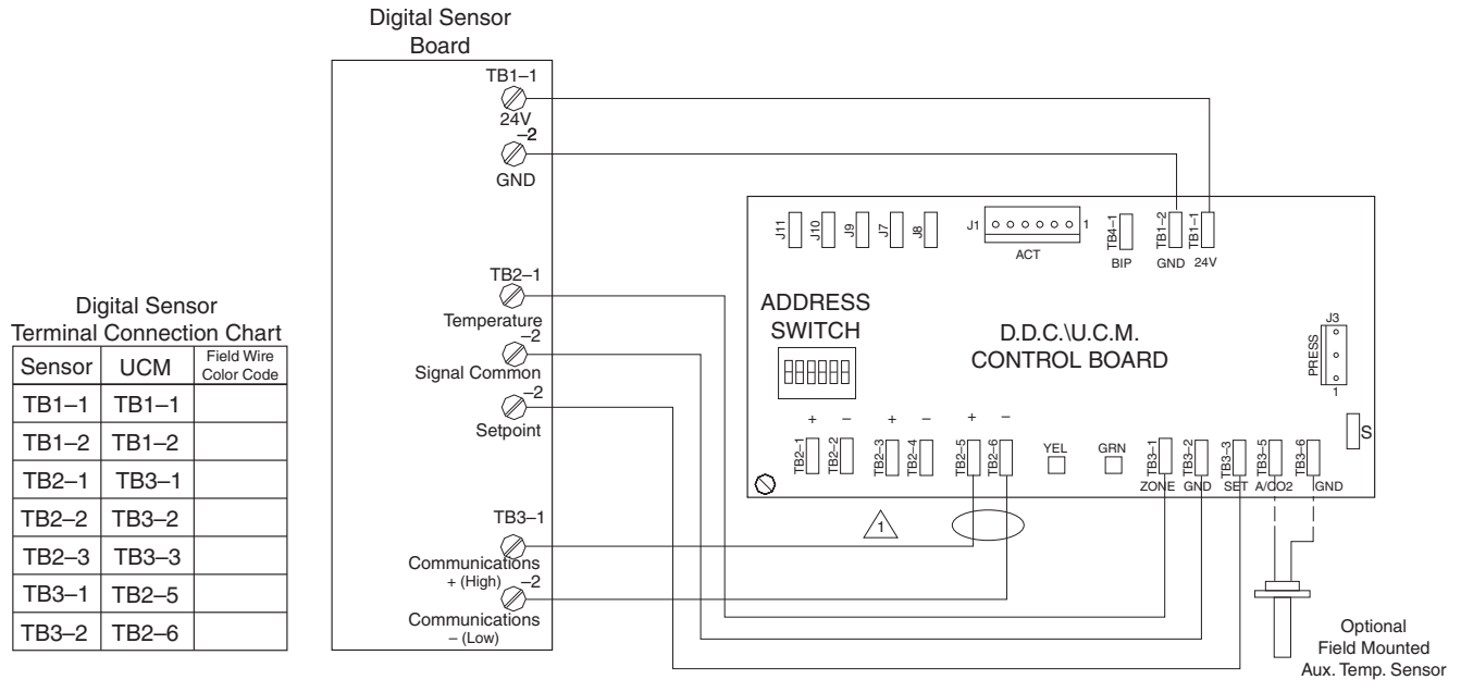
Figure 35. DDC zone sensor with LCD
