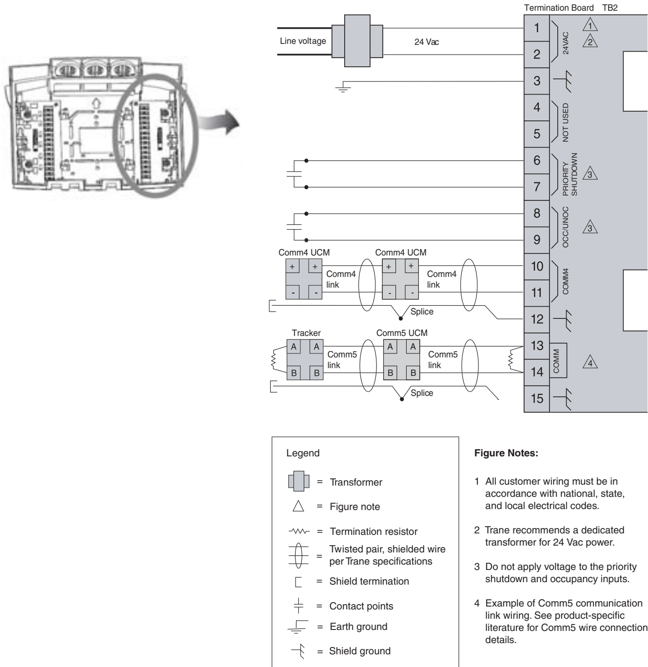
Figure 29. Central control panel field wiring
