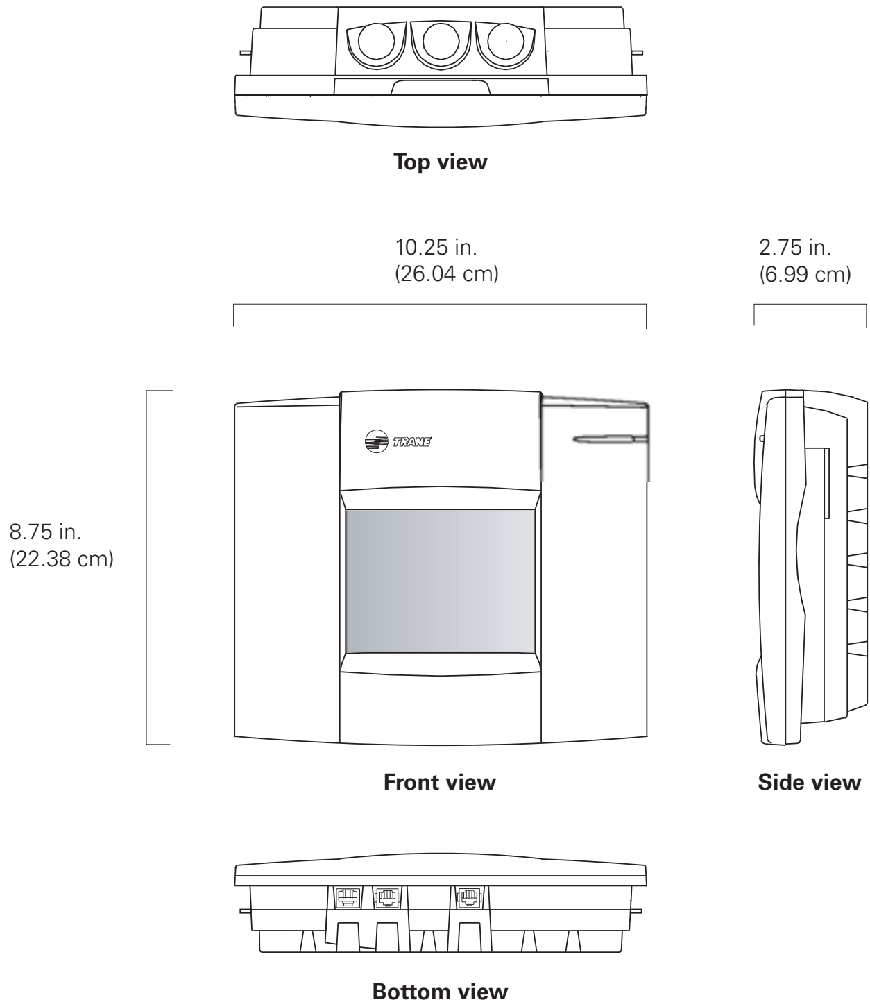
Figure 37. Central control panel dimensions
