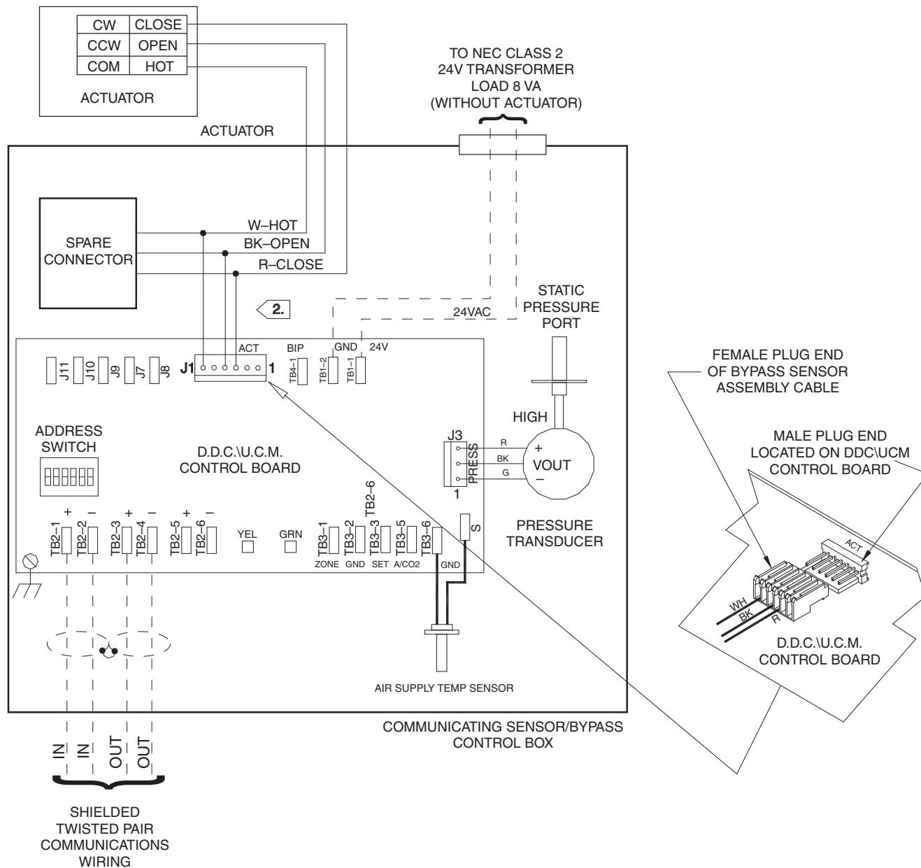
Figure 33. Communicating bypass controller wiring
