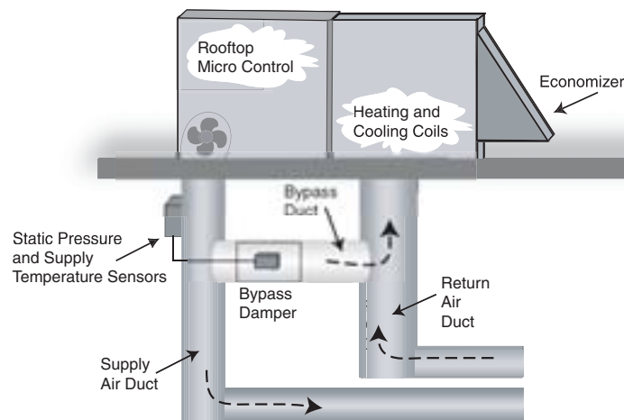
Figure 25. Changeover bypass variable-air-volume system
