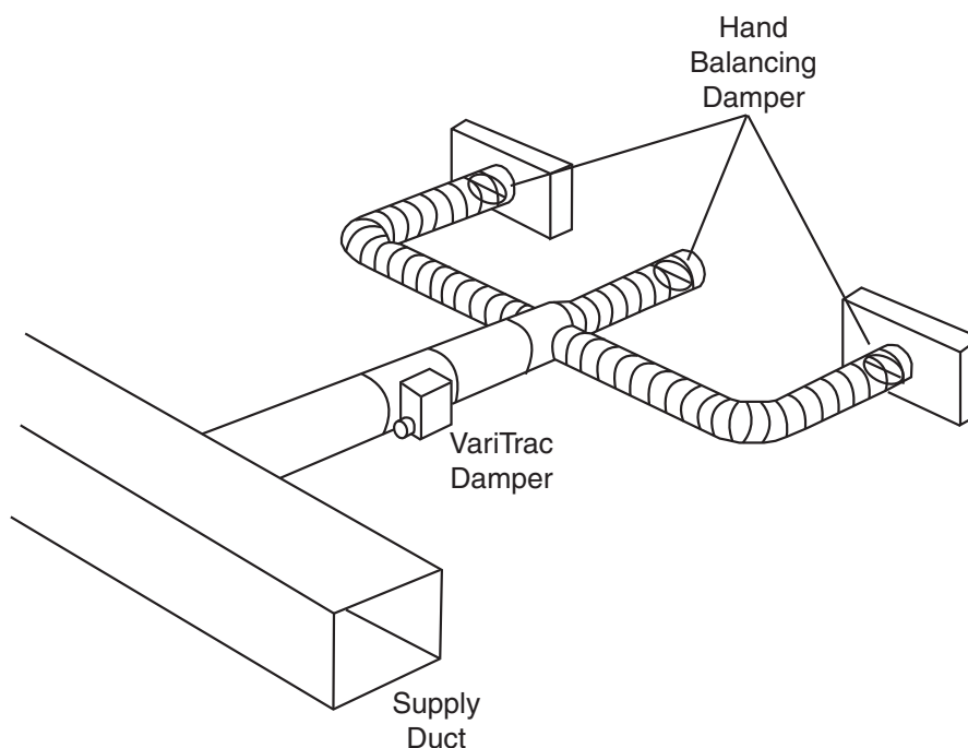
Figure 18. Hand balancing dampers
