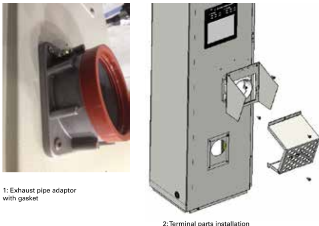
Figure 13 - Exhaust gas terminal installation
