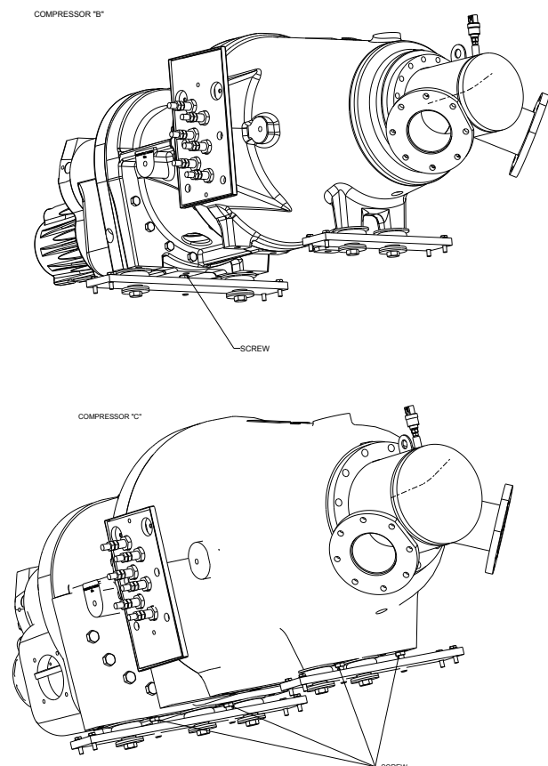
Figure 4 – Shipping spacer and brackets to be removed prior to unit startup
