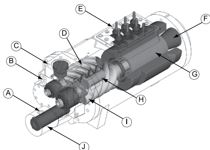
Figure 11 – RTWF compressor description
