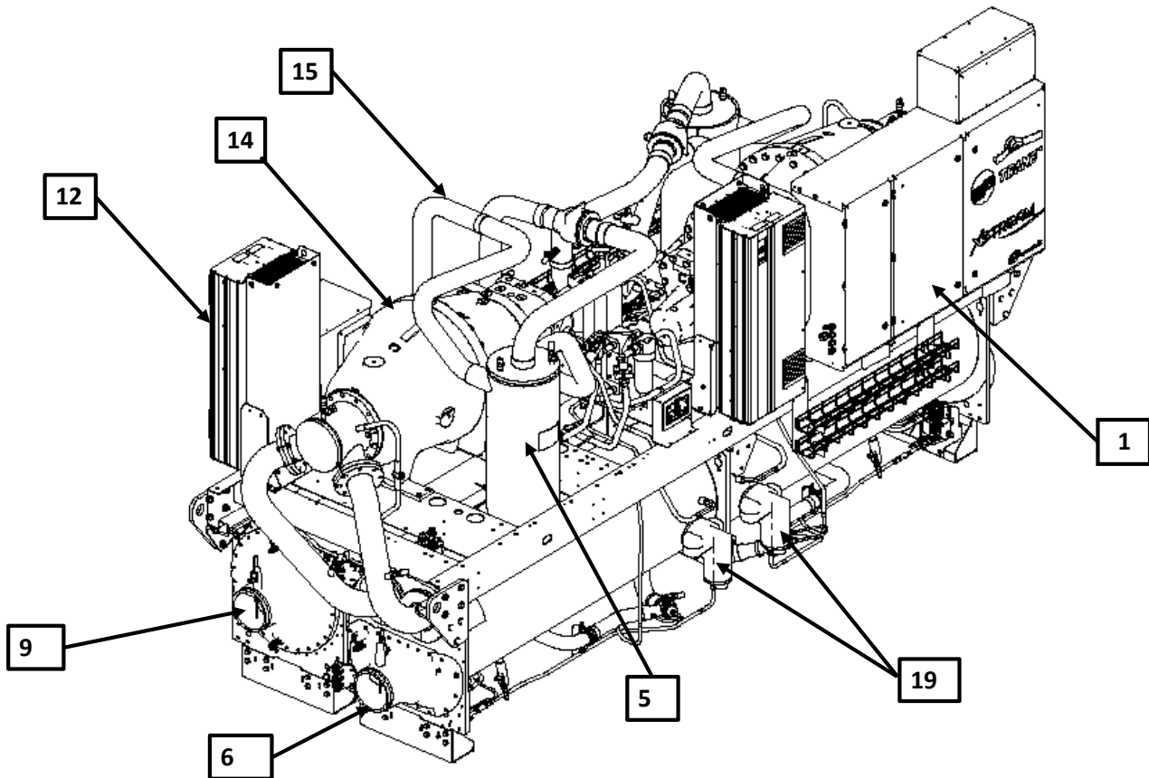
Figure 2 – Component Location for Typical RTHF Unit
