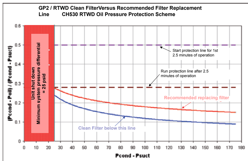
Figure 14 – Oil Filter Replacement Chart for RTWF
