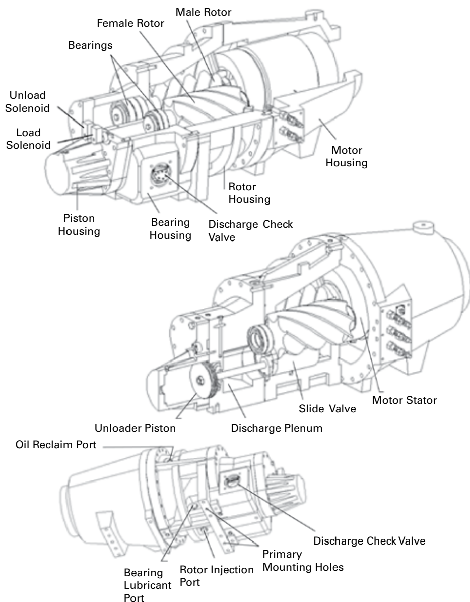
Figure 10 – CHHC - RTHF compressor description
