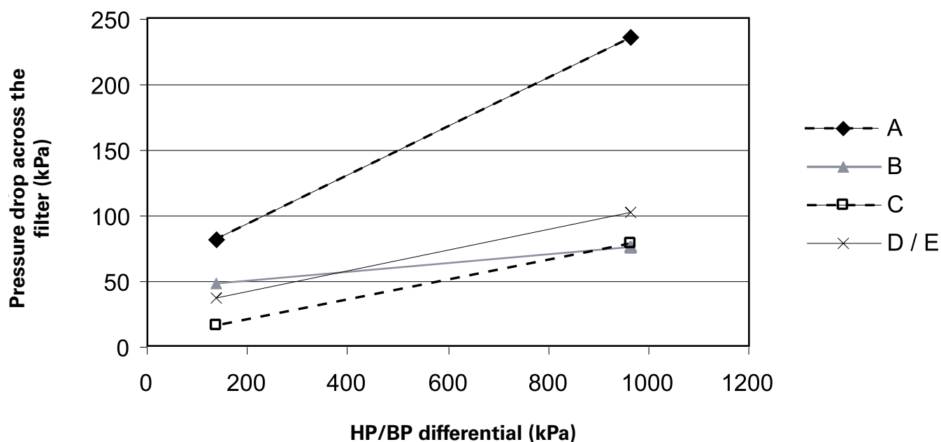
Figure 13 – Oil Filter Replacement Chart for RTHF
