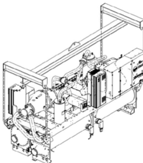
Figure 3 – Example of spreader to be used to lift RTHF-RTWF
