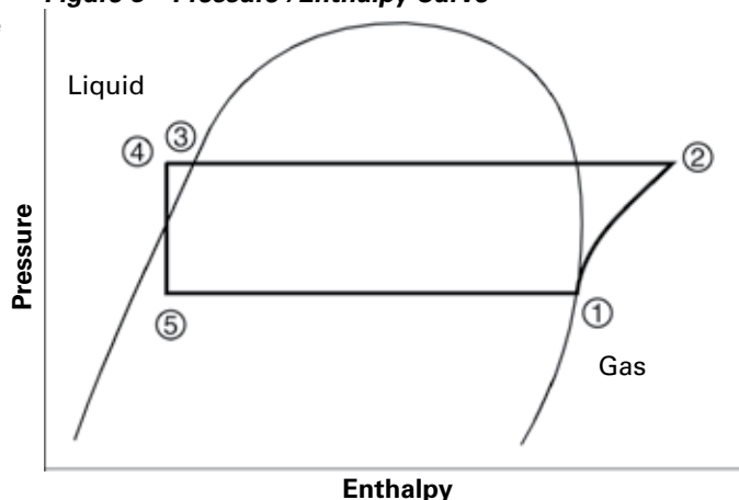
Figure 8 – Pressure /Enthalpy Curve
