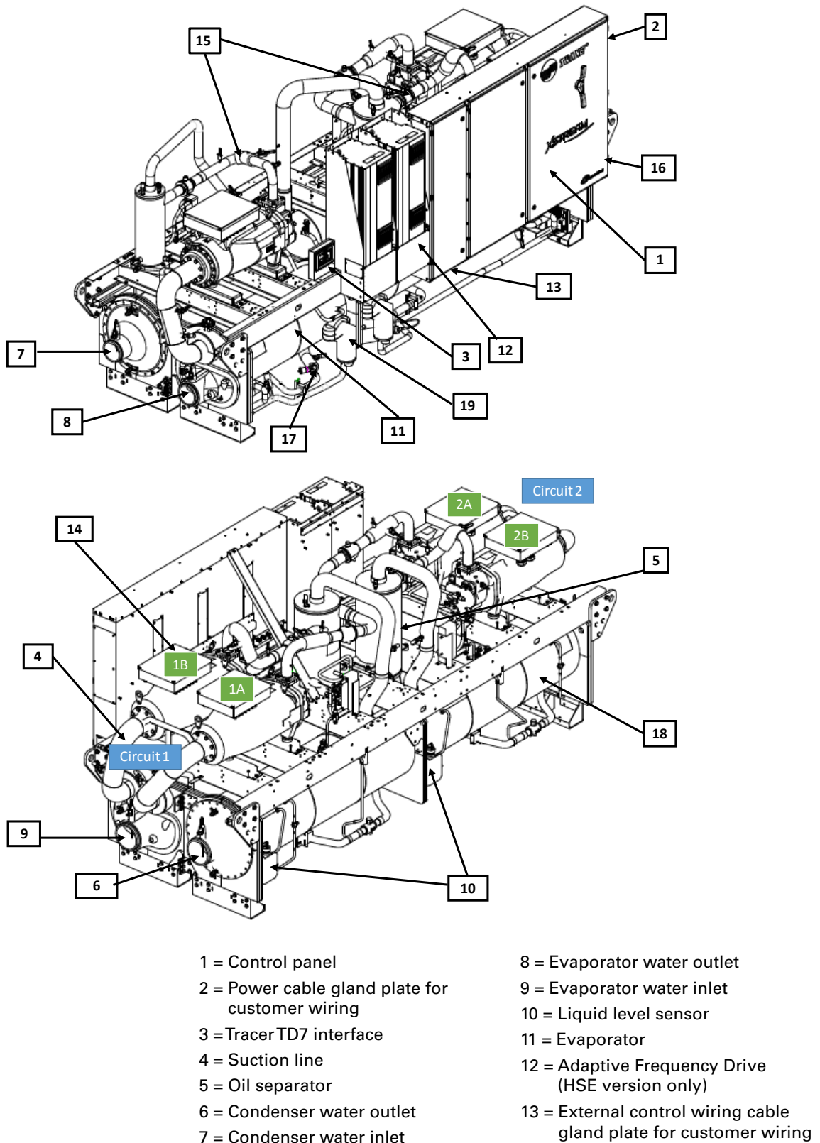
Figure 1 – Component Location for Typical RTWF Unit
