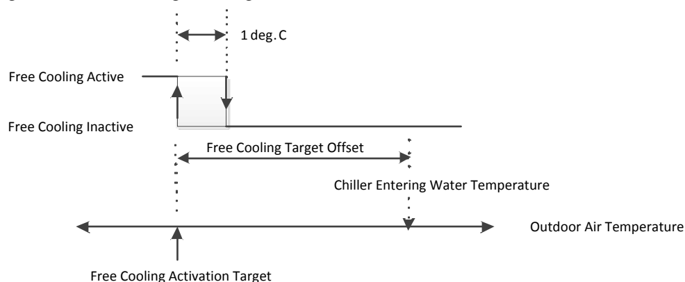
Figure 12 – Free-cooling enabling conditions
