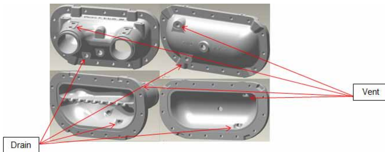
Figure 6 – Drain and vent position on evaporator
