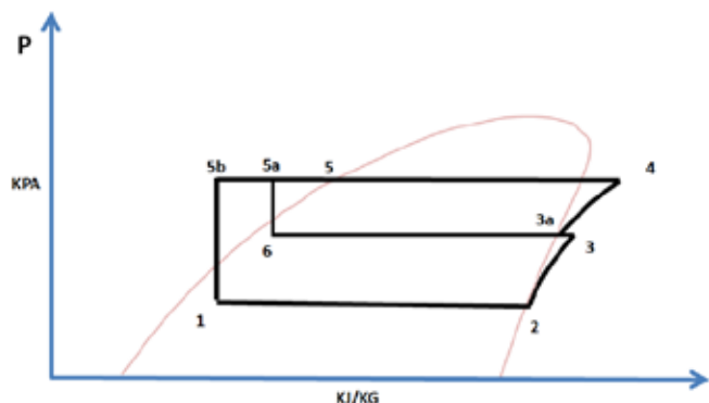
Figure 21 – Pressure enthalpy (P-h) diagram
