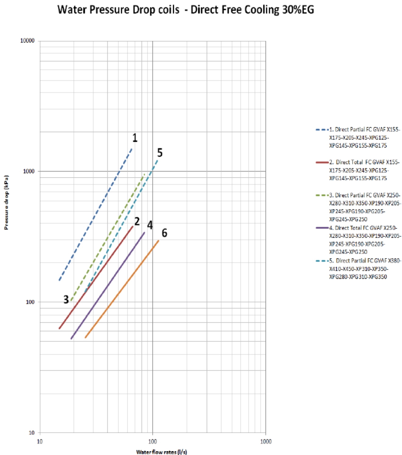
Figure 14 – Water Pressure drop coils - Total and Partial Direct Free cooling
