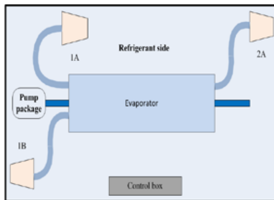
Figure 18 – 3 compressors unit
