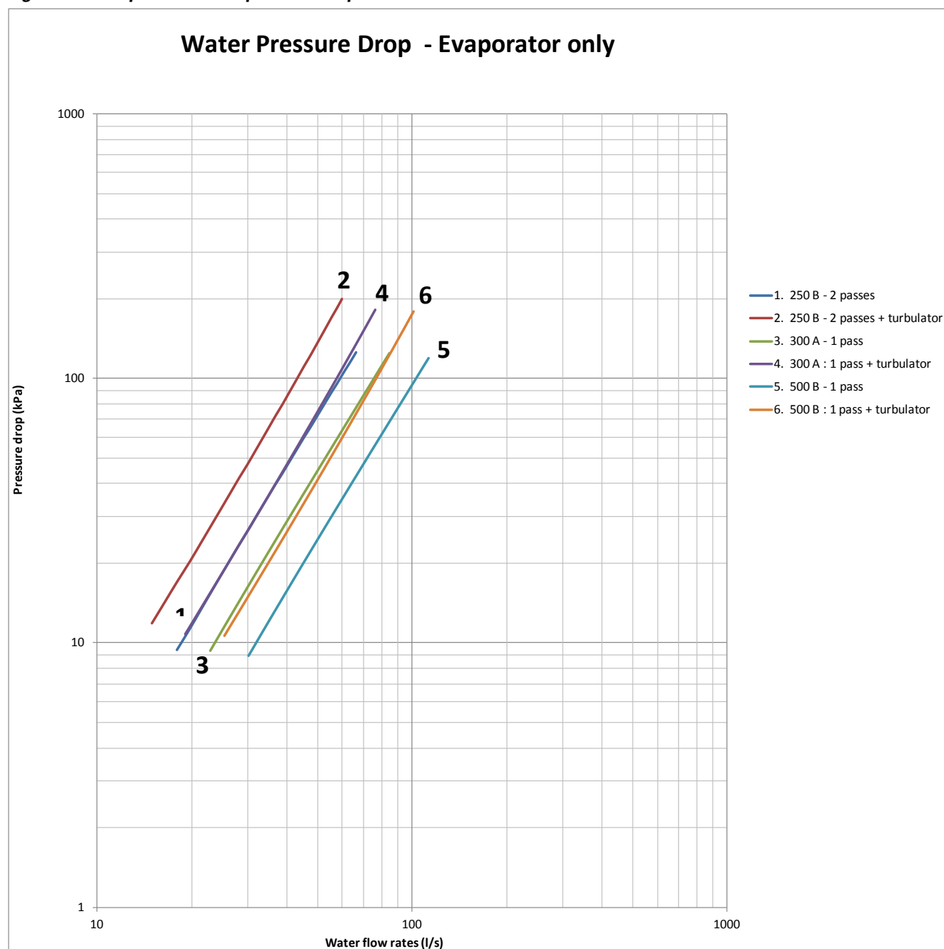
Figure 16 – Evaporator water pressure drop
