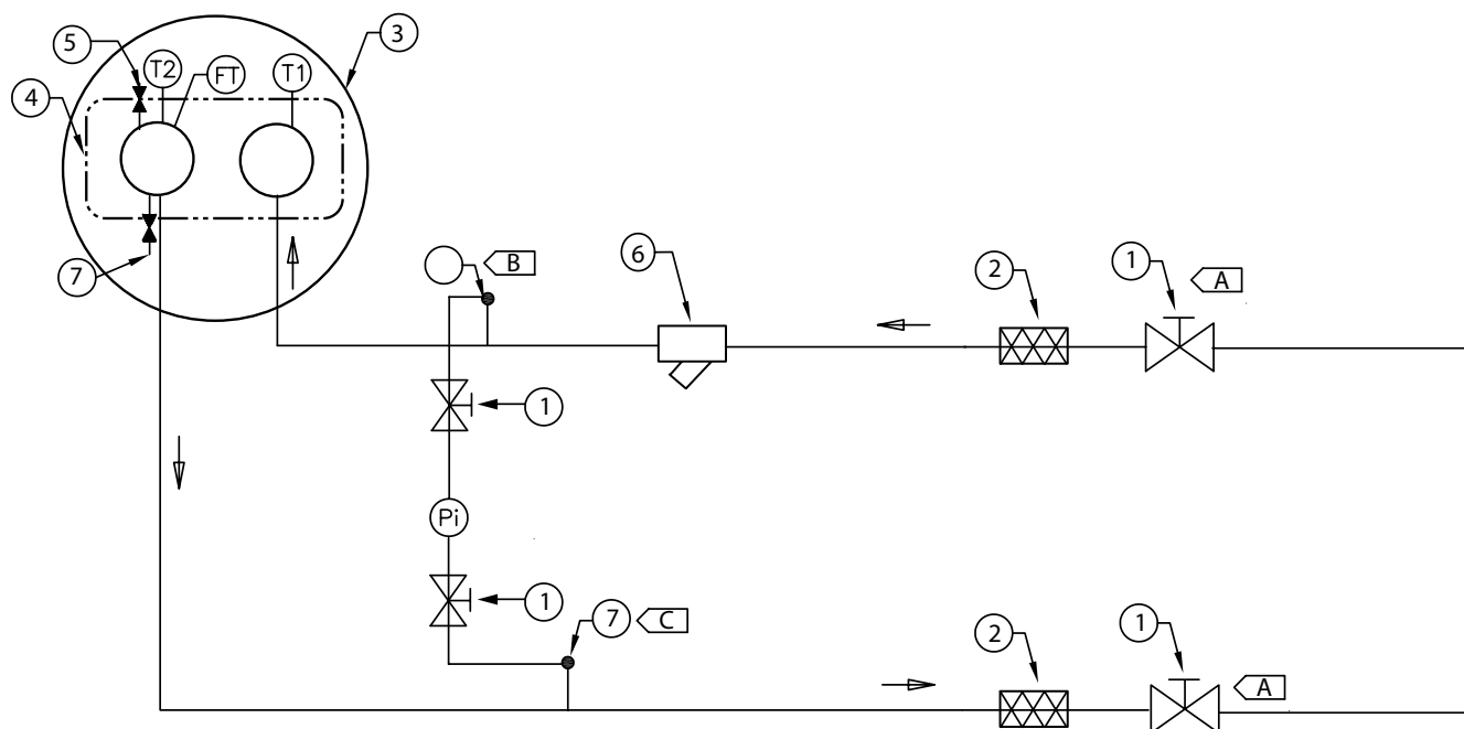
Figure 5 – Typical GVAF evaporator water piping
