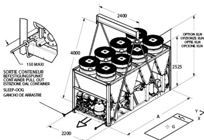
Figure 1b – Lifting
