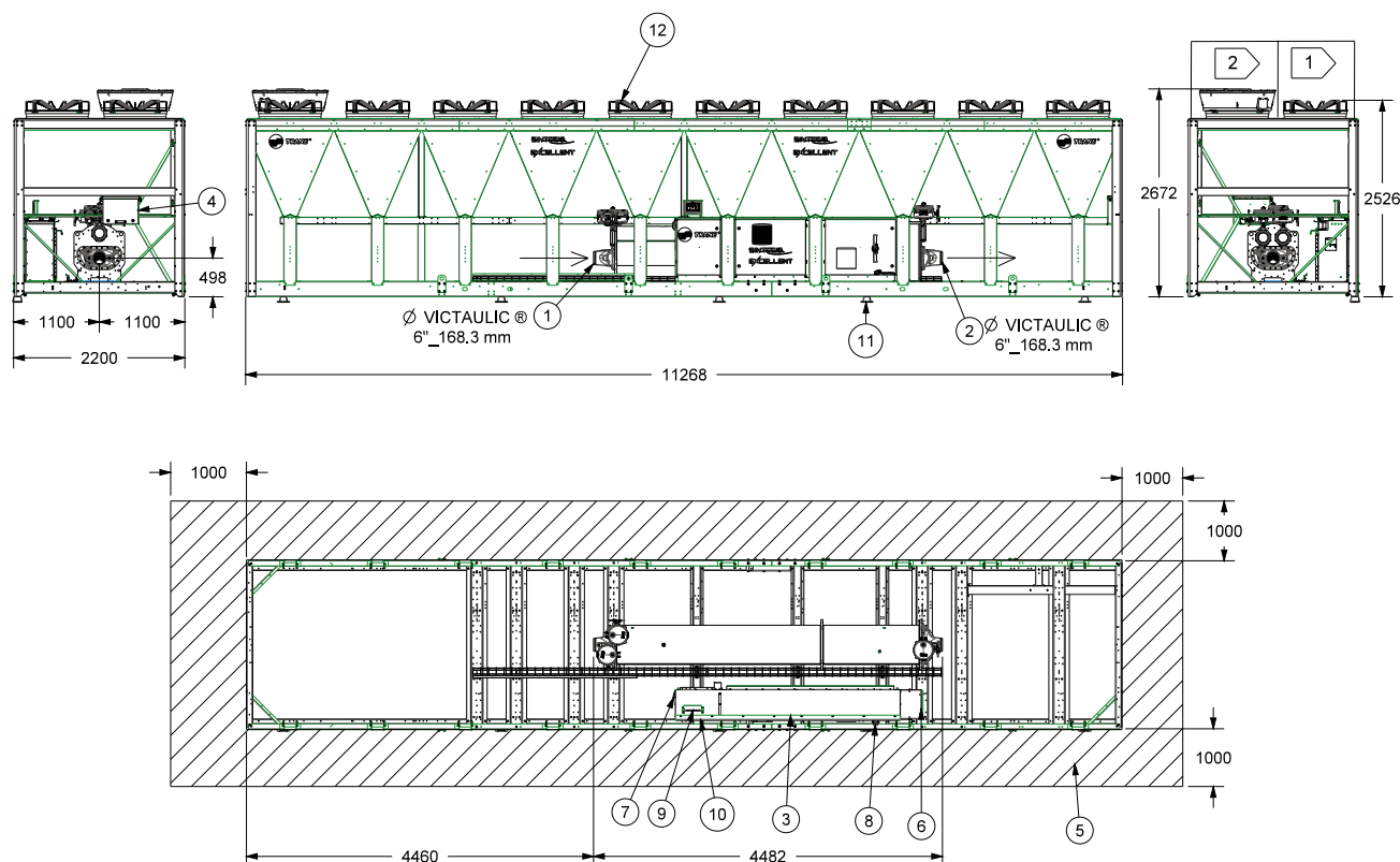
Figure 4 – Typical submittal example: GVAF 250X-350X / GVAF 190XP-245XP / GVAF 190XPG-250XPG
