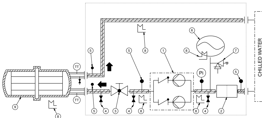
Figure 9 – Hydraulic module water chart
