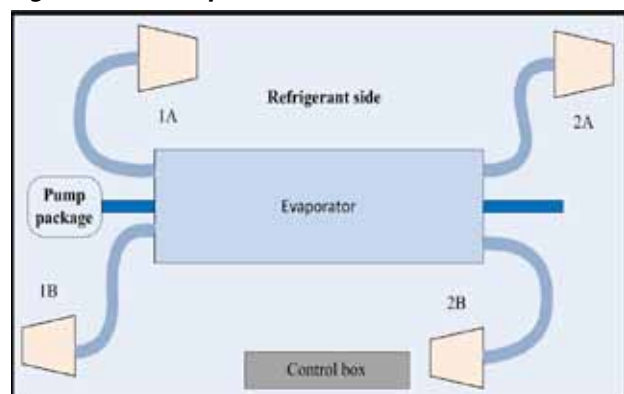
Figure 19 – 4 compressors unit
