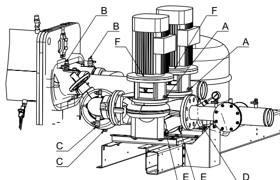
Figure 22 – Pump Package
