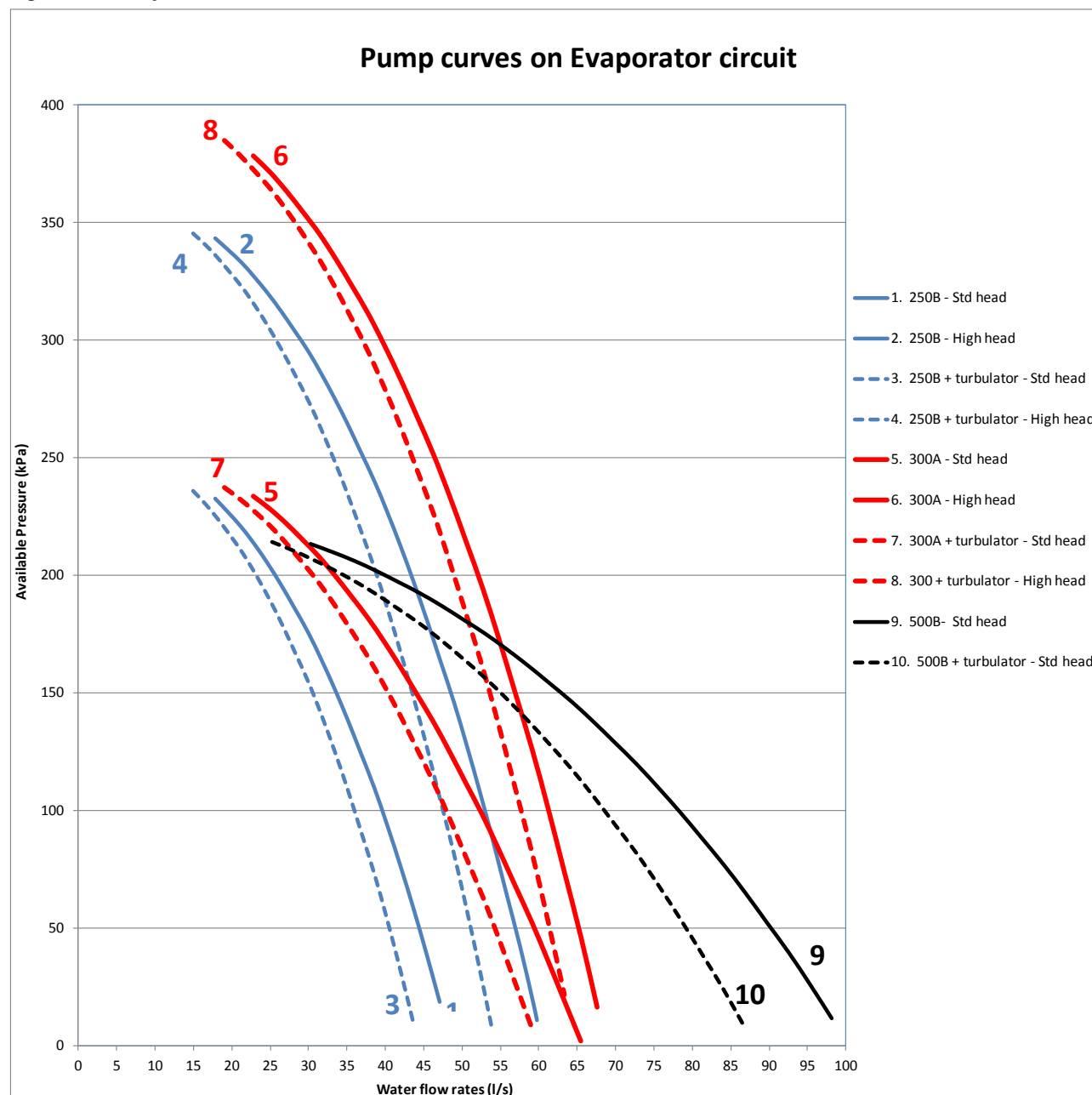
Figure 8 – Pump Curve
