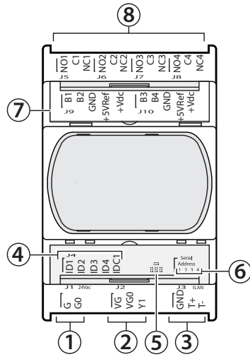
Figure 3 – CH535 extension terminal locations
