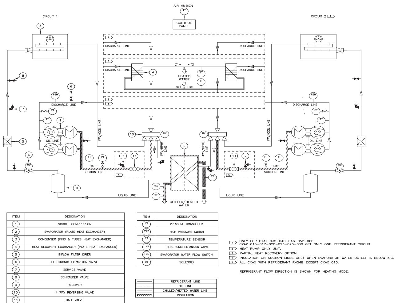
Figure 10a - Example of Typical Refrigerant System Schematic of duplex heat pump unit
