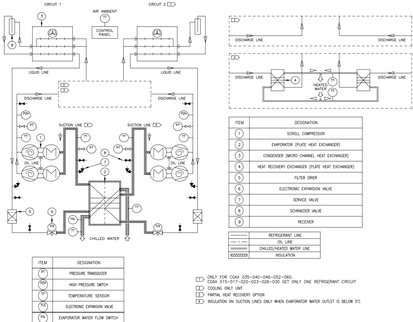
Figure 9a - Example of Typical Refrigerant System Schematic of duplex cooling only unit
