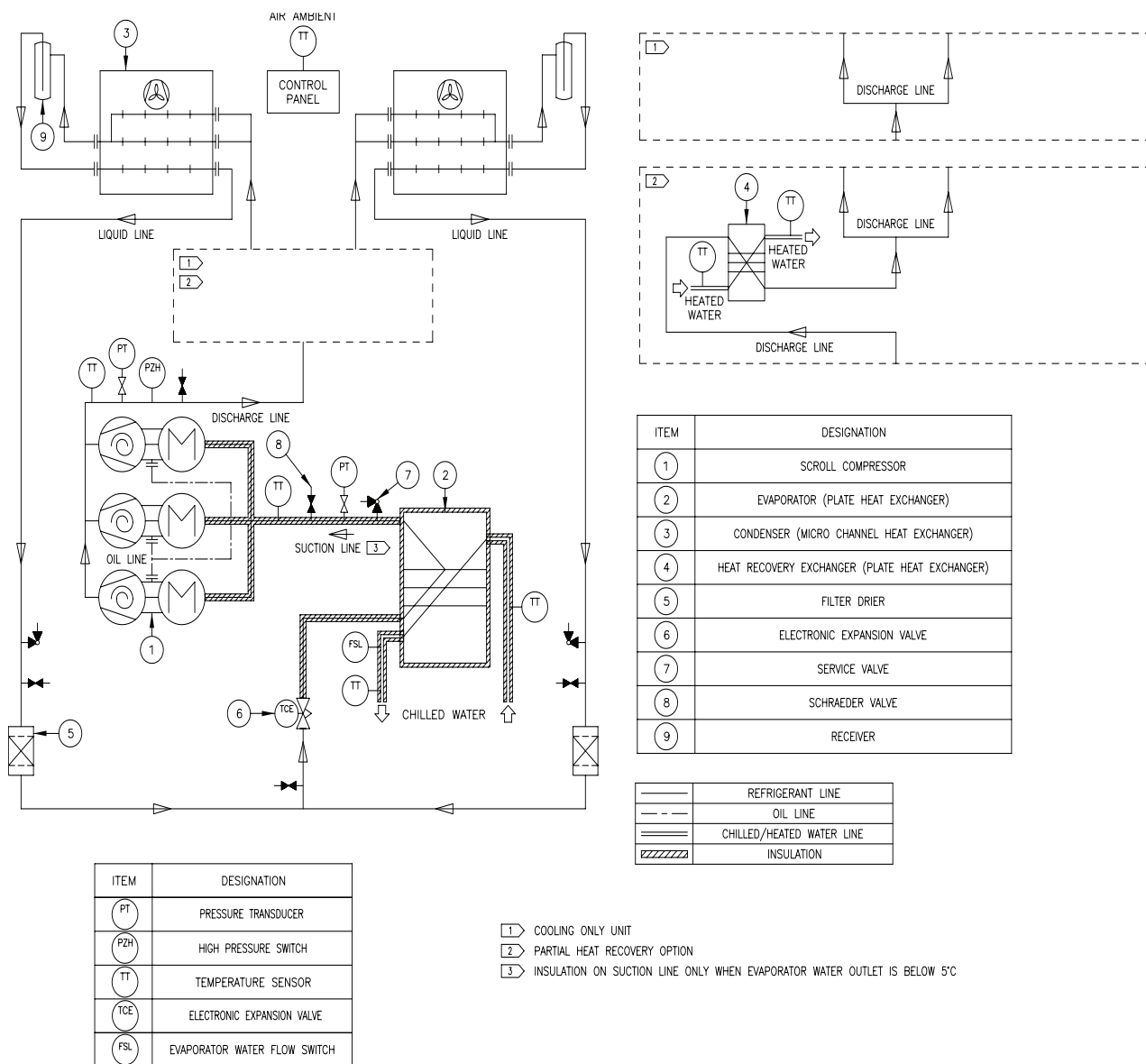
Figure 9b - Example of Typical Refrigerant System Schematic of simplex large trio cooling only unit
