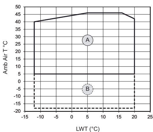
Figure 6 - Operating map- Cooling-only CGAX
