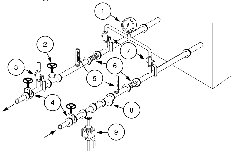
Figure 3 - Unit typical water circuit
