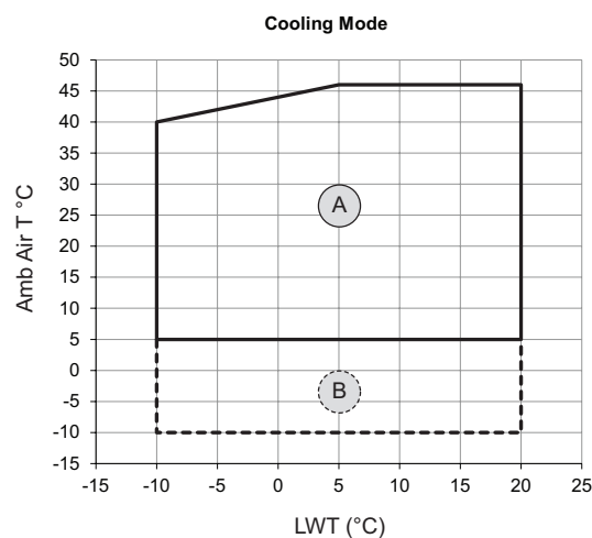
Figure 7 - Heat Pump CXAX operating map
