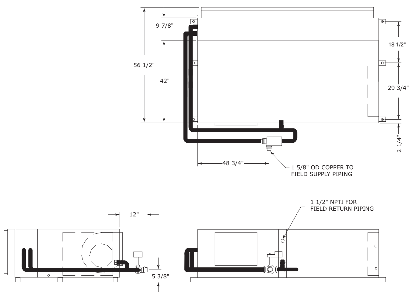
Figure 40. GEH 12.5 to 15 tons (60 Hz), GEH 10 to 12.5 tons (50 Hz), right return with waterside economizer (a)
