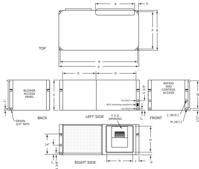
Figure 11. Right return/right supply (GEH/EXH)
