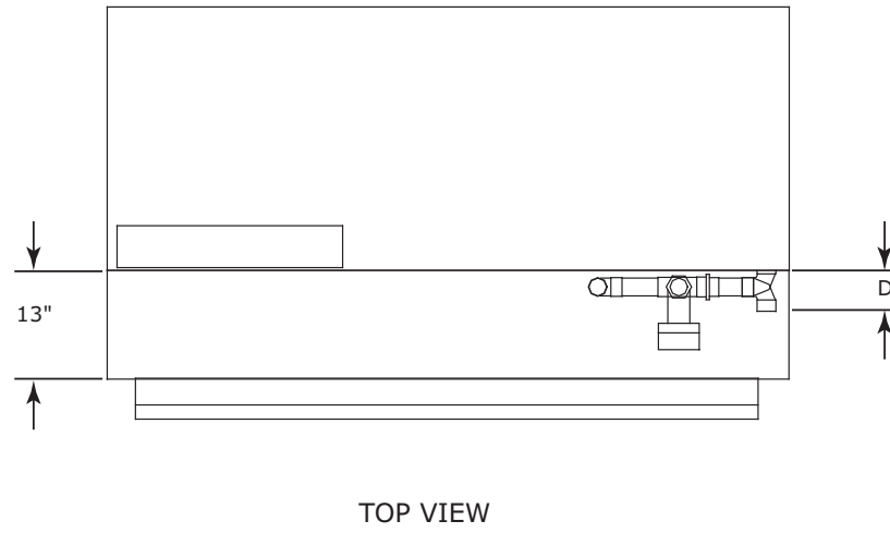
Figure 43. GEV 12.5 to 25 tons - waterside economizer
