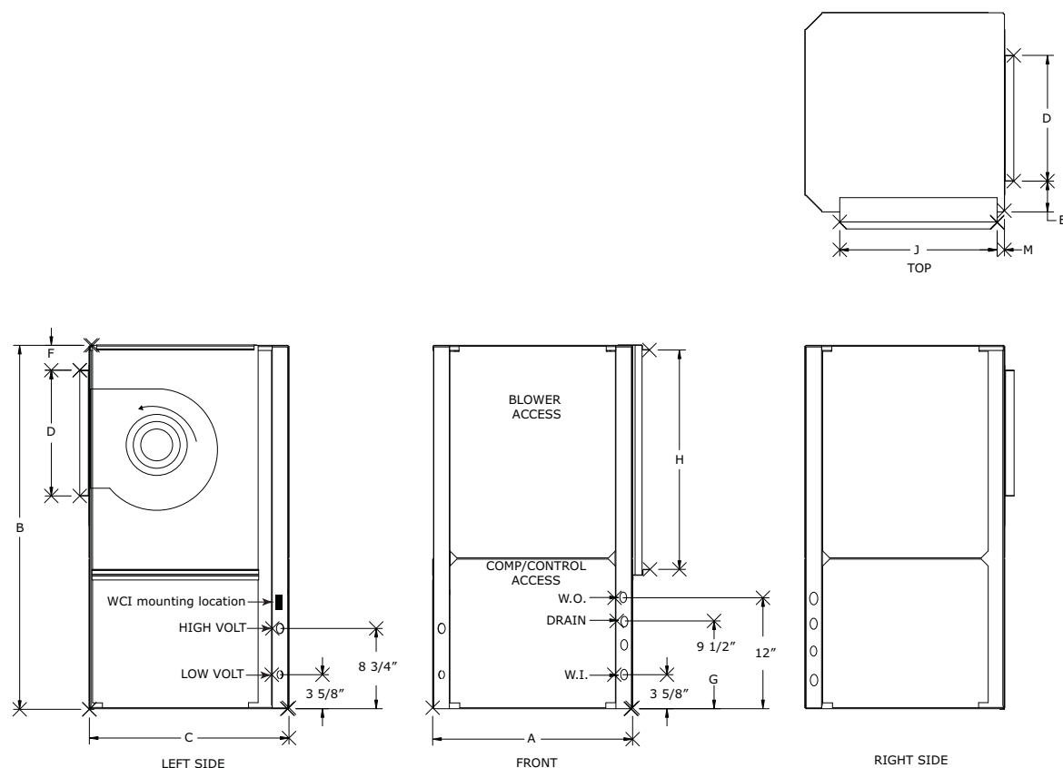
Figure 15. Right return/back supply (GEV/EXV)
