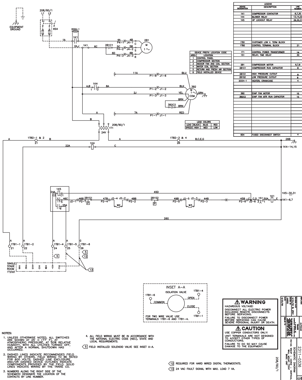
Figure 82. GEH_V (.5 to 5 tons) - basic-208V - 60 Hz - 1 ph(a)
