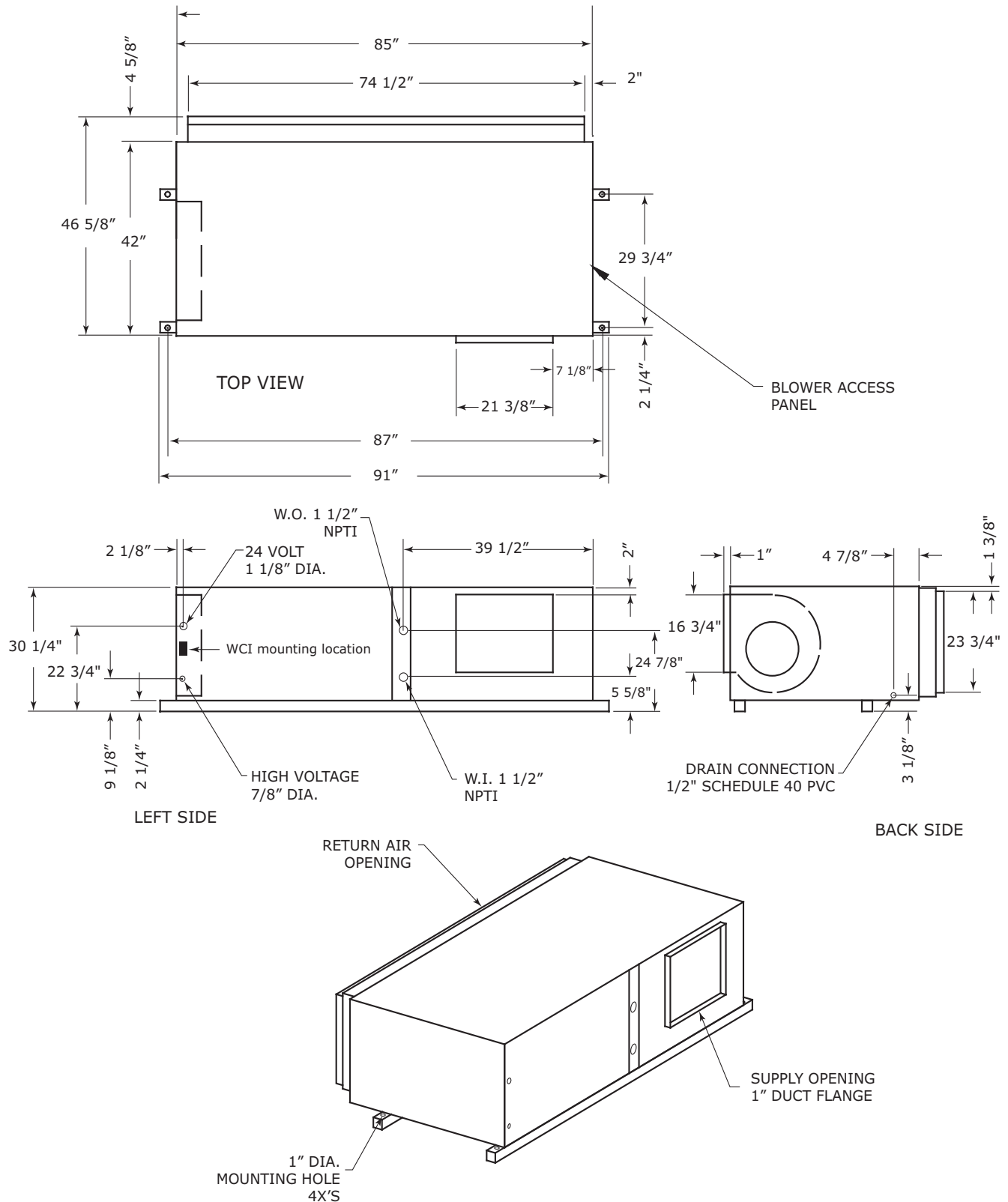
Figure 22. Left return/right supply GEH 12.5 to 15 tons (60 Hz); GEH 10 to 12.5 tons (50 Hz)
