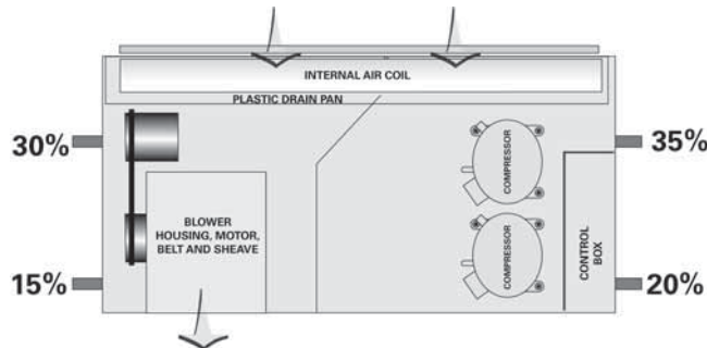
Figure 46. Weight distribution GEH 6 to 15 tons
