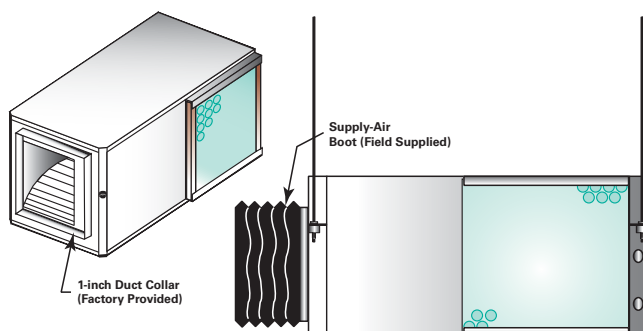
Figure 47. Flexible supply-air connector (field provided) GEH supply duct
