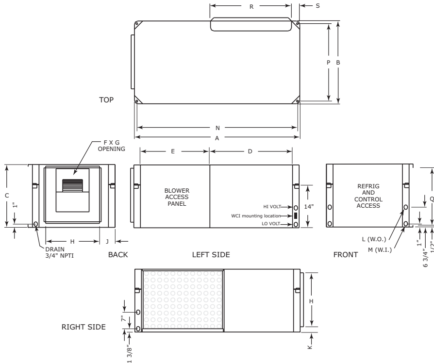
Figure 10. Right return/back supply (GEH/EXH)
