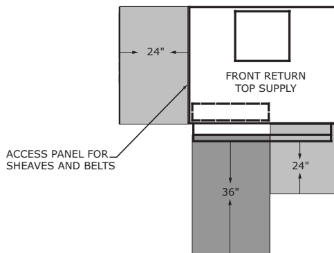
Figure 5. Clearance - GEV 12.5 to 25 Tons
