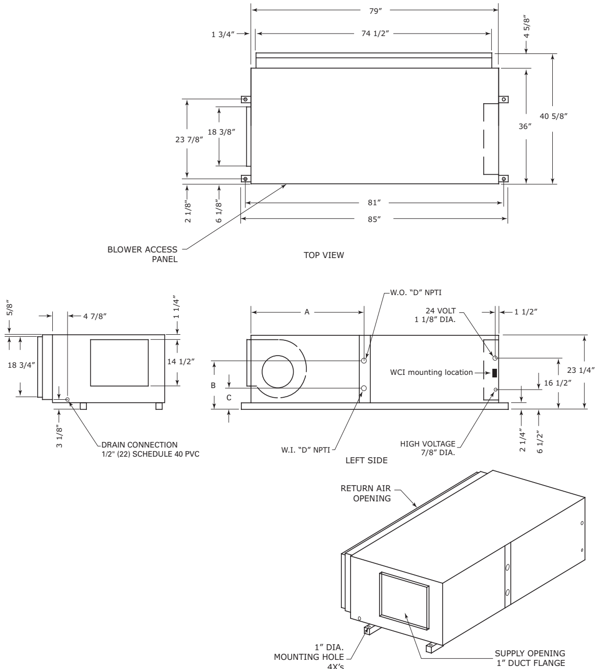
Figure 17. Right return/back supply - GEH 6 to 10 tons (60 Hz); GEH 6 to 7.5 tons (50 Hz)
