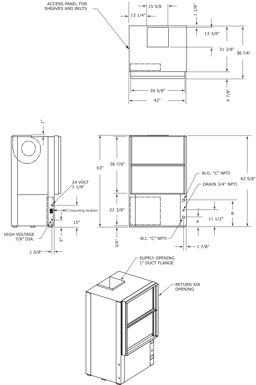
Figure 25. Front return/top supply (a) GEV 6 to 10 tons (60 Hz); 6 and 7.5 tons (50 Hz)
