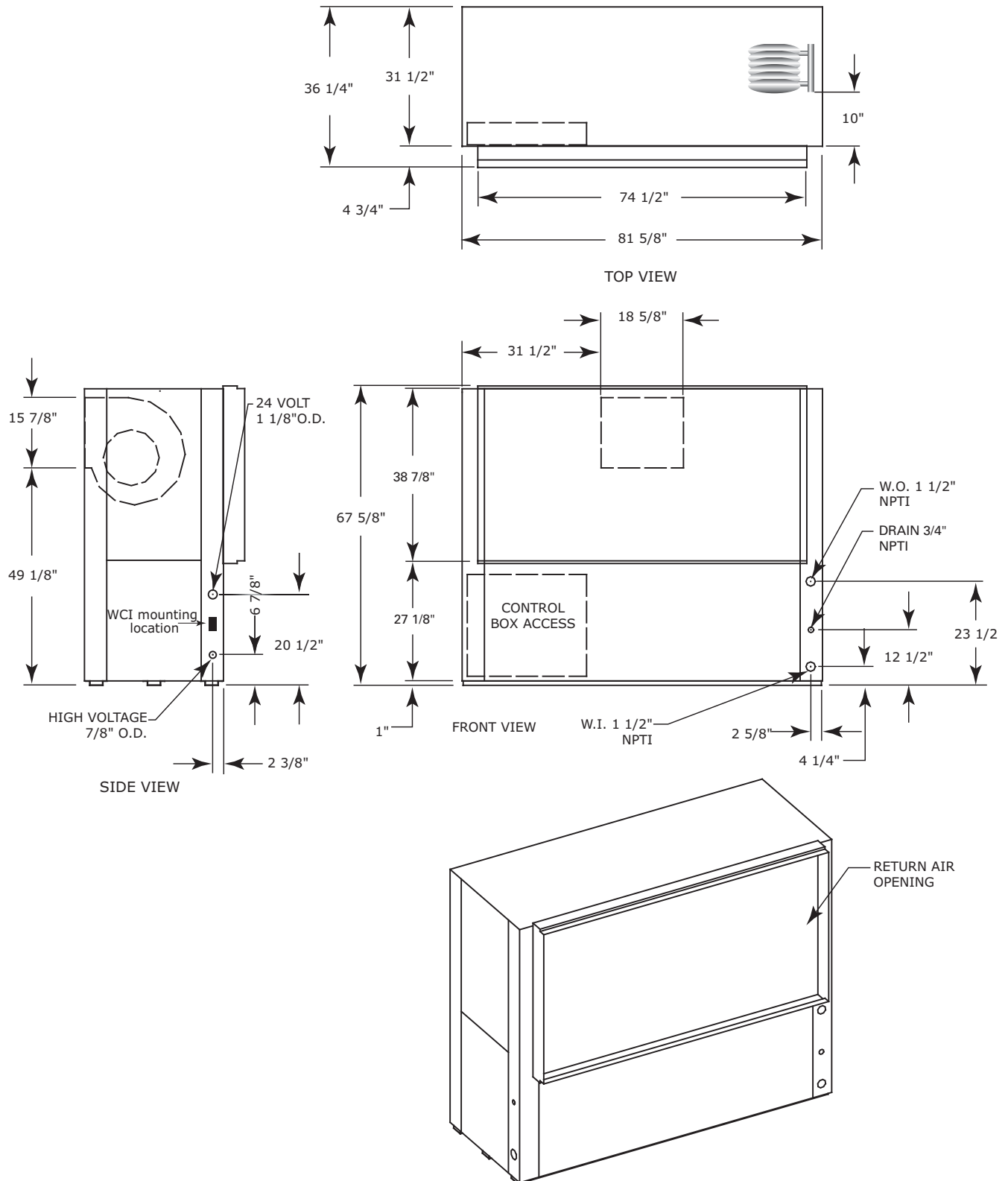
Figure 28. Front return/back supply (a) GEV 12.5 to 15 tons (60 Hz); GEV 10 and 12.5 ton (50 Hz)
