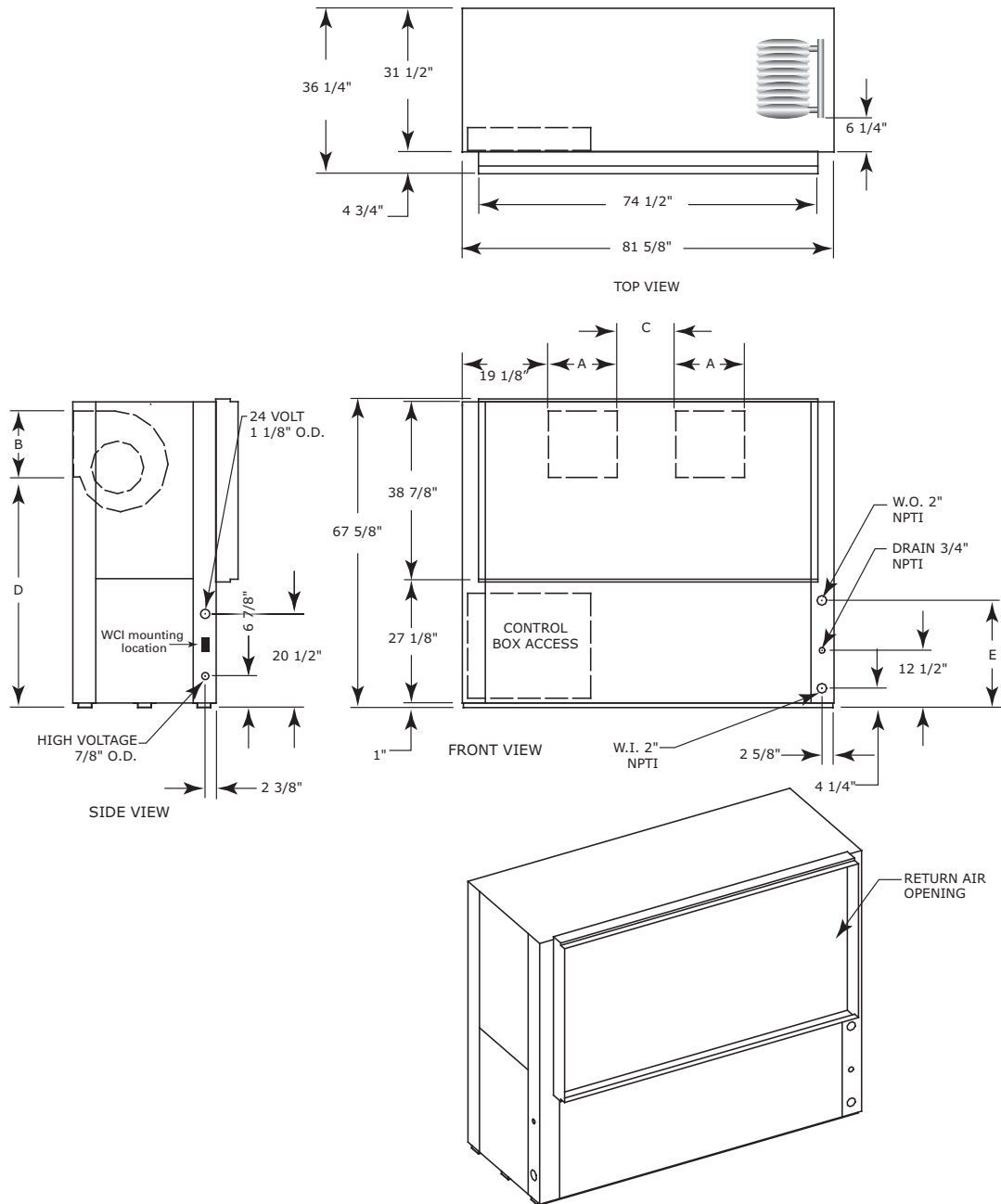
Figure 32. Front return/back supply (a) GEV 20 and 25 ton (60 Hz); GEV 15 and 20 ton (50 Hz)
