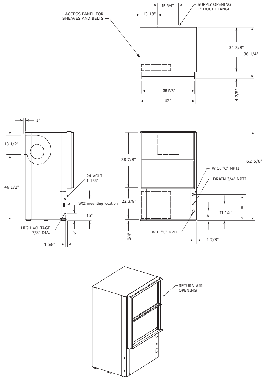
Figure 24. Front return/back supply (a) GEV 6 to 10 tons (60 Hz); 6 and 7.5 tons (50 Hz)
