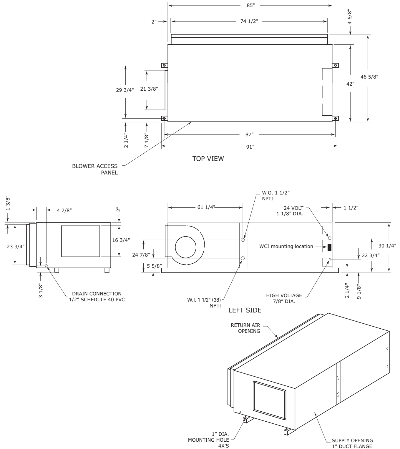
Figure 21. Right return/back supply GEH 12.5 to 15 tons (60 Hz); GEH 10 to 12.5 tons (50 Hz)
