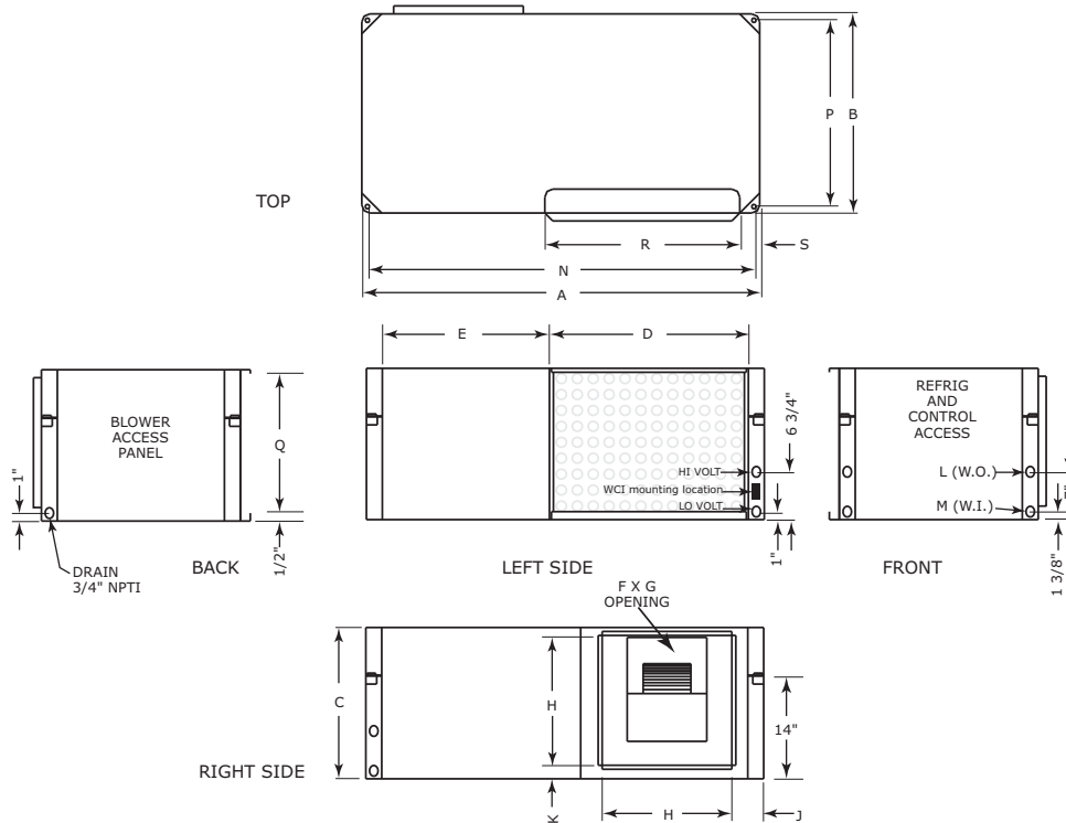
Figure 8. Left return/right supply (GEH/EXH)
