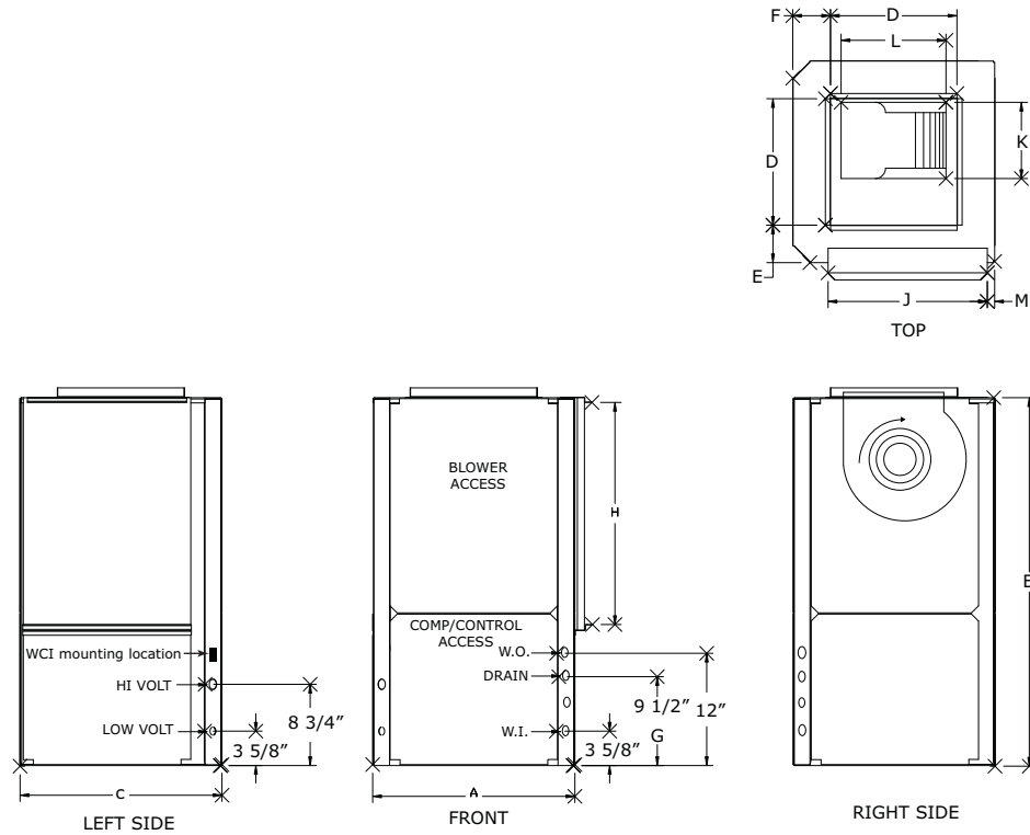
Figure 14. Right return/top supply (GEV/EXV)
