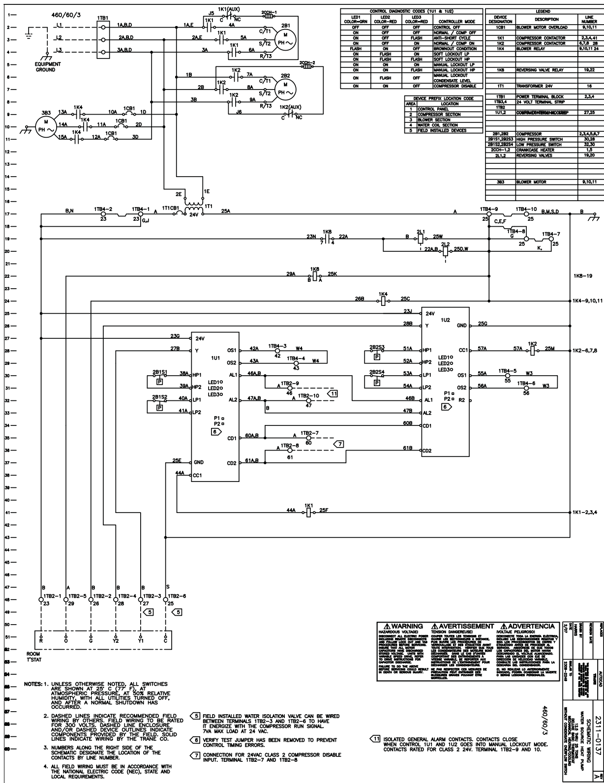
Figure 86. GEH_V (6-25 tons) - deluxe 24V - 460V-60 Hz - 3 ph(a)
