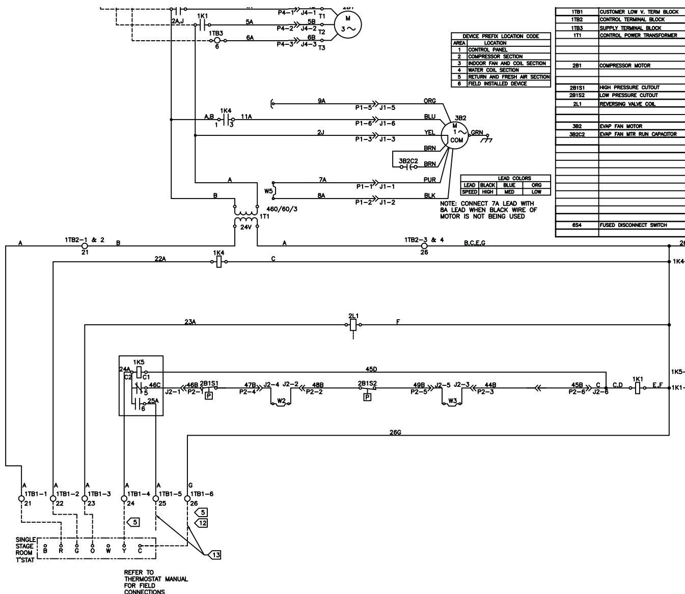
Figure 84. GEH_V (.5 to 5 tons) - basic 24V - 460V-60 Hz - 3 ph(a)
