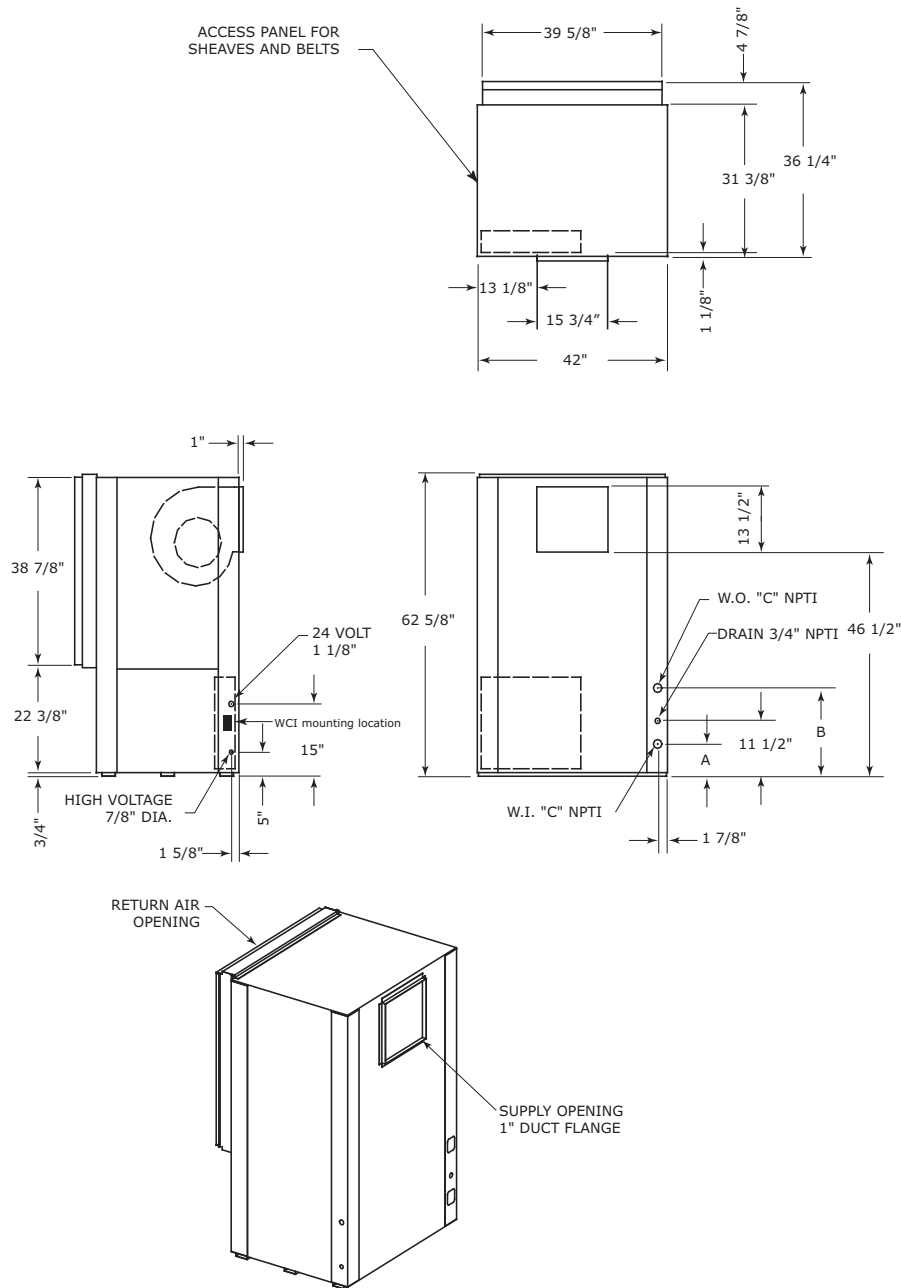
Figure 26. Back return/front supply (a) GEV 6 to 10 tons (60 Hz); 6 and 7.5 ton (50 Hz)
