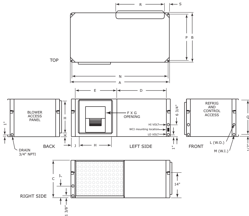
Figure 9. Right return/left supply (GEH/EXH)
