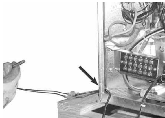
Figure 73. Step 8
