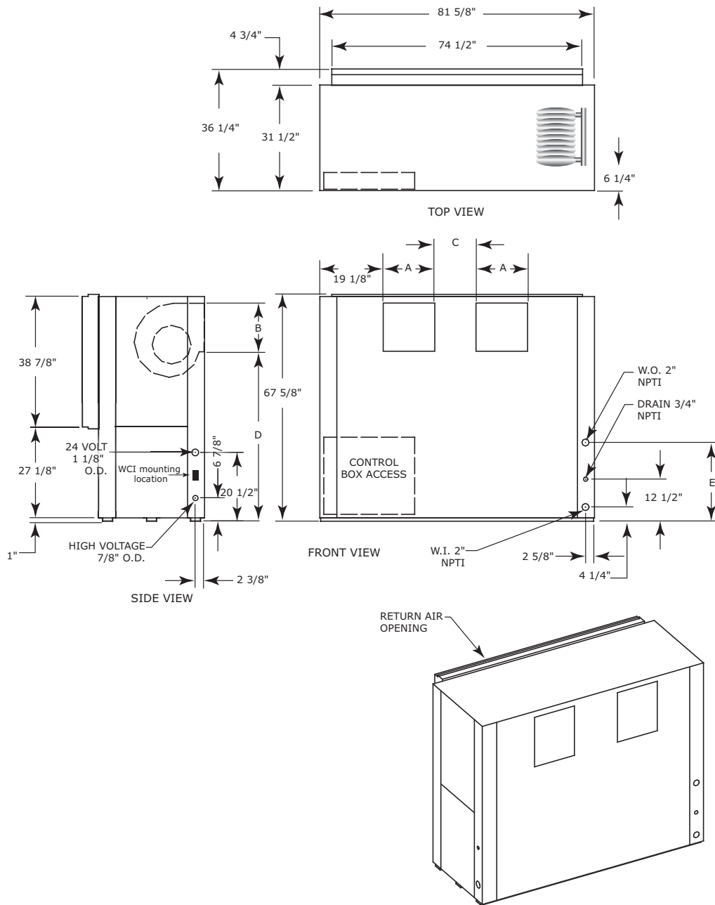
Figure 33. Back return/front supply (a) GEV 20 and 25 ton (60 Hz); GEV 15 and 20 ton (50 Hz)
