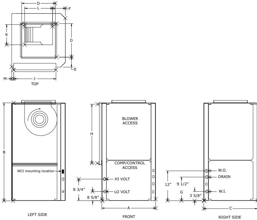
Figure 12. Left return/top supply (GEV/EXV)
