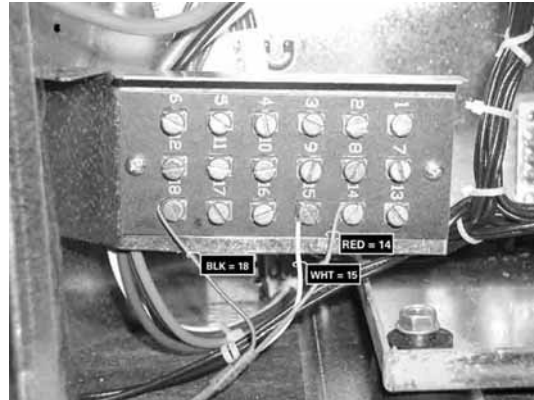
Figure 77. Step 12
