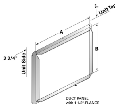
Figure 49. Return-air duct panel
