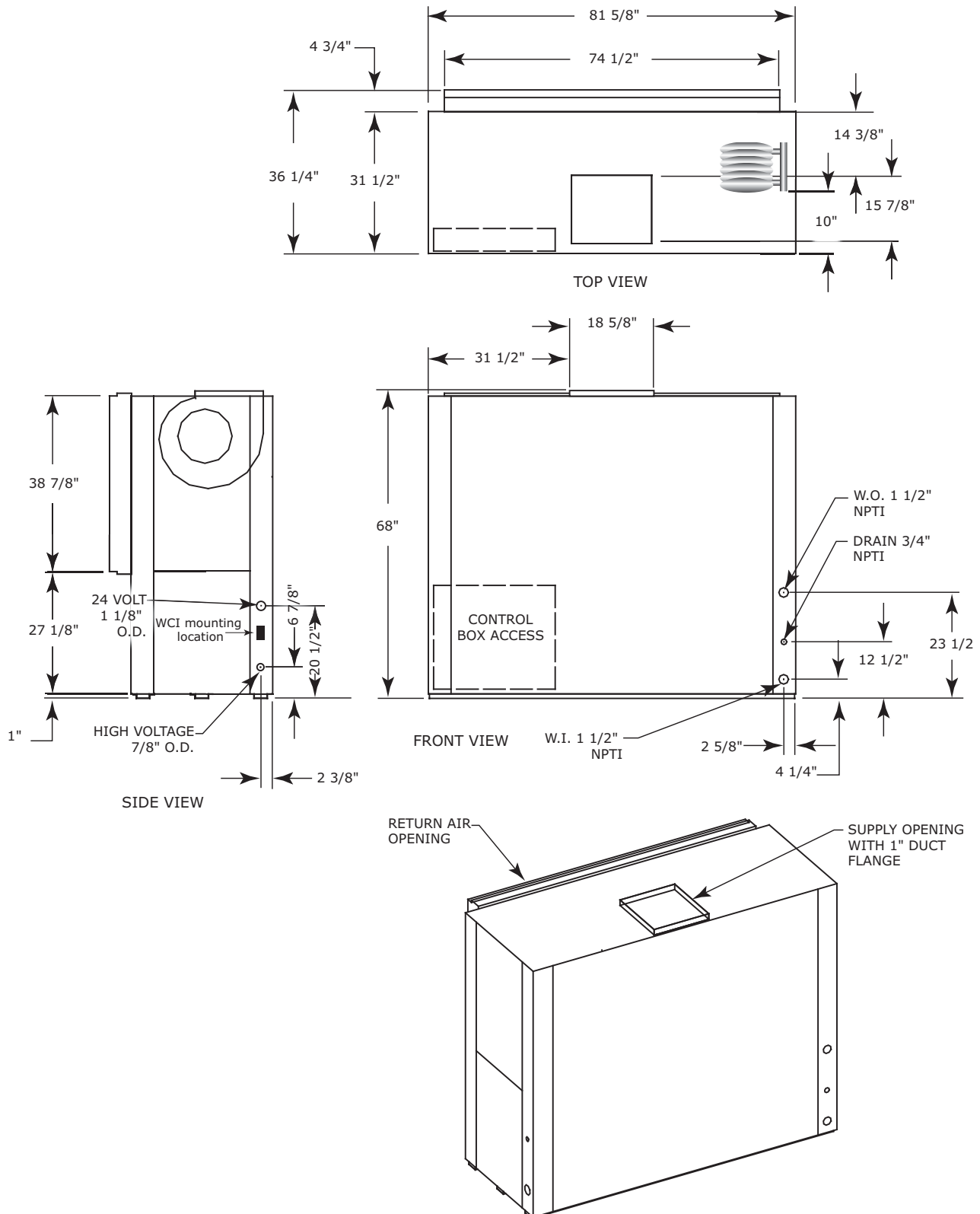
Figure 31. Back return/top supply (a) GEV 12.5 to 15 ton (60 Hz); GEV 10 and 12.5 ton (50 Hz)
