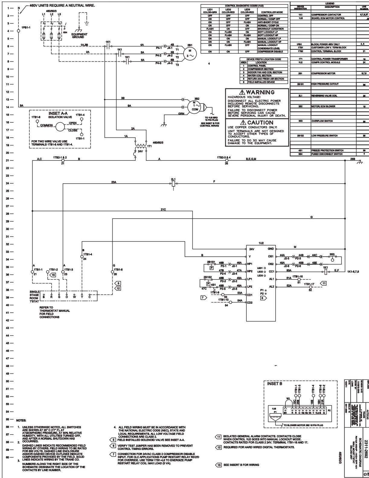
Figure 87. EXH/EXV - deluxe 24V - 460V-60 Hz - 3 ph (a) - (ECM motor wiring diagram)
