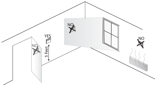
Figure 58. Thermostat/sensor location
