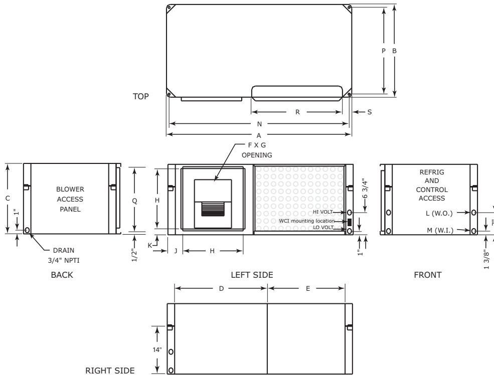
Figure 6. Left return/left supply (GEH/EXH)
