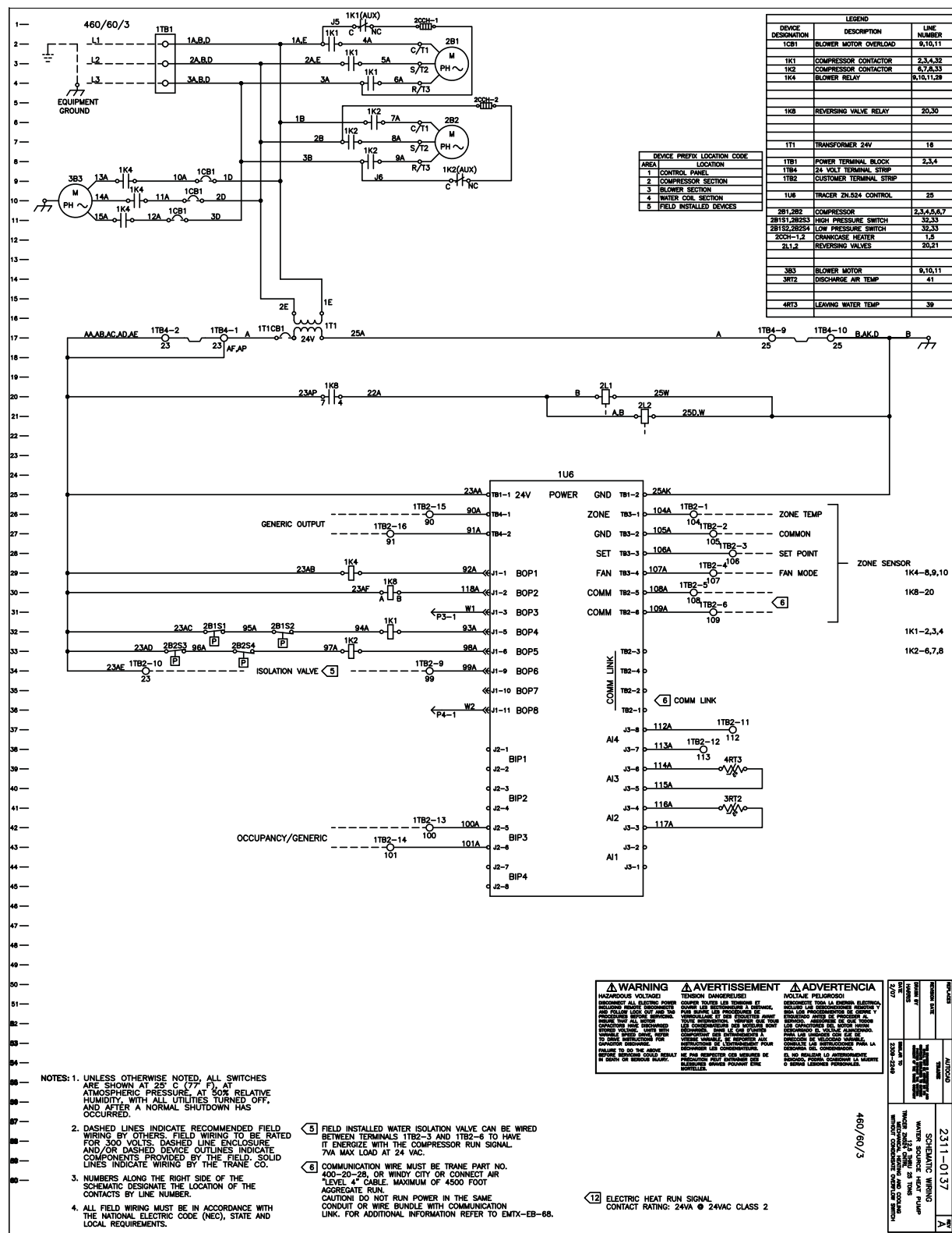
Figure 88. GEH_V (6 to 25 tons) - Tracer® ZN524-460V - 60 Hz - 3 ph (a)
