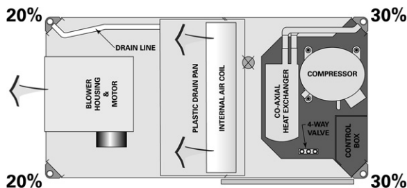
Figure 45. Weight distribution GEH .5 to 5 tons; EXH .5 to 6 tons
