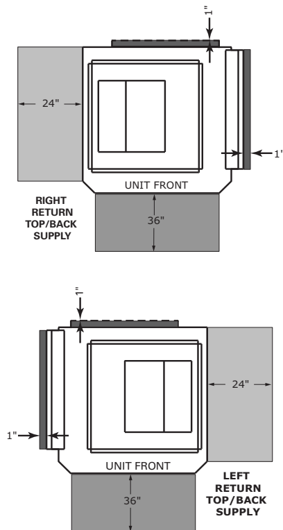
Figure 3. Clearance - GEV .5 to 5 tons & EXV .5 to 6 Tons
