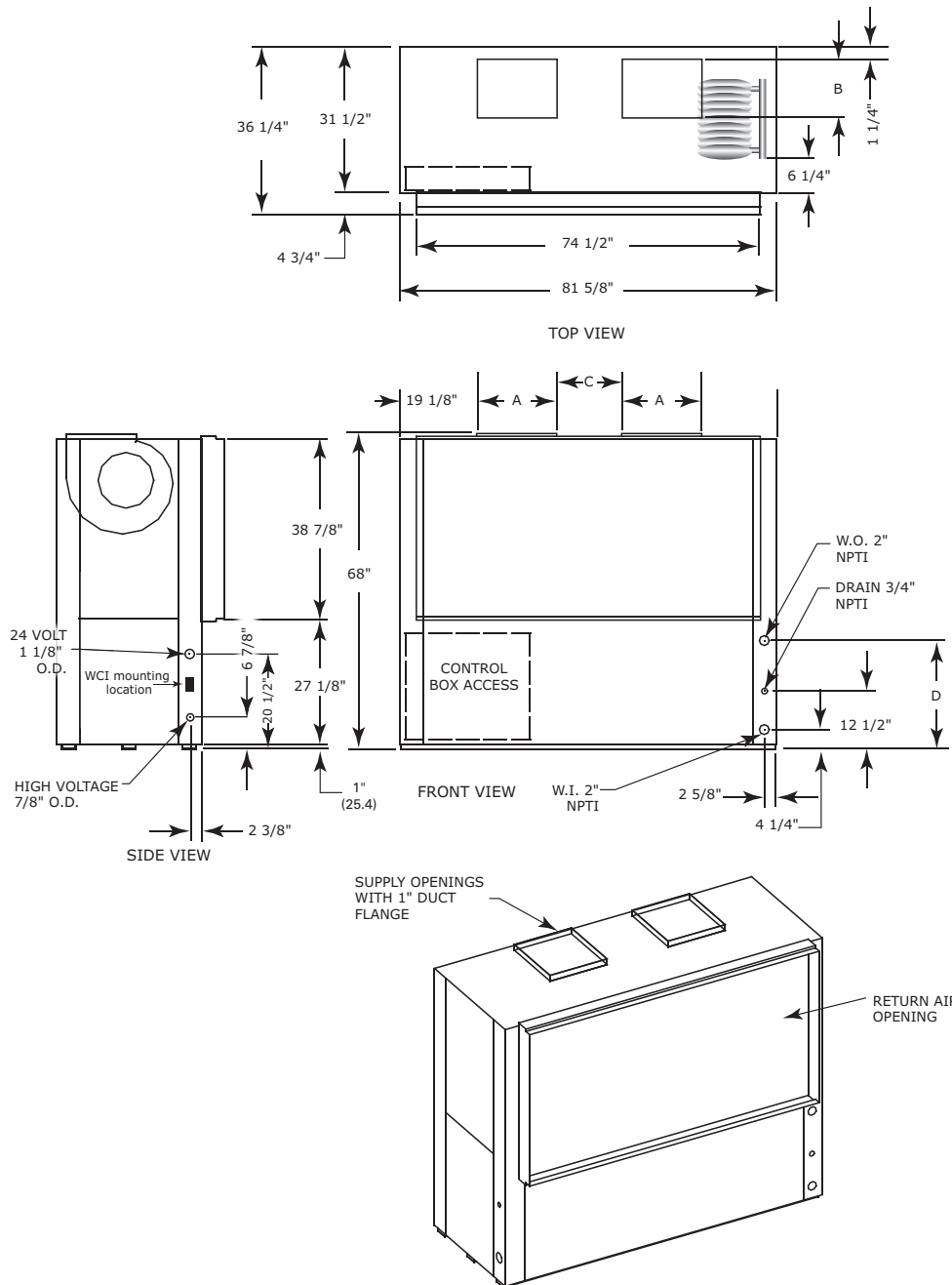
Figure 34. Front return/top supply (a) GEV 20 and 25 ton (60 Hz); GEV 15 and 20 ton (50 Hz)
