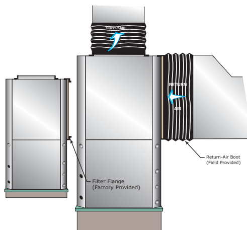
Figure 48. Flexible return-air connector (field provided) GEV return duct
