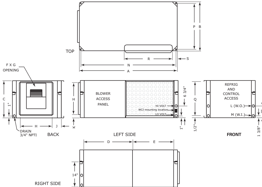
Figure 7. Left return/back supply (GEH/EXH)
