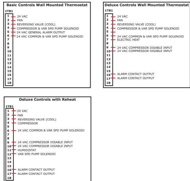
Figure 59. Low-voltage connection (GEH/V .5 to 5 ton and EXH/V (a) .5 to 6 ton equipment)
