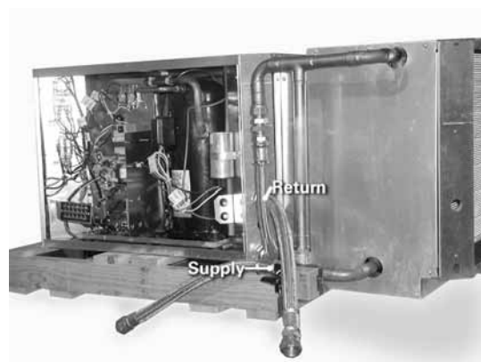
Figure 71. Step 6
