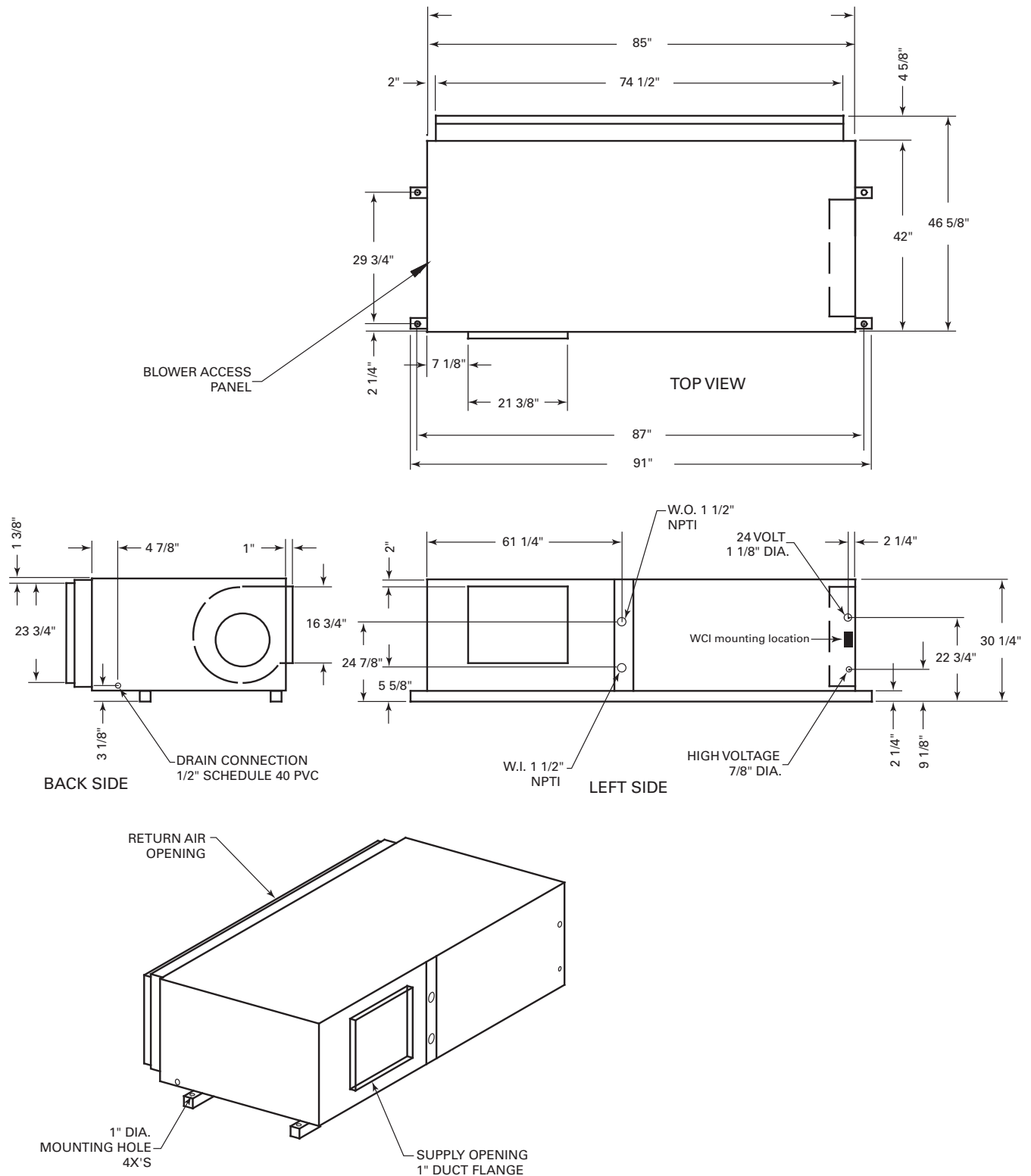
Figure 20. Right return/left supply GEH 12.5 to 15 tons (150-180) 60 Hz; GEH 10 to 12.5 tons (120-150) 50 Hz
