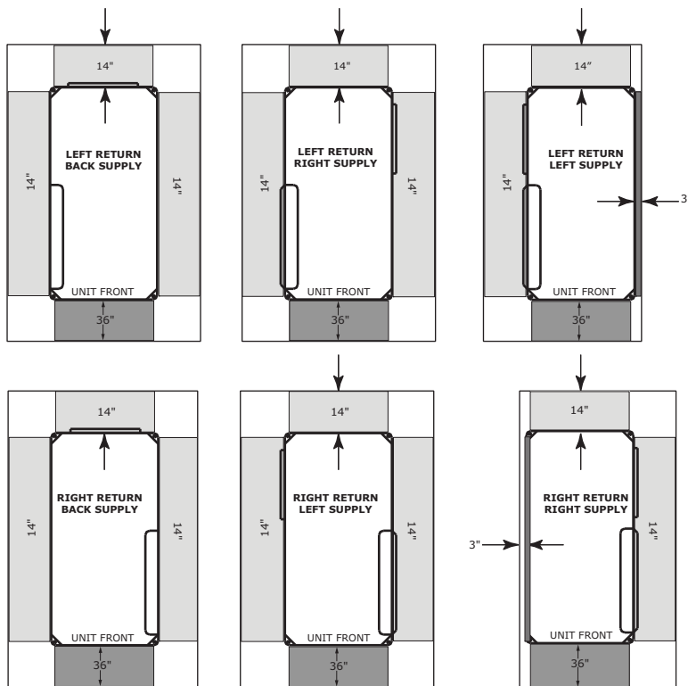
Figure 1. Clearances - GEH .5 to 5 tons & EXH .5 to 6 Tons
