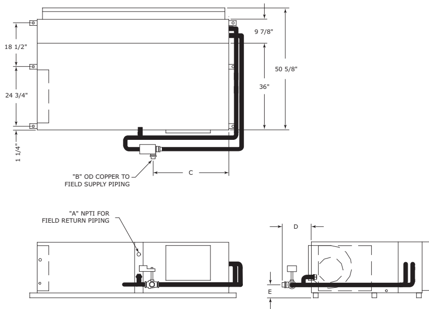
Figure 39. GEH 6 to 10 tons (60 Hz), GEH 6 to 7.5 tons (50 Hz) - left return with waterside economizer (a)
