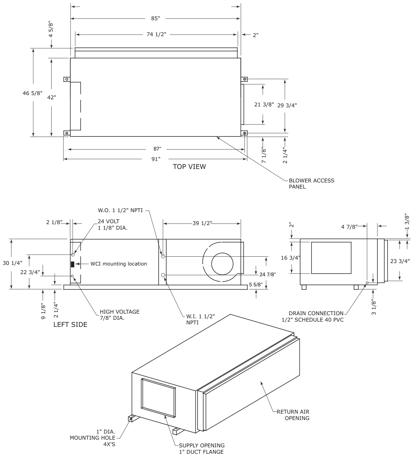
Figure 23. Left return/back supply GEH 12.5 to 15 tons (60 Hz); GEH 10 to 12.5 tons (50 Hz)
