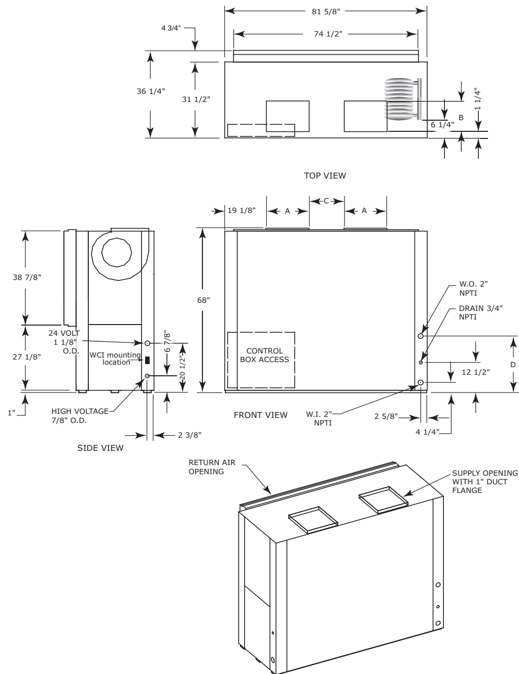
Figure 35. Back return/top supply (a) GEV 20 and 25 ton (60 Hz); GEV 15 and 20 ton (50 Hz)
