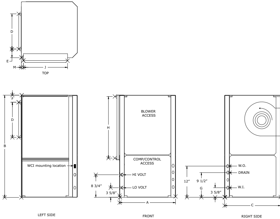
Figure 13. Left return/back supply (GEV/EXV)
