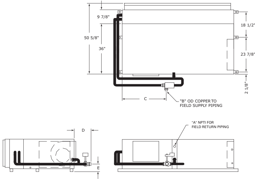
Figure 38. GEH 6 to 10 tons (60 Hz), GEH 6 to 7.5 tons (50 Hz) - right return with waterside economizer (a)
