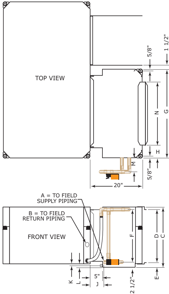
Figure 36. Waterside economizer (a) (GEH/EXH)
