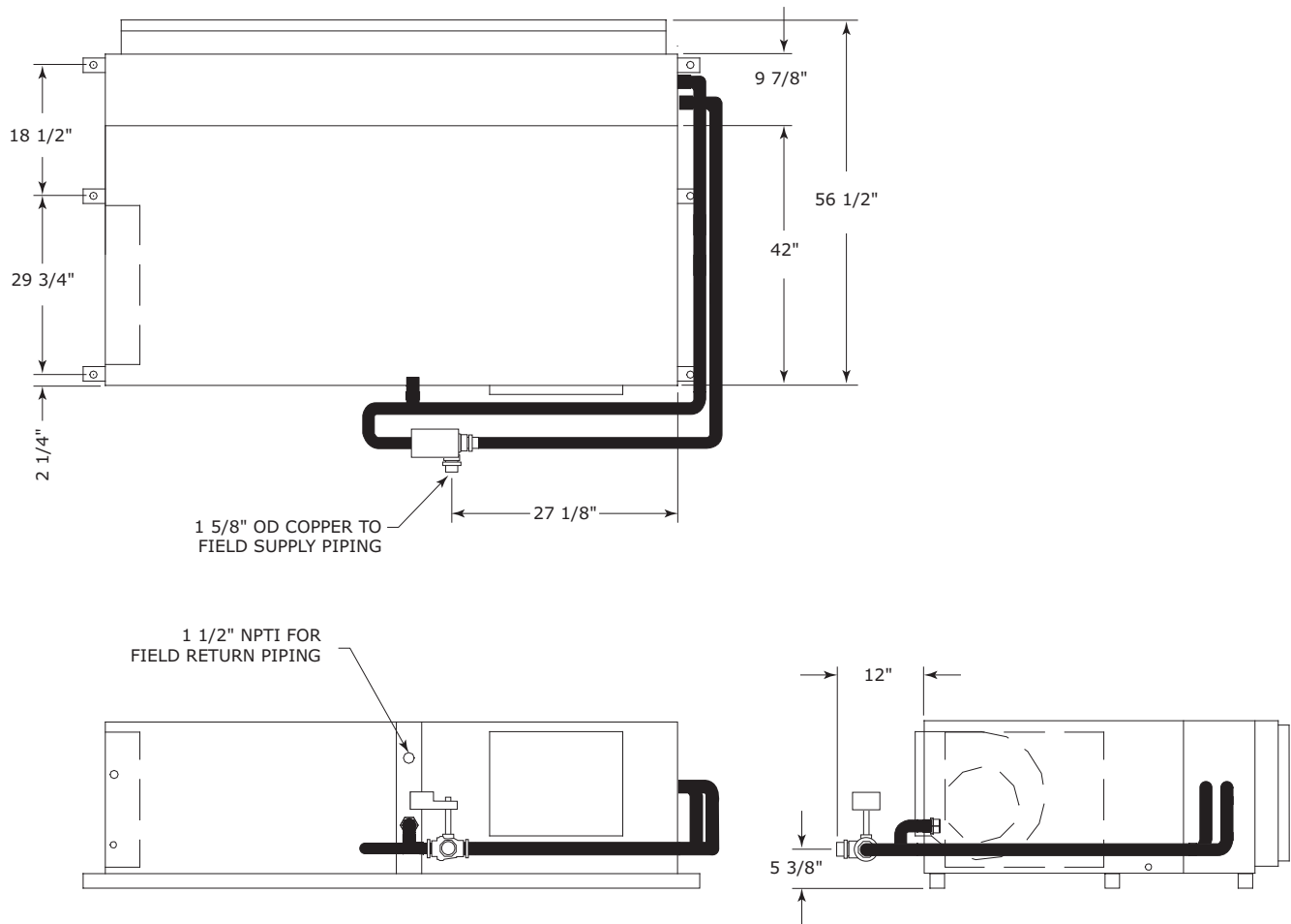
Figure 41. GEH 12.5 to 15 tons (60 Hz), GEH 10 to 12.5 tons (50 Hz), left return with waterside economizer (a)
