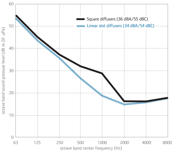
Figure 6. Effect of replacing square diffusers with linear slot diffusers
