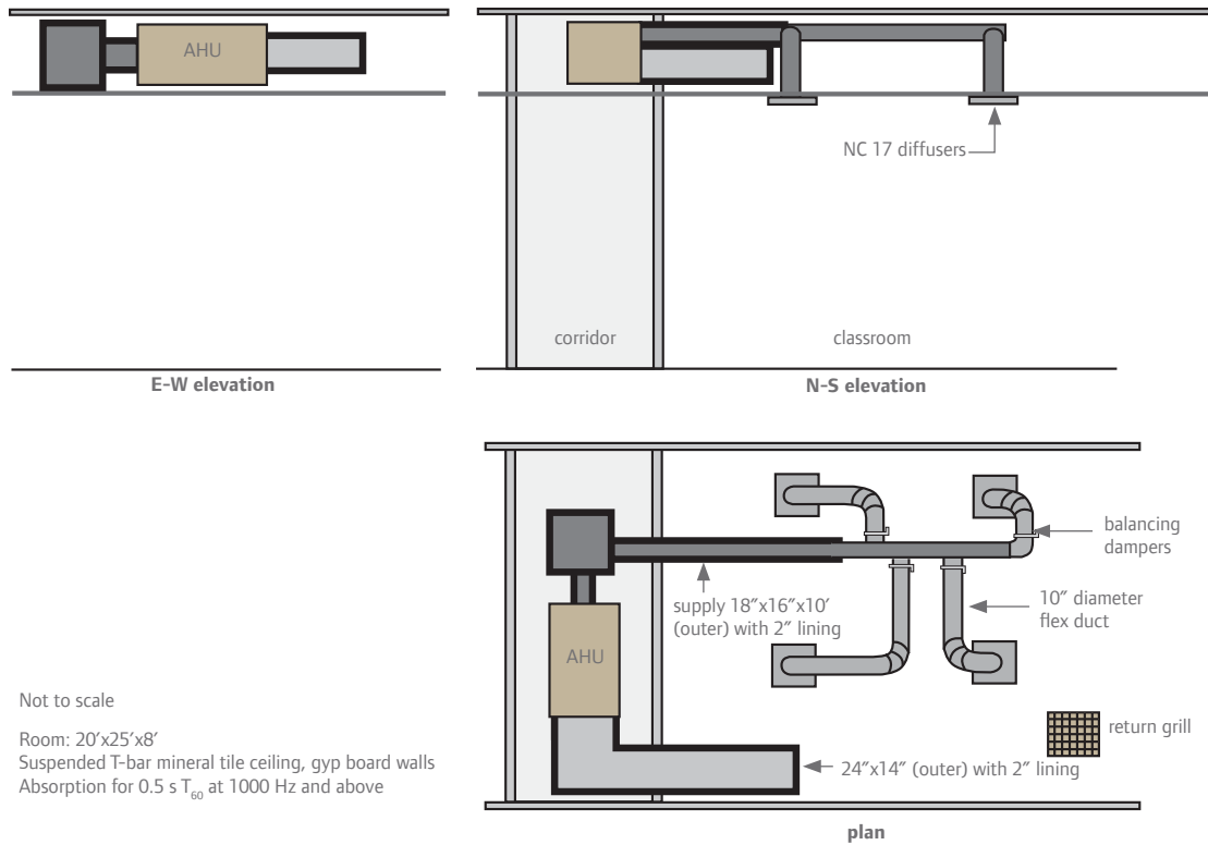
Figure 2. Mock-up classroom layout for zone-level air handler
