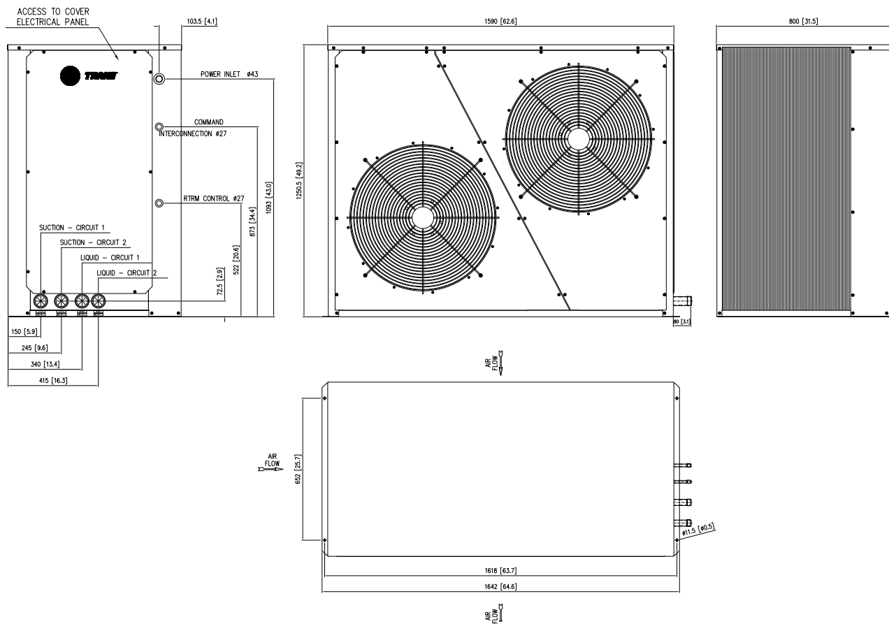
Fig. X-29 - Dimensions - Condensing Units TRAE 150 - 2 circuits
