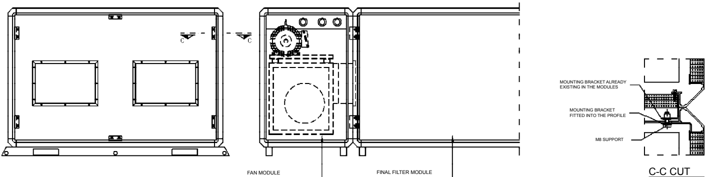
Fig. X-18 – Horizontal assembly with Final Filter
