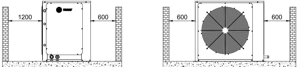
Fig. X 36 - Clearances required for Maintenance and Air Circulation - TRAE Suggestes clearances TRAE 050 to 150 - Horizontal Discharge
