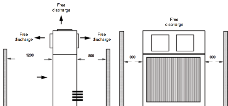
Fig. X 38 - Suggested Clearances for Maintenance and Air Circulation - Condensing Unit TRCE 050 to 150.
