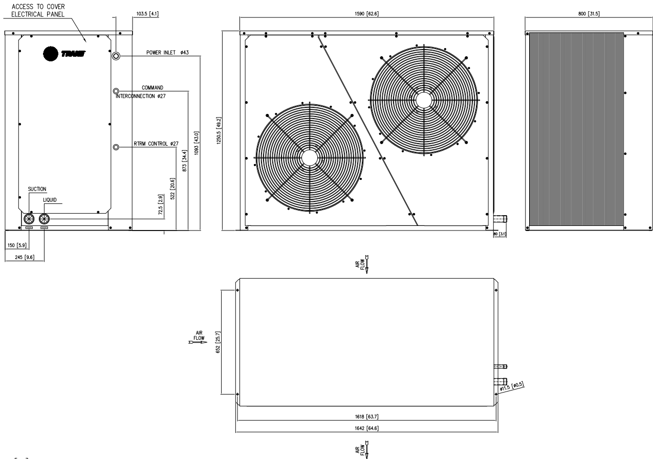
Fig. X-28 - Dimensions - Condensing Units TRAE 150 - 1 circuit
