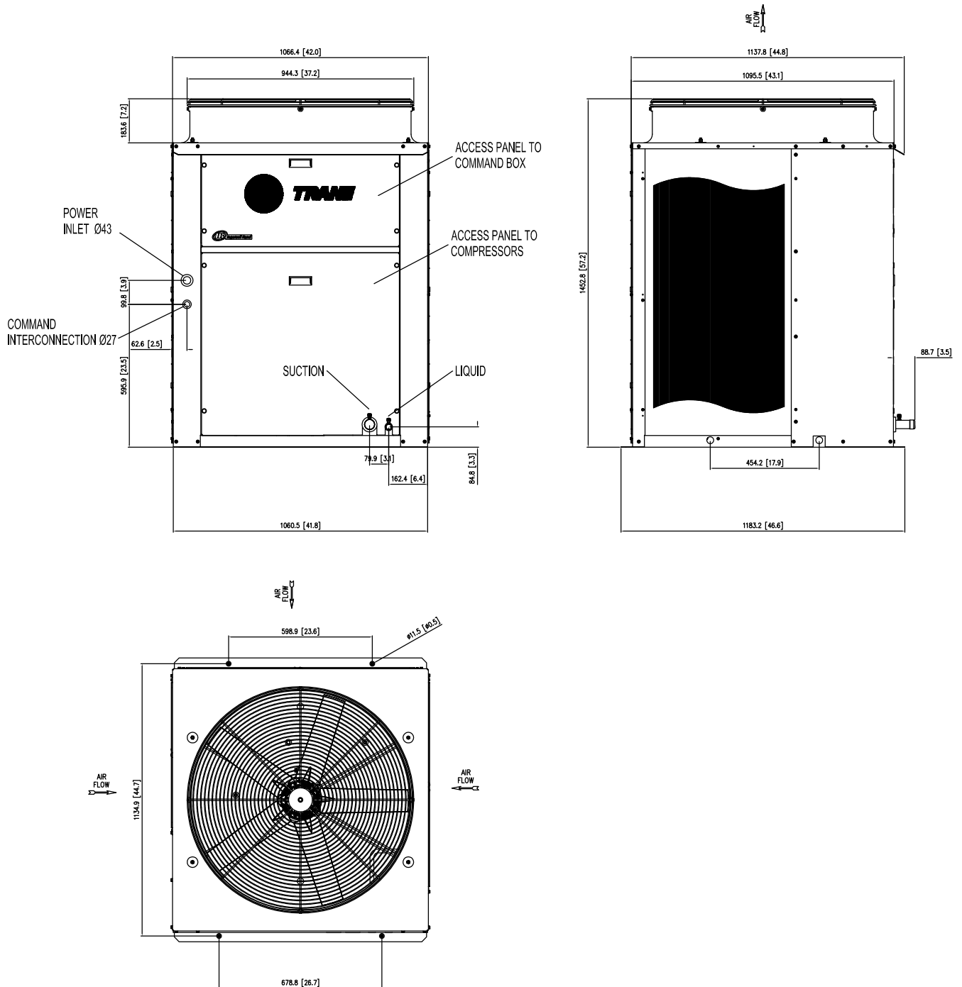
Fig. X-30 - Dimensions - Condensing Units TRAE 200 - 1 Circuit
