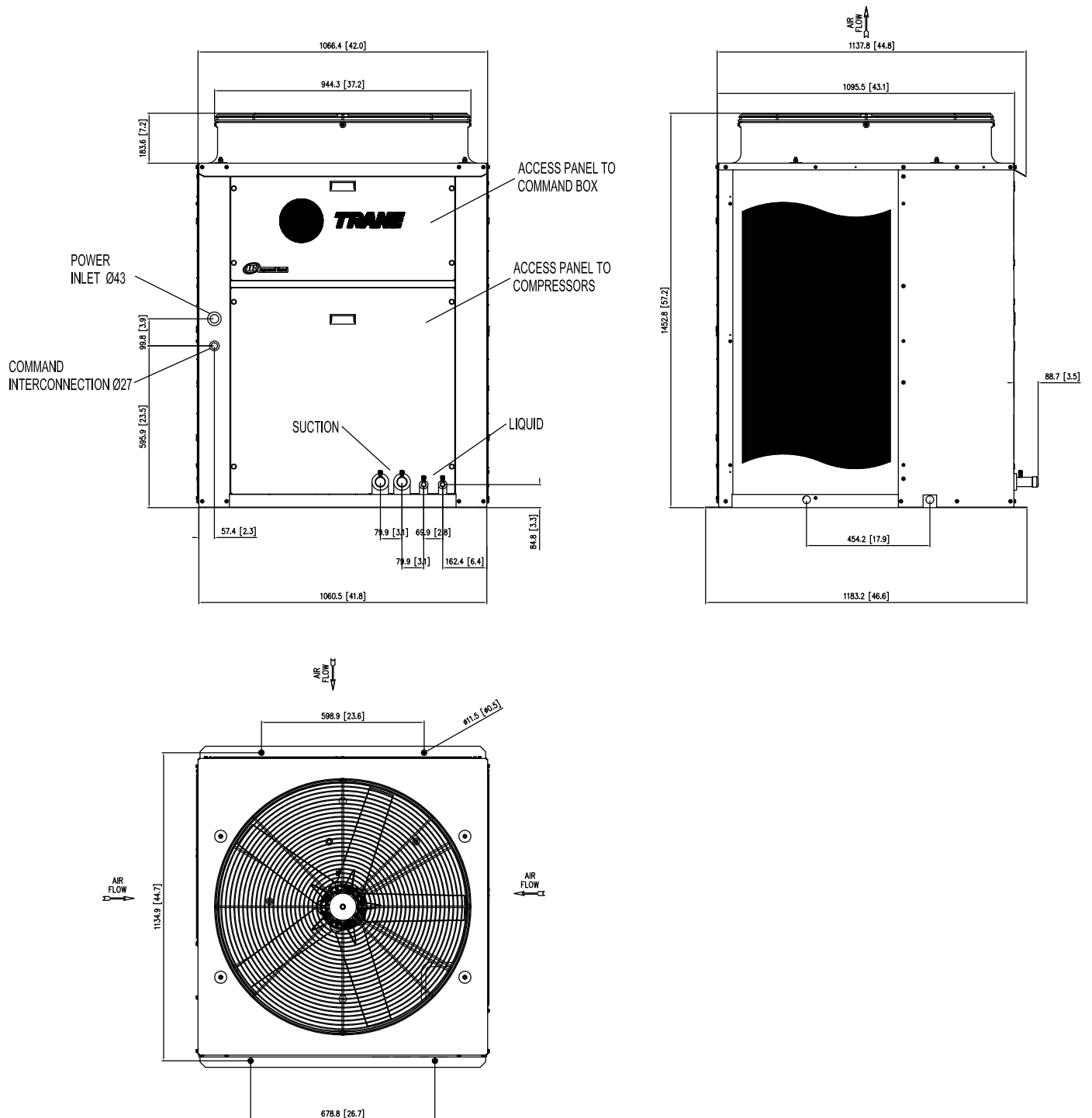
Fig. X-31 - Dimensions - Condensing Units TRAE 200 - 2 Circuits
