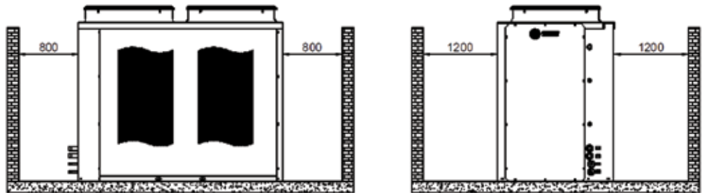
Fig. X 37 - Suggested clearances TRAE 200 to 250 - Vertical Discharge
