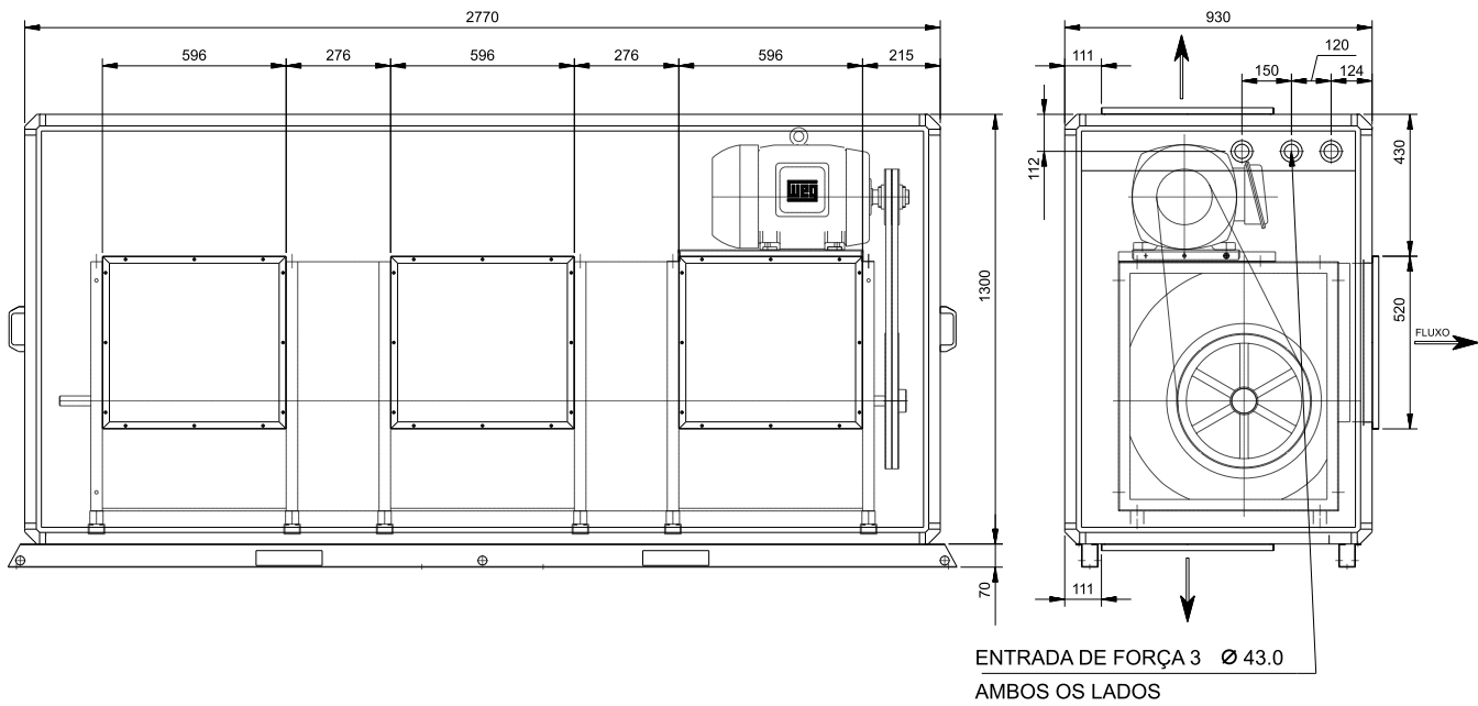
Fig. X-08 - Dimensions - Fan Modules 35/40/50 - Backward-Curved
