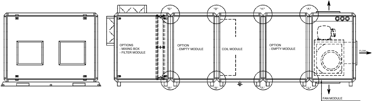
Fig. X-17 – Horizontal/vertical assembly 05 to 50 – DL (Only by design special requiring)
