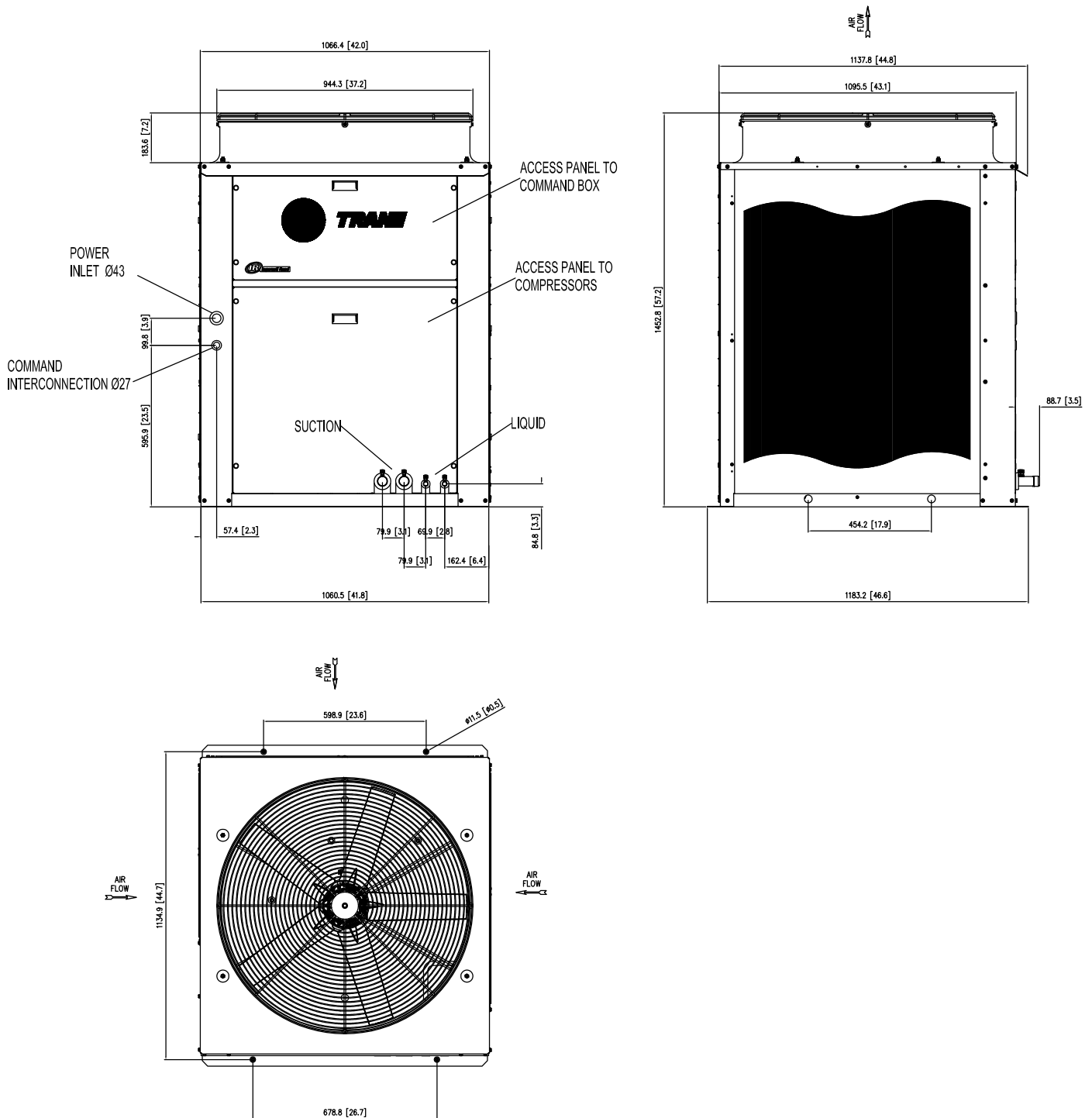
Fig. X-33 - Dimensions - Condensing Units TRAE 250 - 2 Circuits
