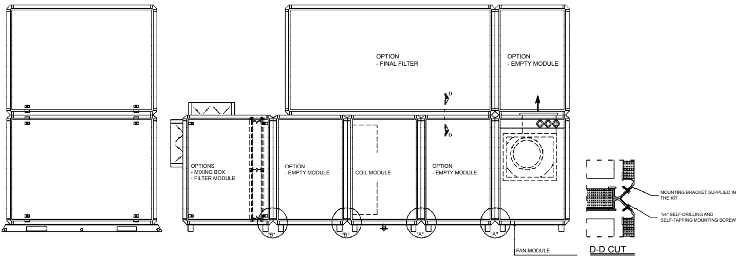
Fig. X-18 – Horizontal assembly with Final Filter
