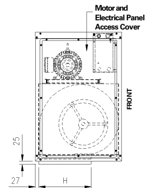
Fig. 18c - Downflow Discharge
