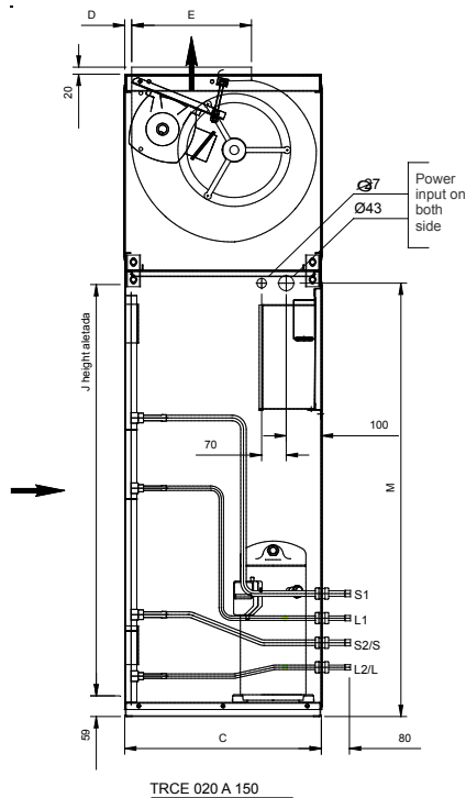
Fig. 41 - Connections - condensing unit TRCE
