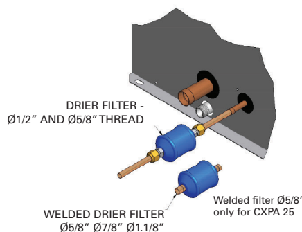
MOUNTING DIAGRAM DRIER FILTER
