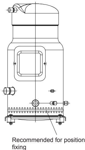
Fig.09 - Crankcase Heater
