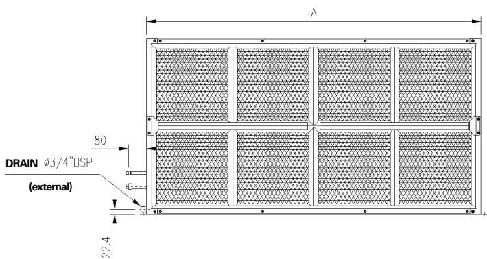
Fig. 13 - Dimensional Data - Coil Module - 050 to 100
