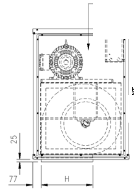
Fig. 21c - Downflow Discharge
