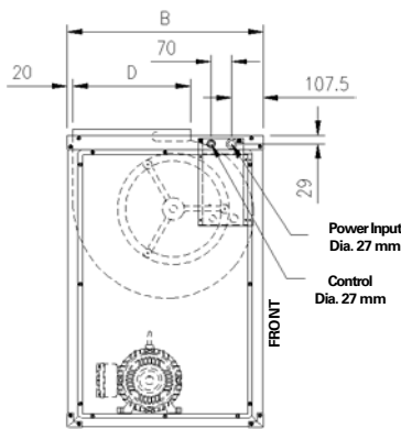
Fig. 18a - Vertical Discharge
