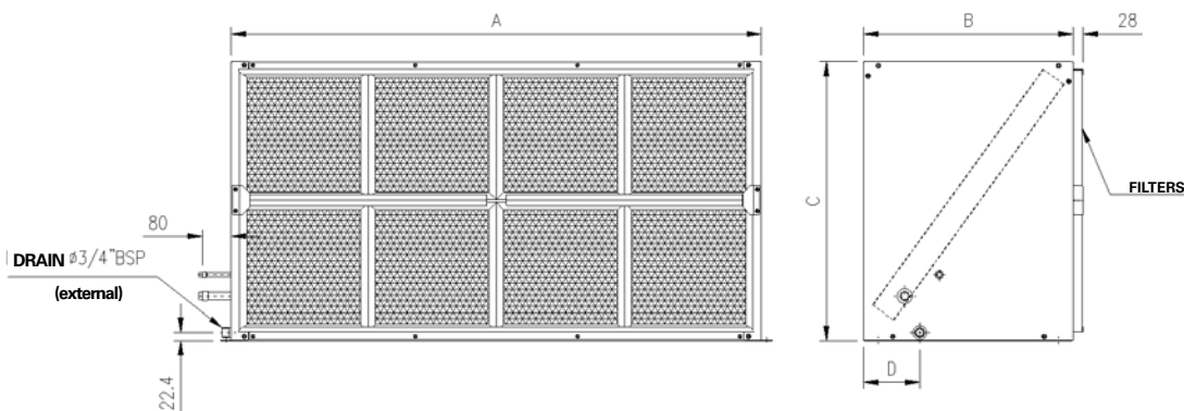
Fig. 19 - Dimensional Data - Coil Module - 200 to 300
