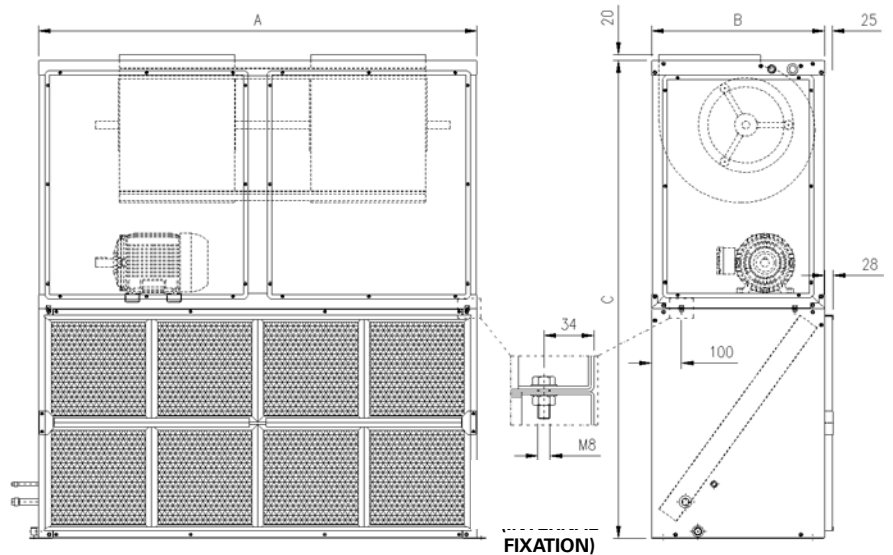
Fig. 27 - Fan and Coil Module Assembly - CXPA 050 to 500 - Vertical
