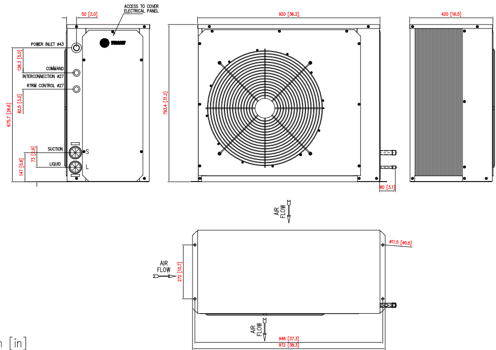
Fig. 32 - Dimensions - Condensing Units TRAE 075
