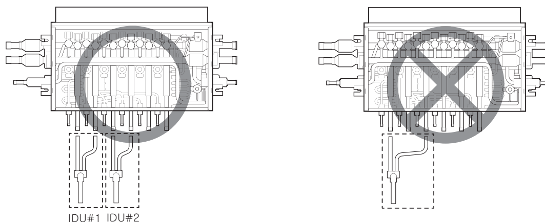
Figure 3. Connect Y-joint in series to MCU
