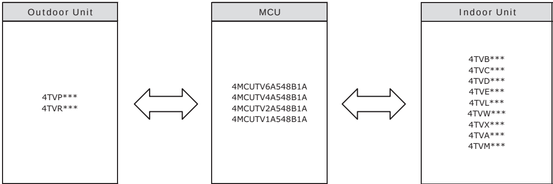
Figure 1. MCU compatibility with outdoor and indoor units
