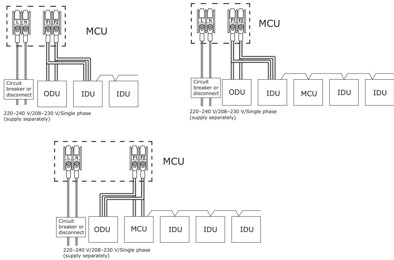
Figure 4. MCU wiring terminal connections: three examples
