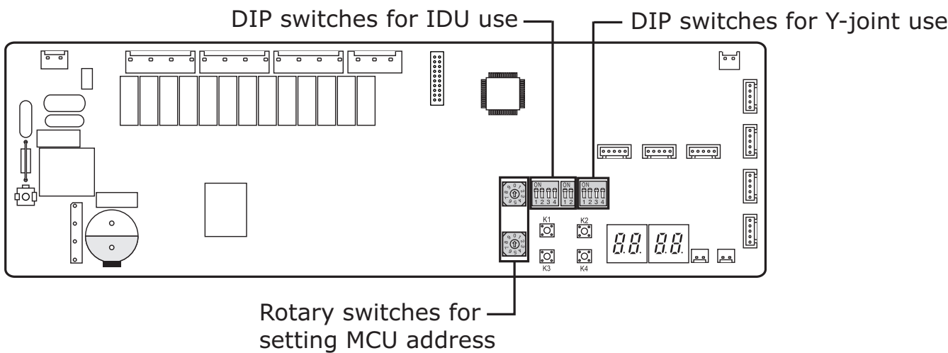
Figure 5. MCU control board
