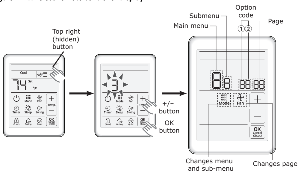
Figure 7. Wireless remote controller display
