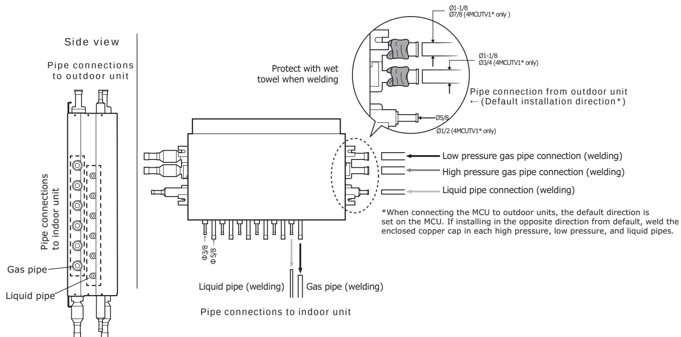
Figure 2. Connecting refrigerant piping to the MCU
