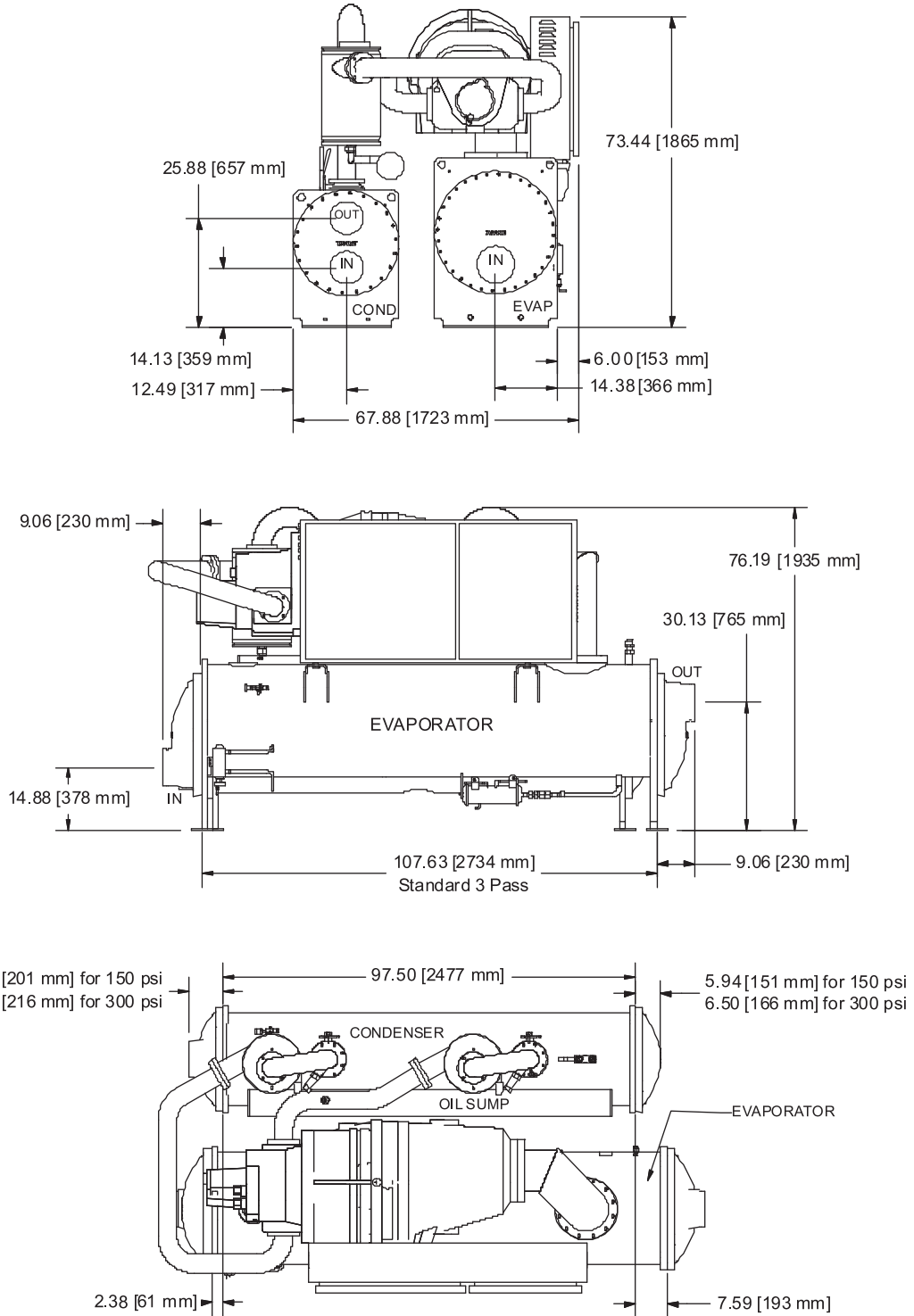
Figure 3. CDE, DDE, EDE configurations
