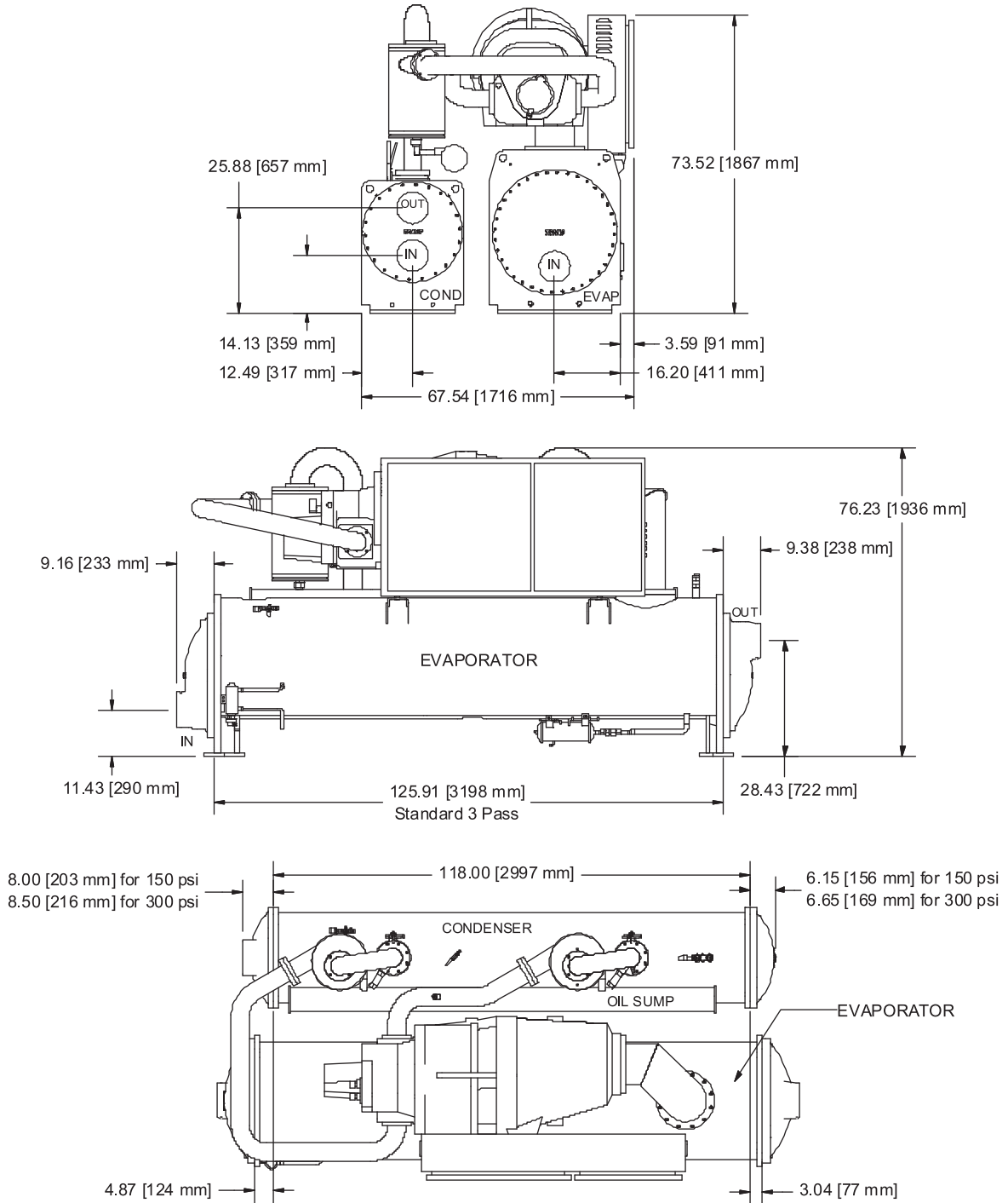
Figure 5. CFF, DFF, EFF configurations
