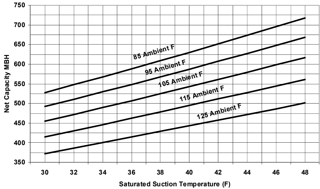
Figure 16. 60 Ton condensing unit performance — RAUJ-C60 (50 HZ)
