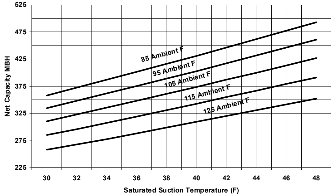
Figure 14. 40 Ton condensing unit performance – RAUJ-C40 (50 HZ)
