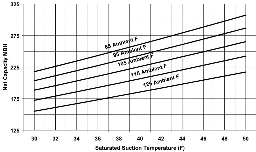
Figure 3. 25 Ton condensing unit performance — RAUJ-C25 (60 HZ)
