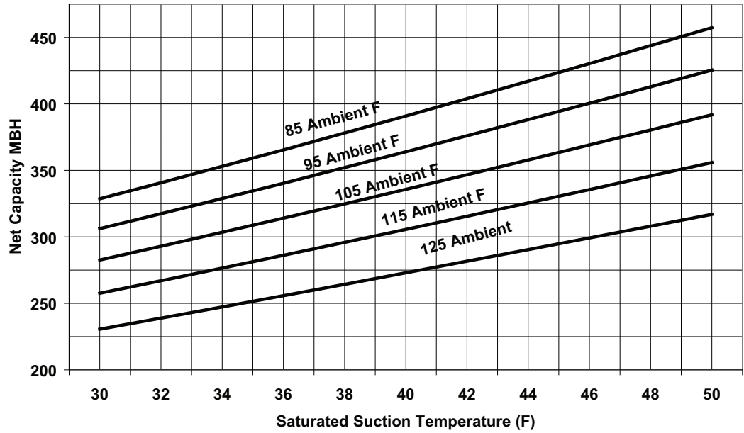
Figure 4. 30 Ton condensing unit performance — RAUJ-C30 (60 HZ)
