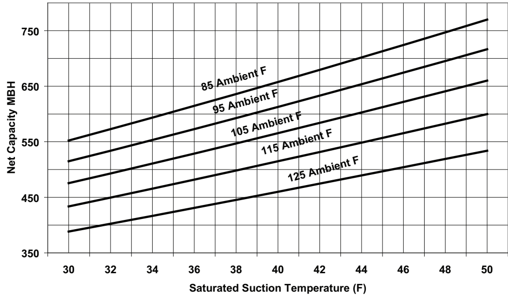
Figure 6. 50 Ton condensing unit performance — RAUJ-C50 (60 HZ)
