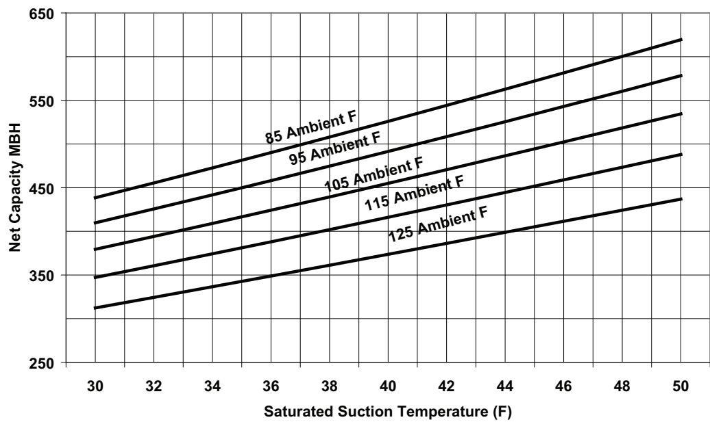
Figure 5. 40 Ton condensing unit performance — RAUJ-C40 (60 HZ)
