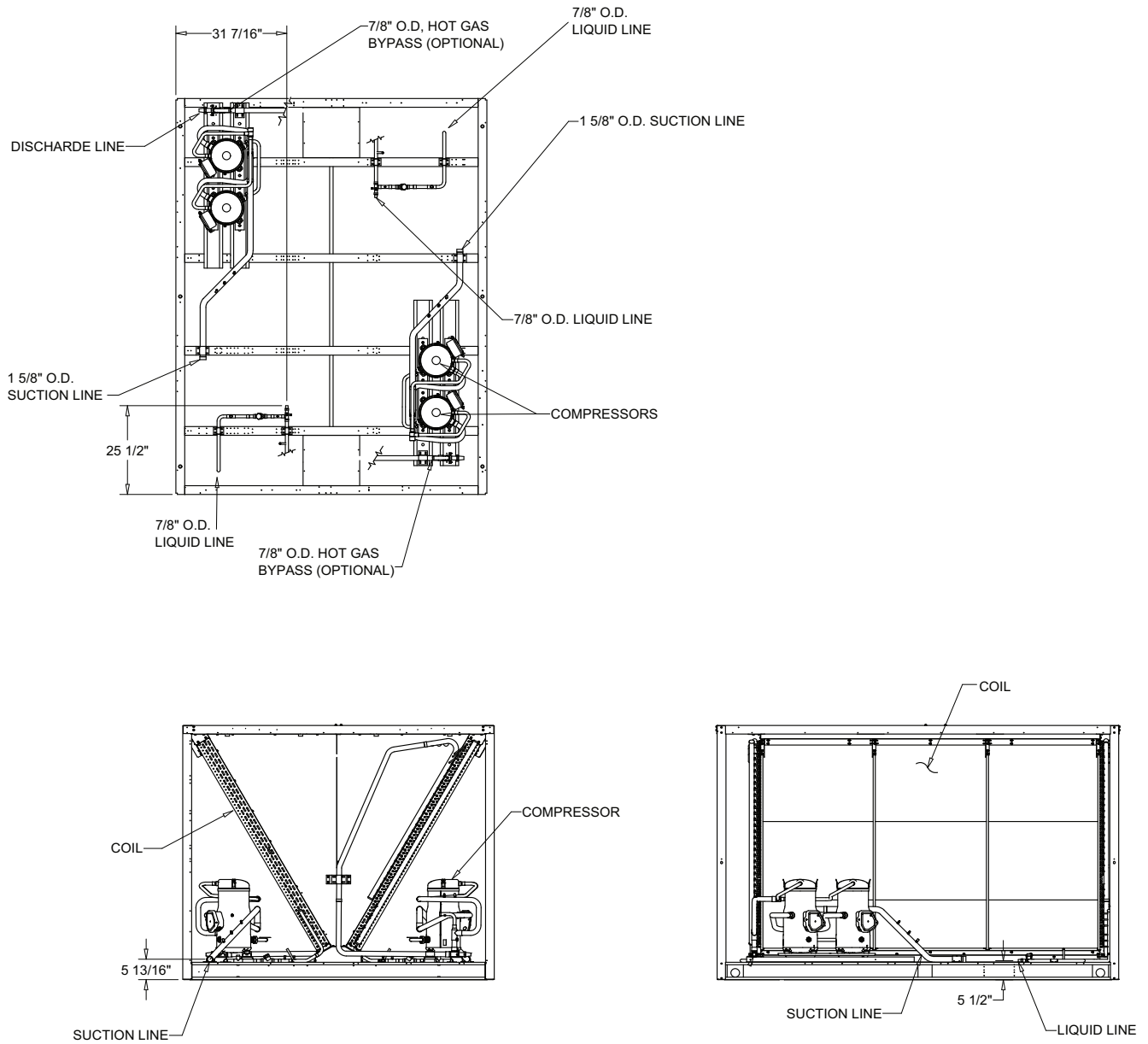
Figure 32. 60-Ton air-cooled condensing unit (connections)
