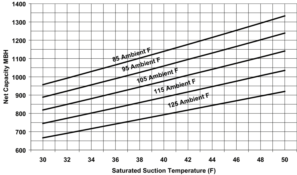
Figure 8. 80 Ton condensing unit performance — RAUJ-C80 (60 HZ)
