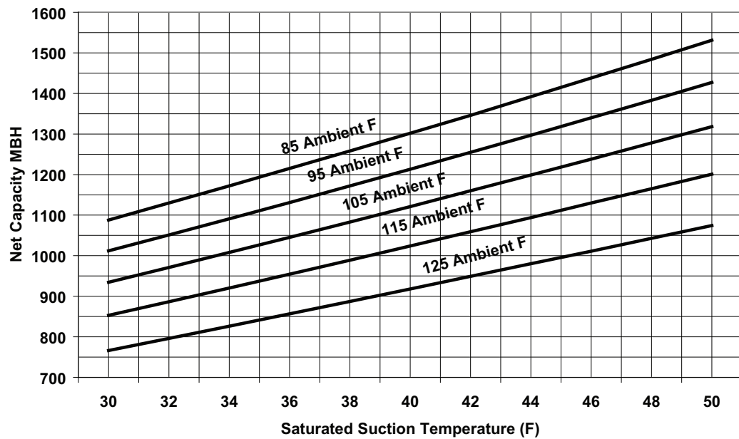
Figure 9. 100 Ton condensing unit performance — RAUJ-D10 (60 HZ)
