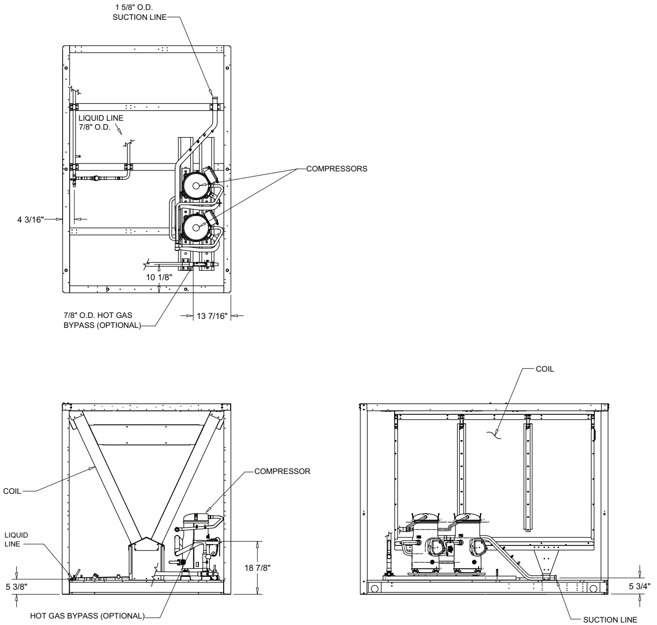
Figure 26. 25- and 30-Ton air-cooled condensing unit (connections)
