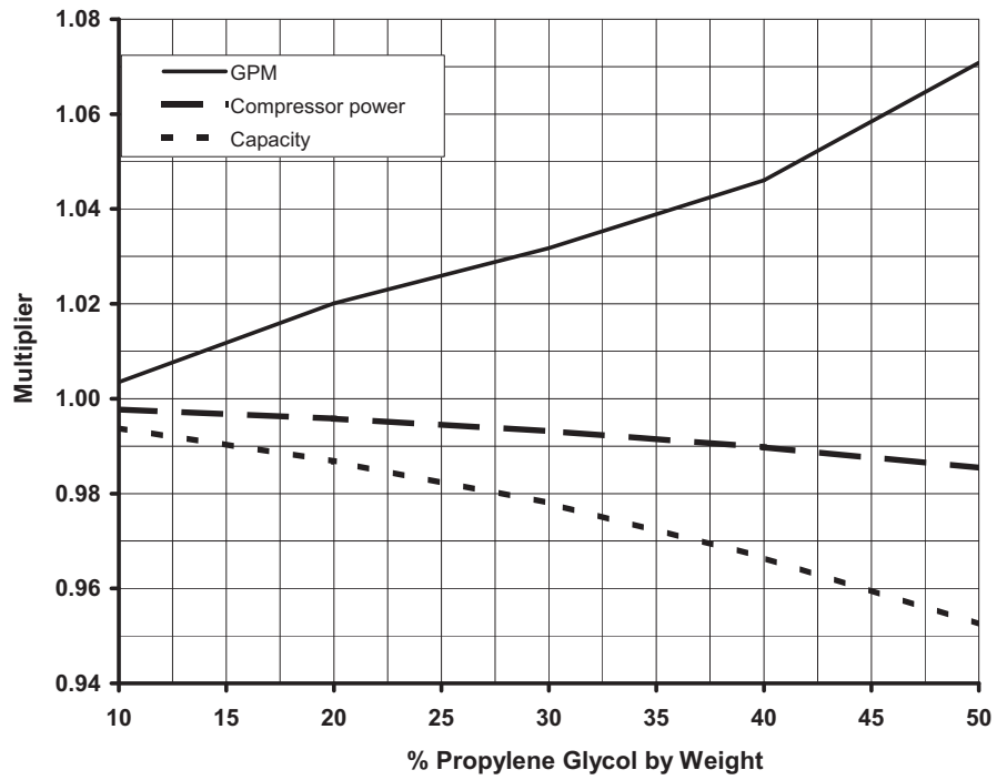
Figure 22. Remote EVP Propylene Glycol GPM, Capacity, and Compressor Power Adjustment
