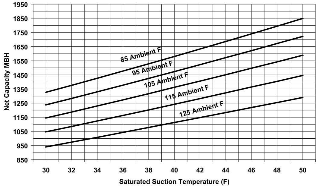
Figure 10. 120 Ton condensing unit performance – RAUJ-D12 (60 HZ)
