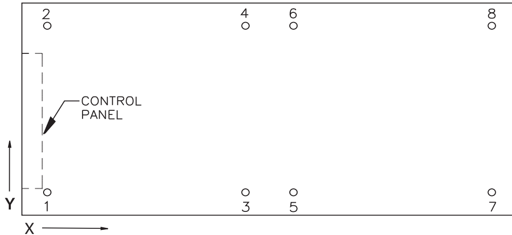
Figure 3. 80- to 120-Ton air-cooled condensing units
