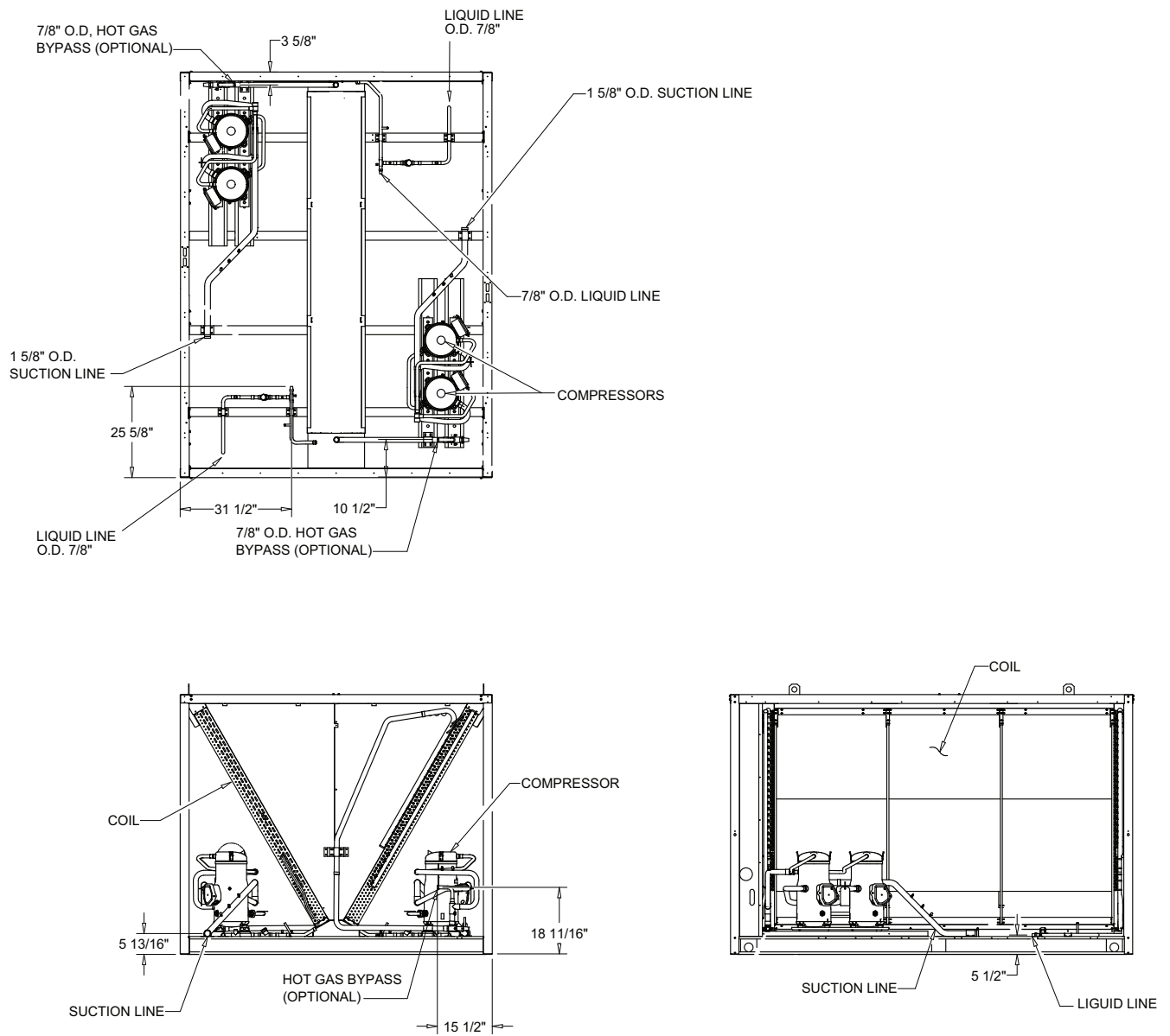
Figure 30. 50-Ton air-cooled condensing unit (connections)
