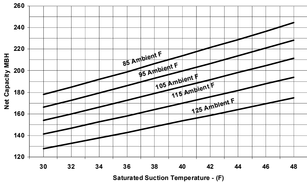
Figure 11. 20 Ton condensing unit performance – RAUJ-C20 (50 HZ)
