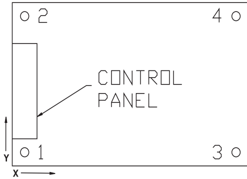
Figure 1. 20- to 30-Ton air-cooled condensing units
