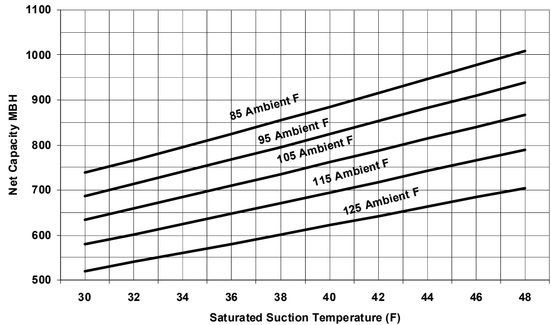
Figure 17. 80 Ton condensing unit performance — RAUJ-C80 (50 HZ)
