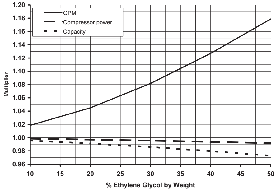
Figure 21. Remote EVP Ethylene Glycol GPM, Capacity, and Compressor Power Adjustment
