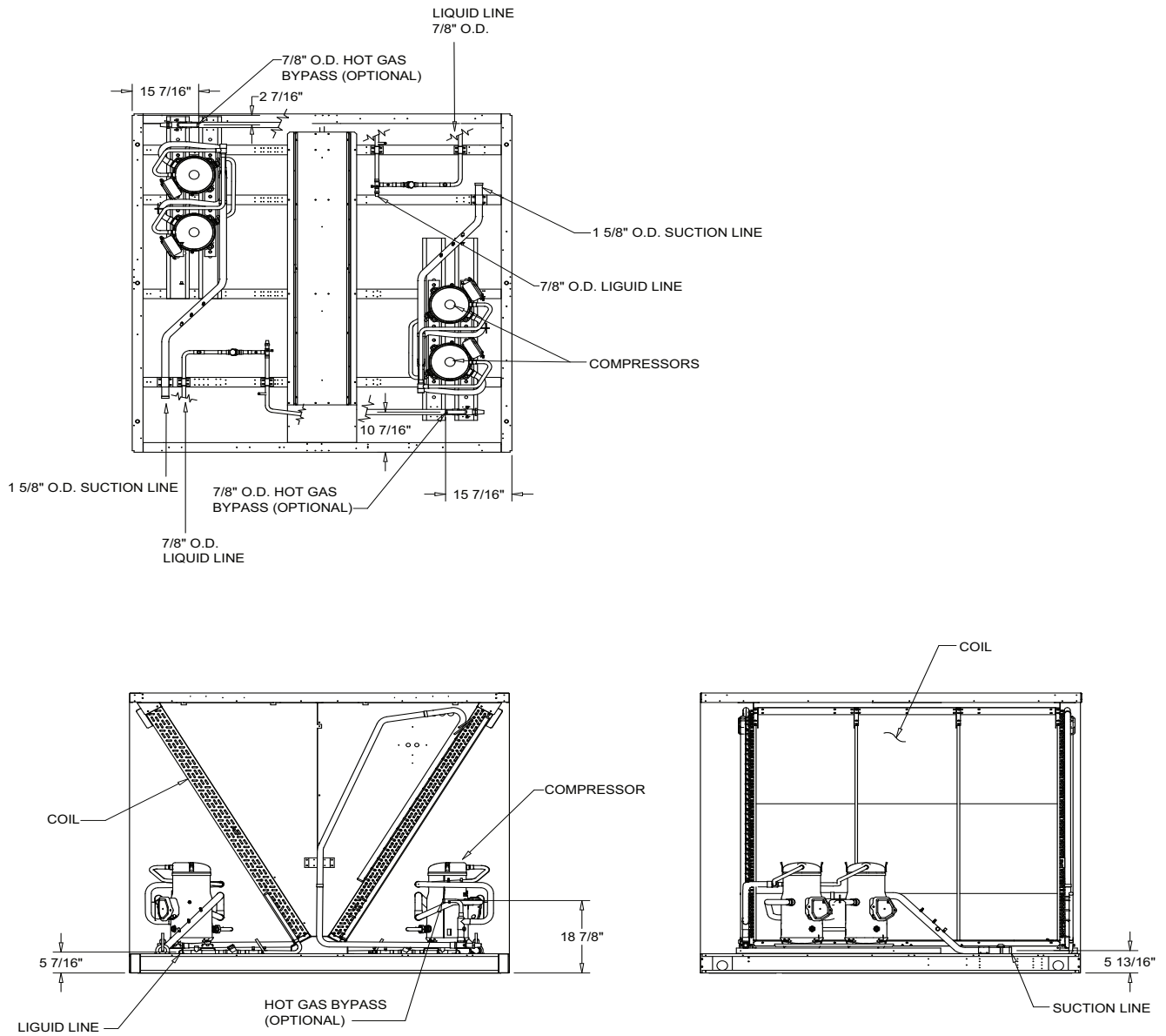
Figure 28. 40-Ton air-cooled condensing unit (connections)
