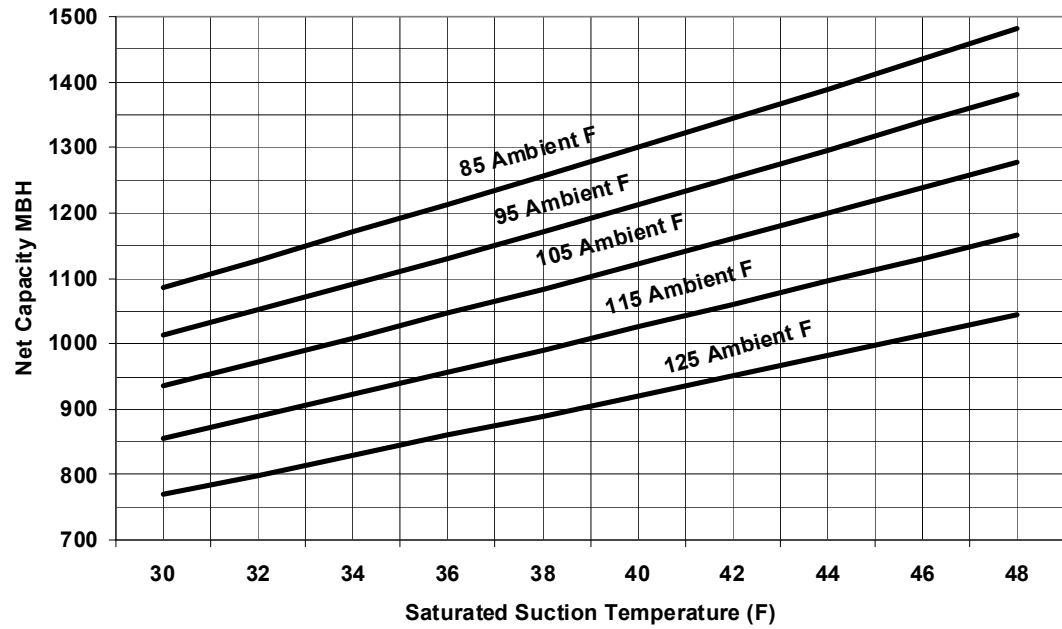
Figure 19. 120 Ton condensing unit performance – RAUJ-D12 (50 HZ)
