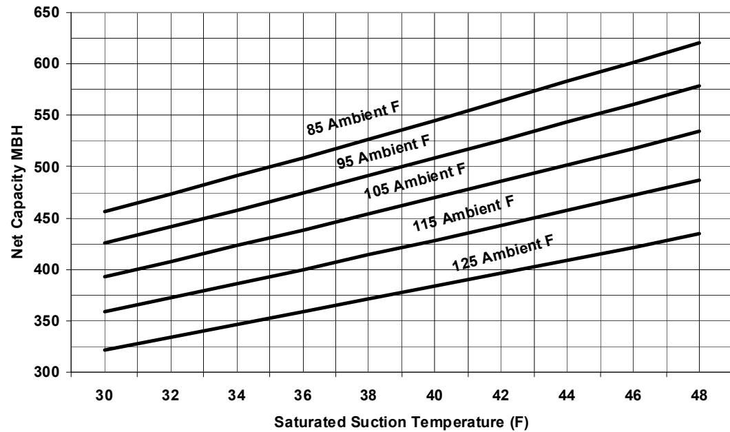
Figure 15. 50 Ton condensing unit performance – RAUJ-C50 (50 HZ)
