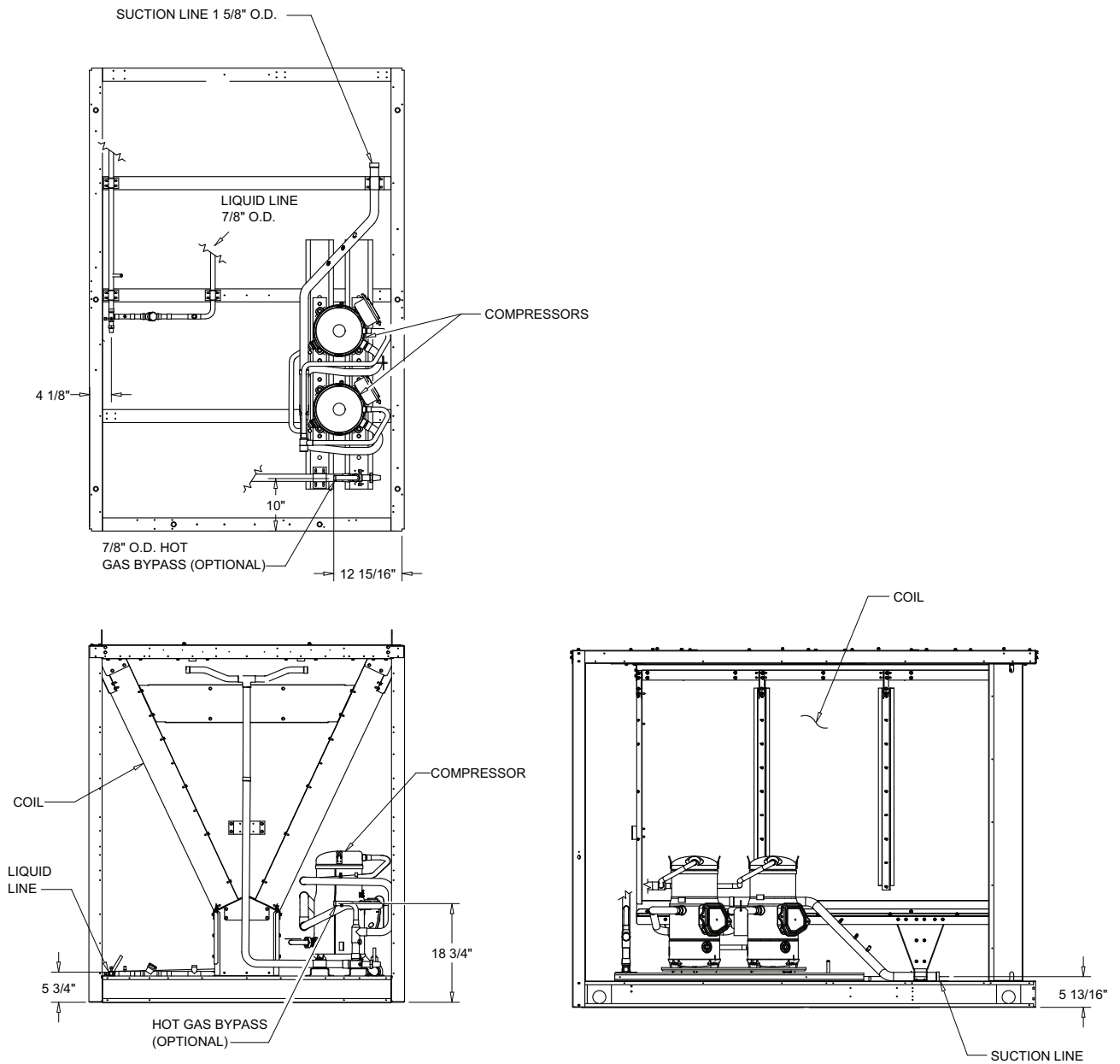
Figure 24. 20-Ton air-cooled condensing unit (connections)
