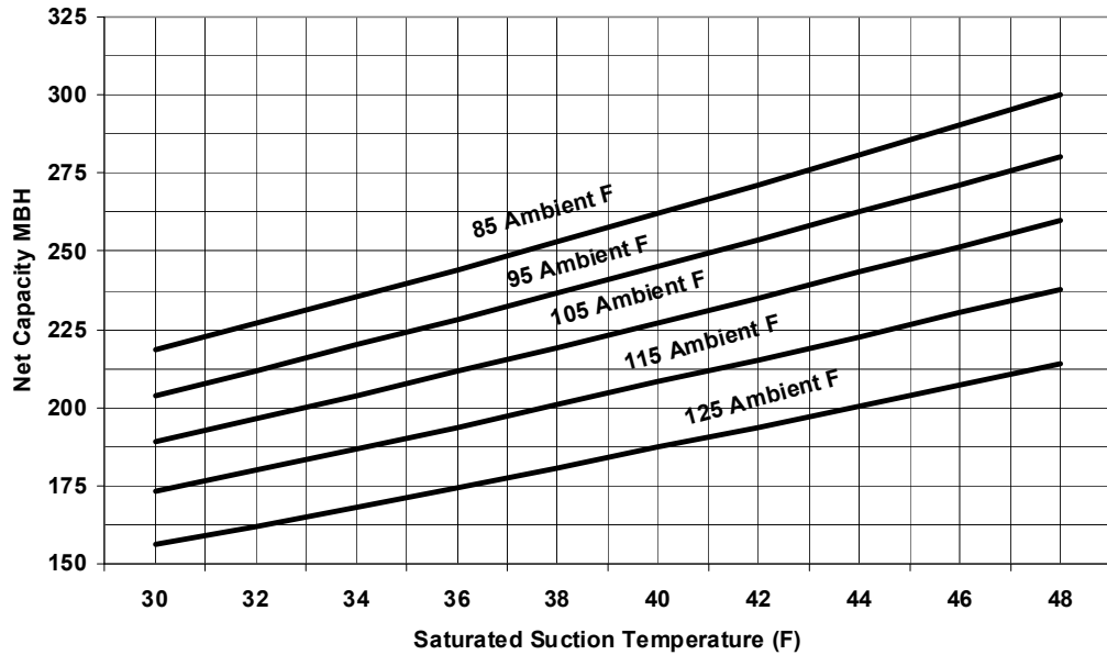
Figure 12. 25 Ton condensing unit performance — RAUJ-C25 (50 HZ)
