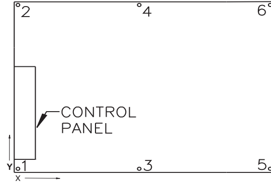
Figure 2. 40- to 60-Ton air-cooled condensing units
