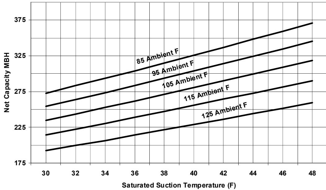
Figure 13. 30 Ton condensing unit performance — RAUJ-C30 (50 HZ)
