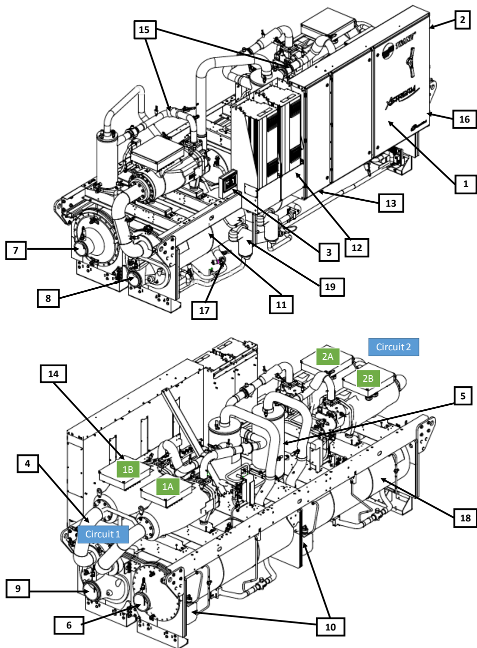
Figure 1 – Component Location for Typical RTWF Unit
