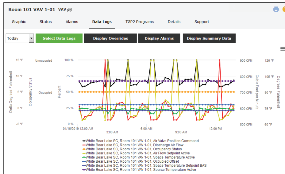
Figure 8. Data Logs Tab
