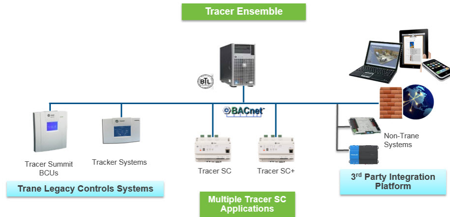
Figure 1. Tracer Ensemble Architecture
