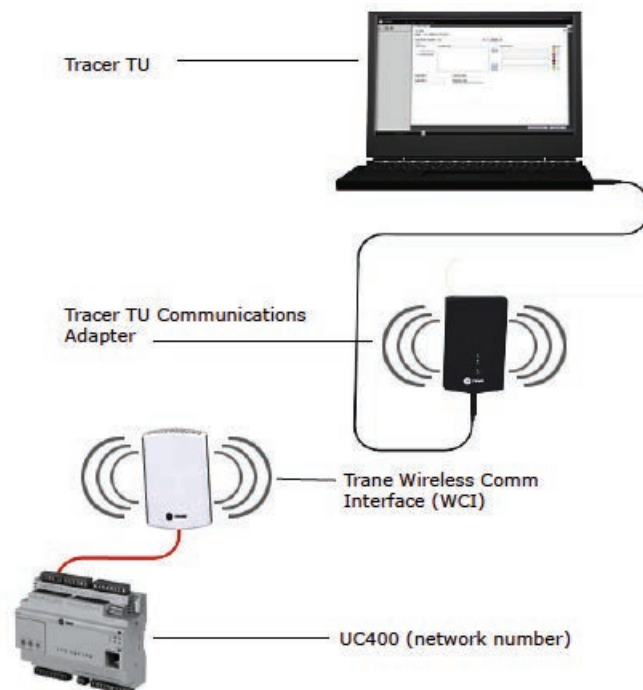
Figure 31. Wireless access through the Tracer TU Communication Adapter
