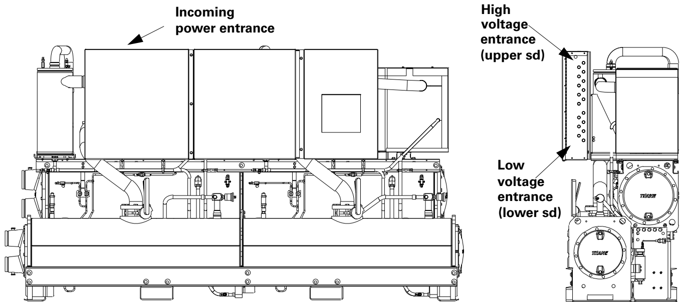
Figure 44. Power entrance
