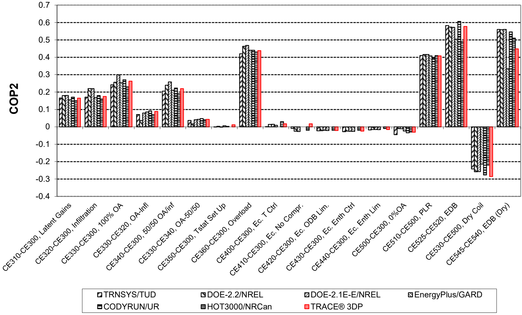
Figure B16.5.2-22. HVAC BESTEST: CE300 - CE545 Annual Mean COP2 Sensitivities
