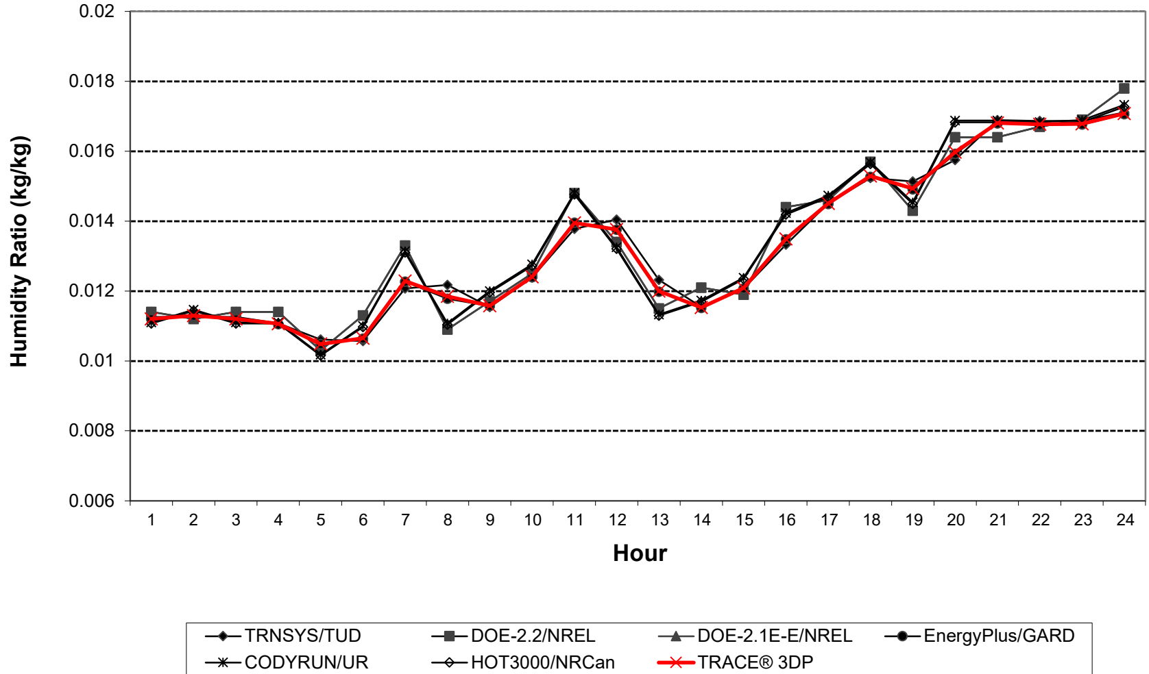
Figure B16.5.2-52. HVAC BESTEST: CE300 June 28 Hourly OHR
